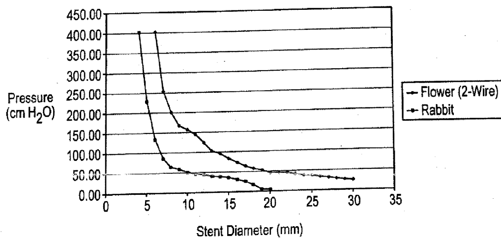
Diameter vs. Pressure
