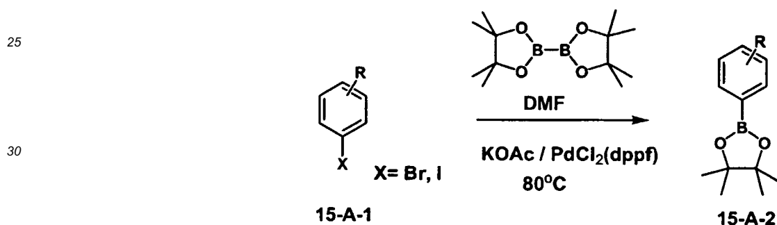
Scheme 15-A: General Procedure for Synthesis of Boronate Esters from Aryl Halides
