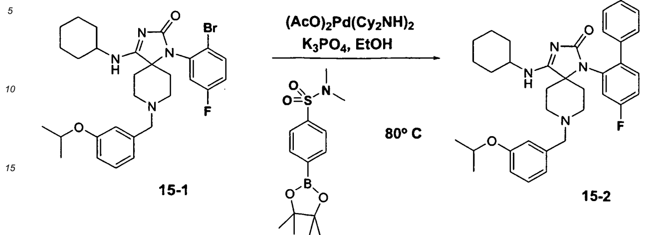
Scheme 15-A: General Procedure for Synthesis of Boronate Esters from Aryl Halides
