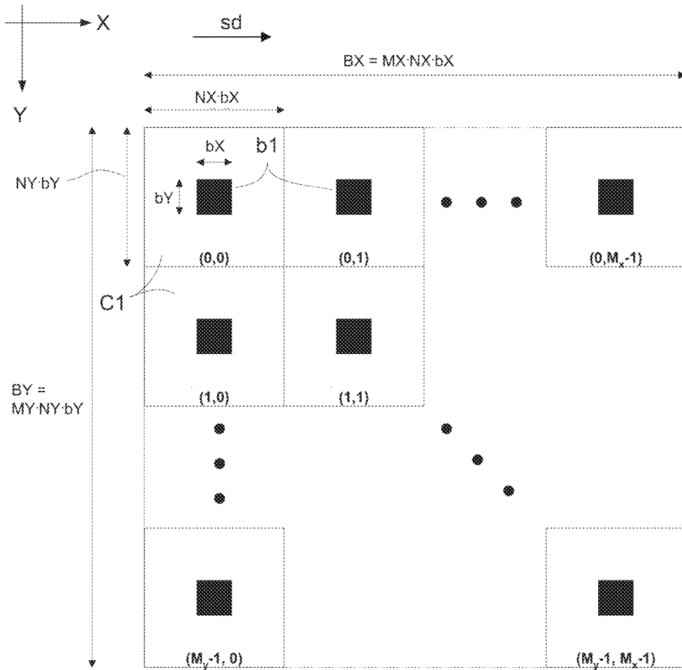
Fig. 4 (prior art)
