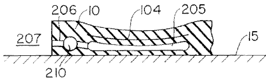
FIG. 10H PRIOR ART
