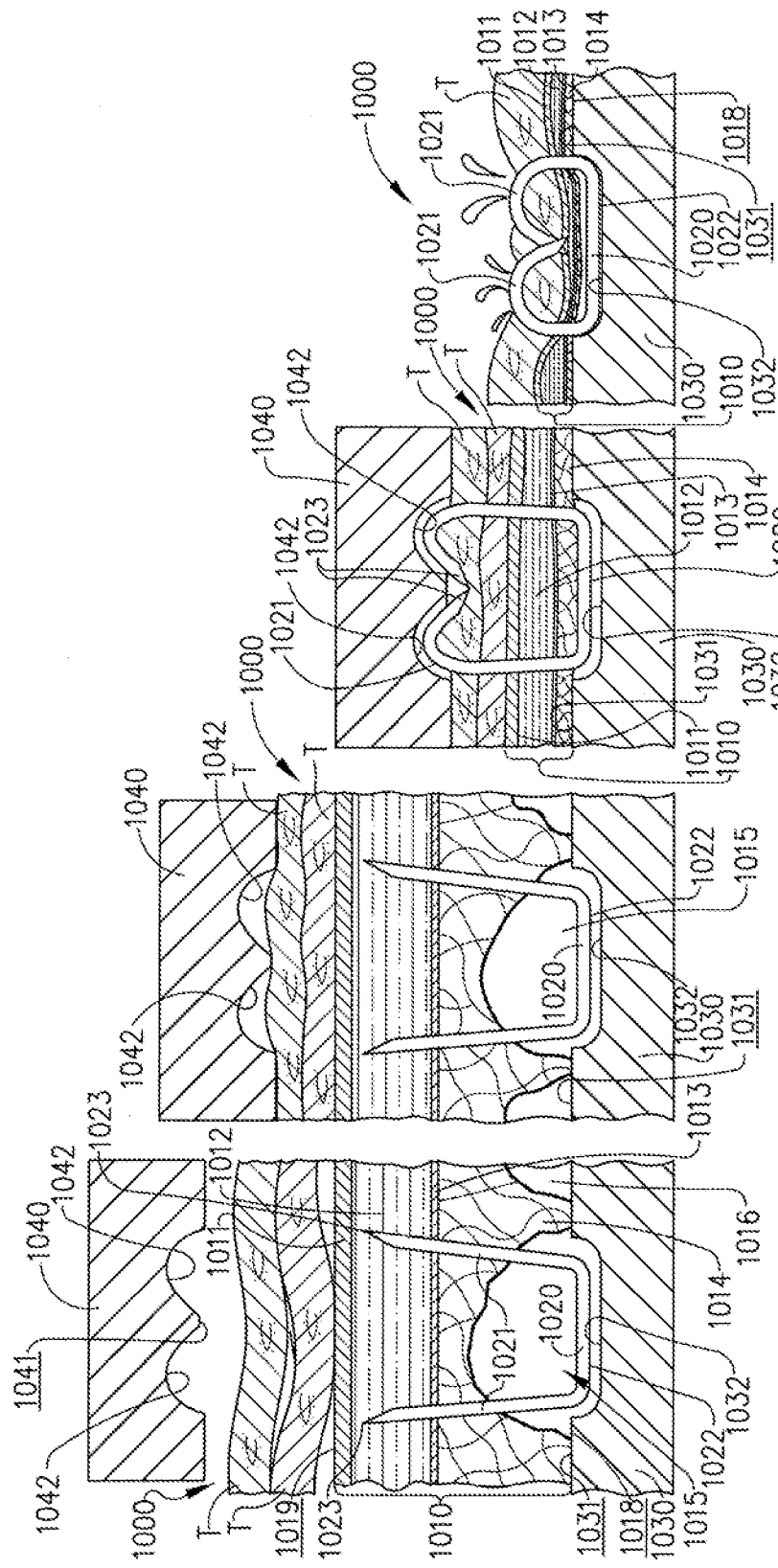
FIG. 18A JAW OPEN FIG. 18B JAW CLOSED FIG. 18C STAPLES FORMING FIG. 18D COMPLETELY FORMED
