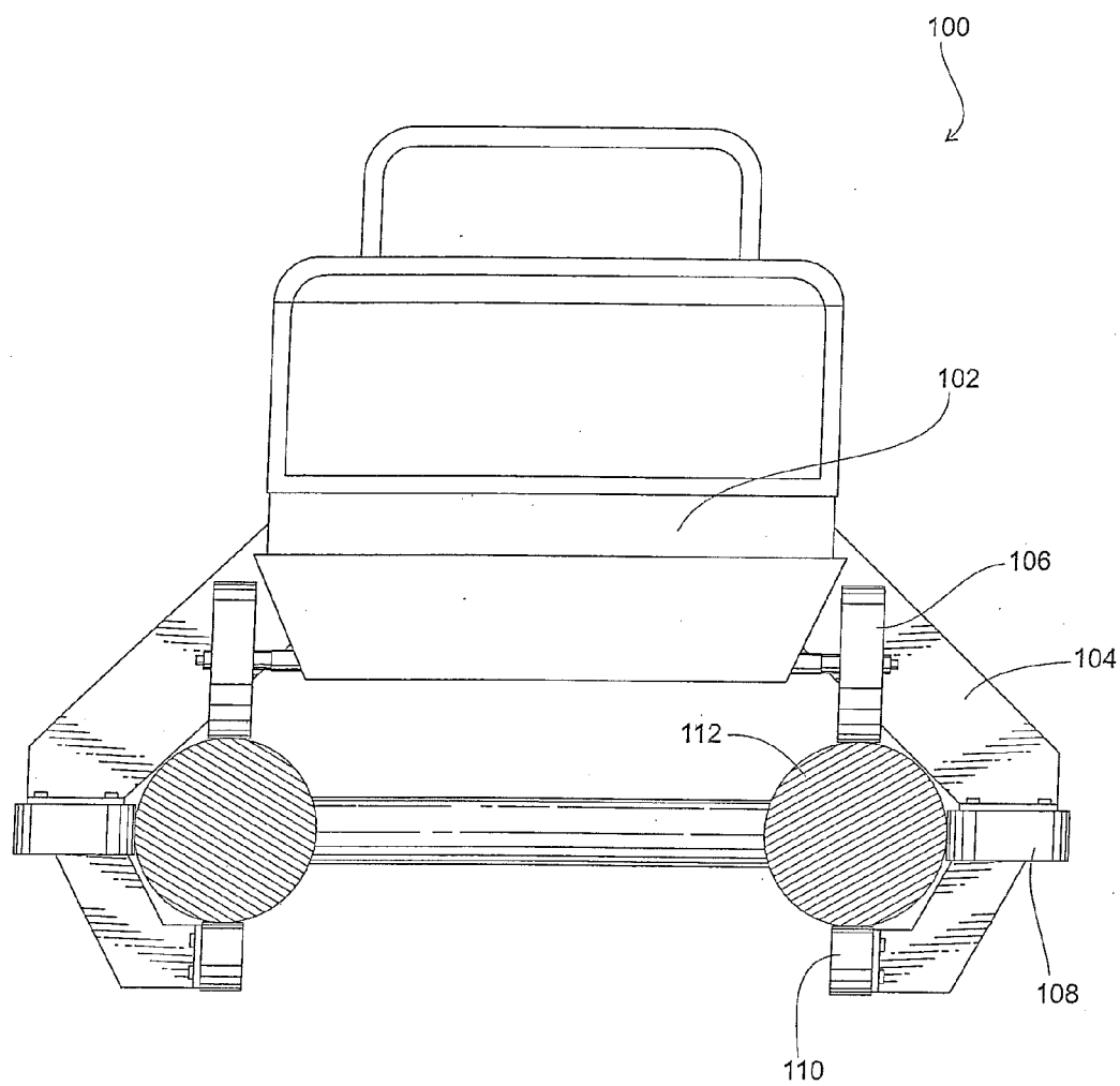
Fig. 1 PRIOR ART
