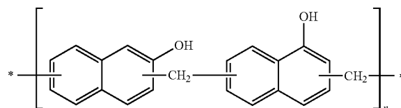
[Chemical Formula 2a]
