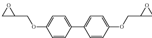
[Chemical Formula C]
