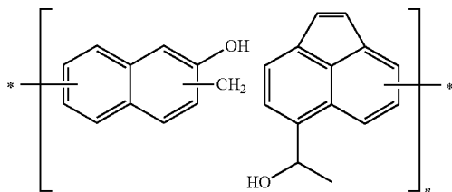
[Chemical Formula 4a]
