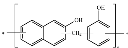
[Chemical Formula 3a]
