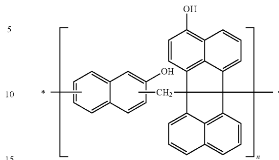
[Chemical Formula 5a]
