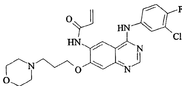
Compound 1
