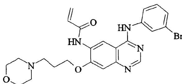
Example 21
