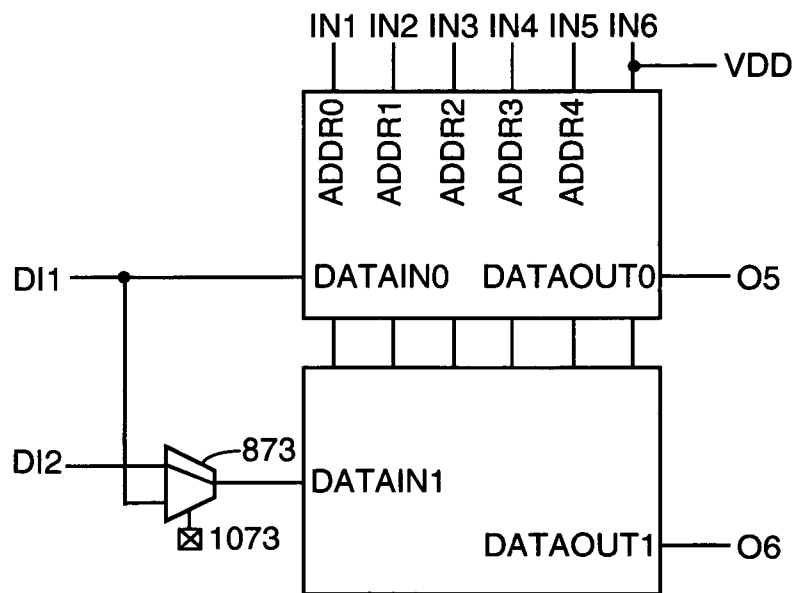
FIG. 11 (32x2 RAM)
