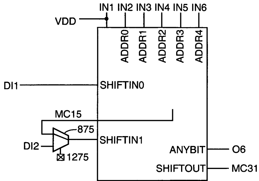
FIG. 12 (32x1 SRL)
