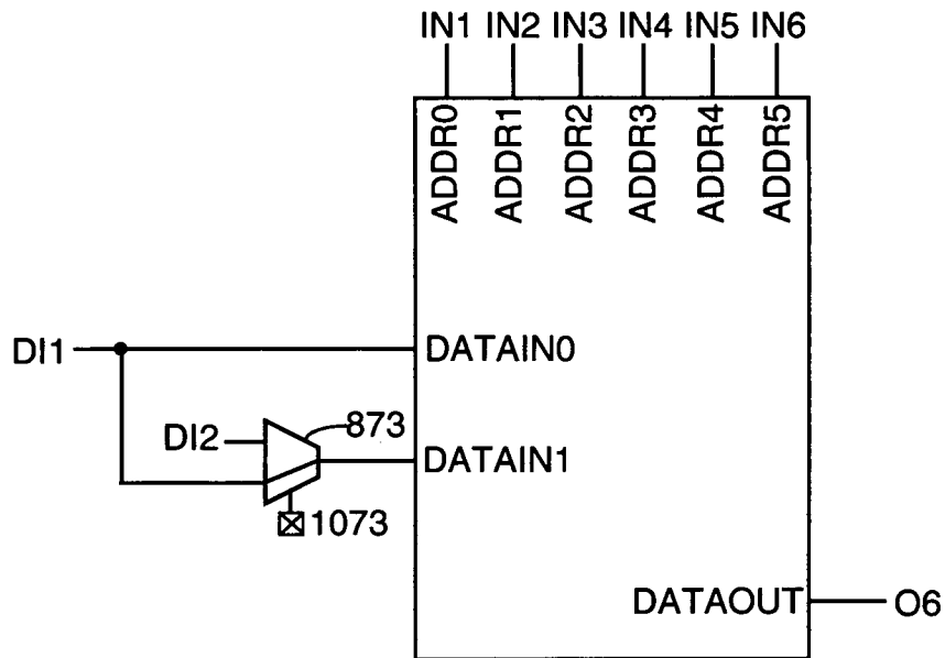
FIG. 10 (64x1 RAM)
