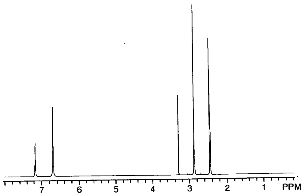
Proton NMR of Dimethylbiguanide
