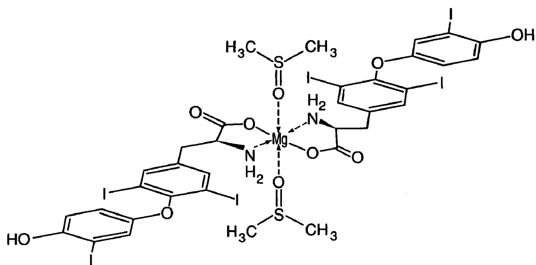
Bis(triiodothyroninato)-bis(dimethylsulfoxide)magnesium
