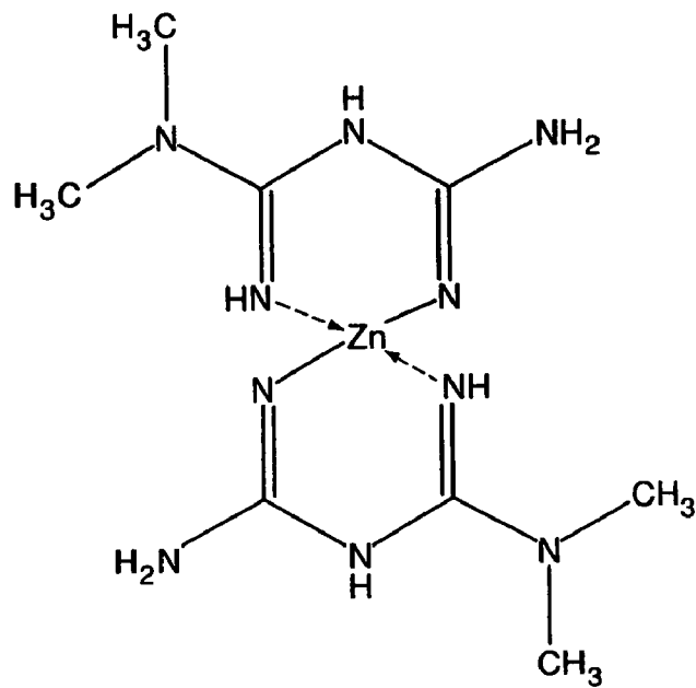
Dimethylbiguanide-zinc complex
