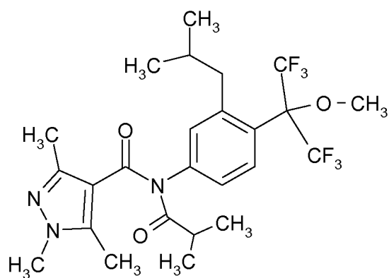
j) Afidopyropen (or also known as coprapidpen or under Code No. ME 5343)
