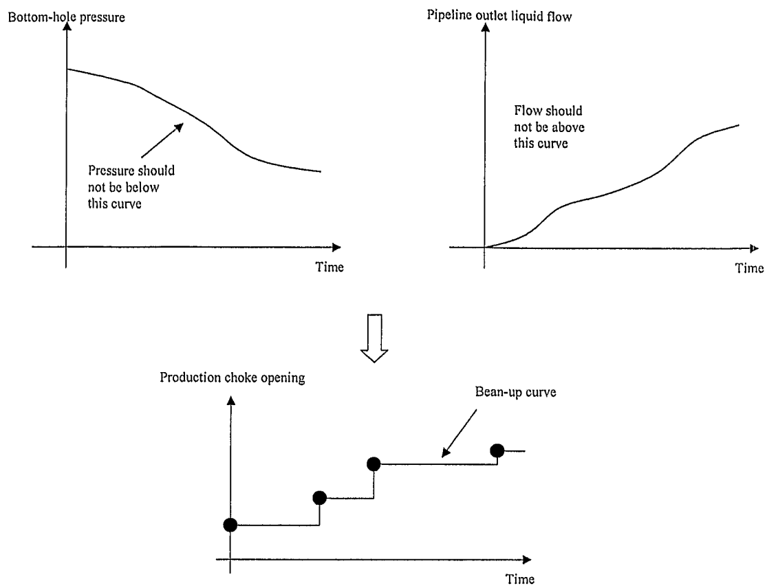
Fig. 19 (Prior Art)
