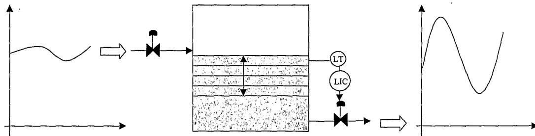
Fig. 18 (Prior Art)
