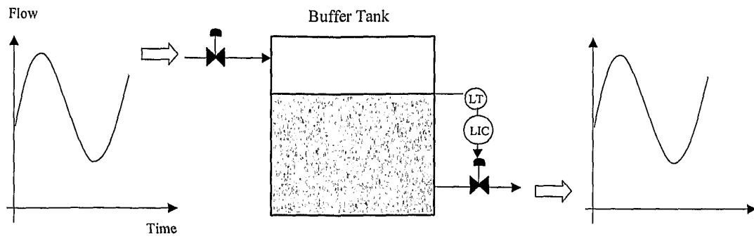
Fig. 17 (Prior Art)
