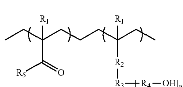
[Chemical Formula 3]
