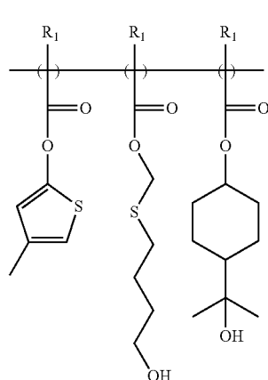
[Chemical Formula 7]
