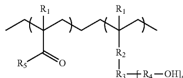
[Chemical Formula 7]
