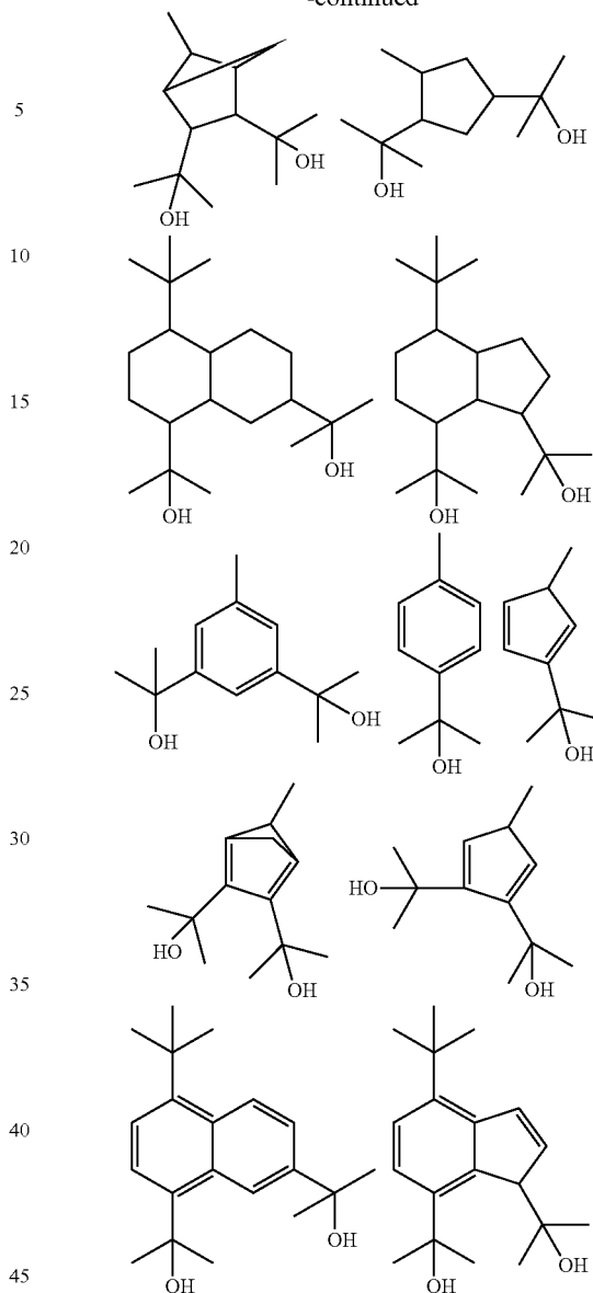
[Chemical Formula 1]
