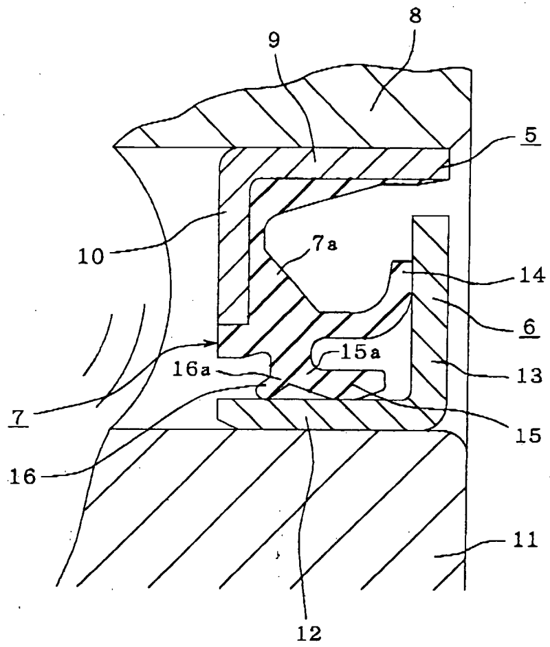
Fig. 3 PRIOR ART
