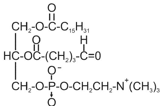
POVPC 1-Hexadecanoyl-2-(5'-oxopentanoyl)-sn-3-glycerophosphocholine
