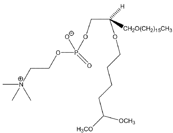
Compound IIa
