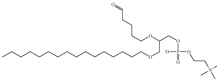
ALLE 1-hexadecyl-2-(5'-oxo-pentanyl)-sn-glycero-3-phosphocholine
