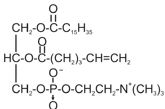
1-Hexadecanoyl-2-(5'-hexenoyl)-sn-3-glycerophosphocholine
