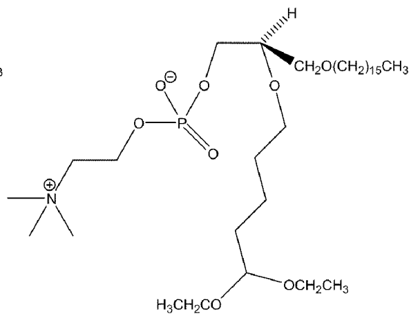
Compound IIb
