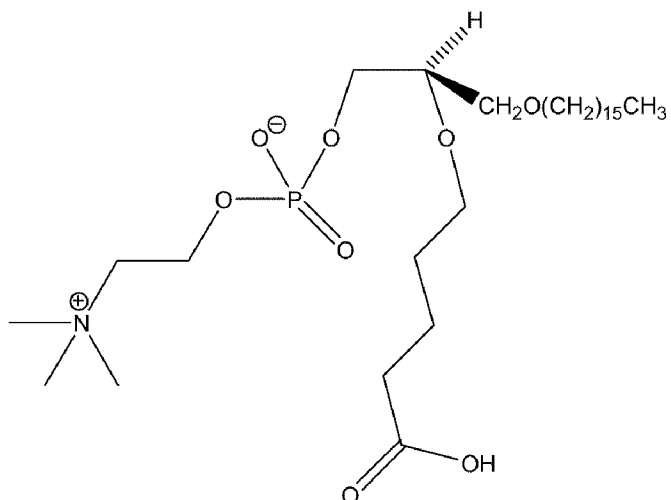
Compound I
