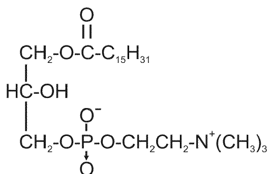
1-Hexadecanoyl-sn-3-glycerophosphocholine
