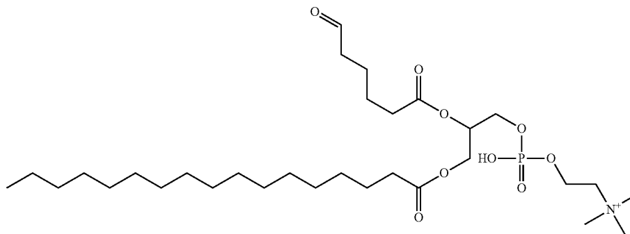
POVPC 1-hexadecanoyl-2-(5'-oxo-pentanoyl)-sn-3-phosphocholine
