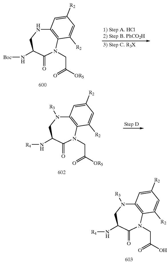
(3S)-2-Oxo-3-benzoylamino-5-(3-phenylpropionyl)-2,3,4,5-tetrahydro-1H-1,5-benzodiazepine-1-acetic Acid Methyl Ester (602a)
