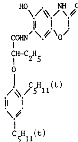
Coupler (4)
