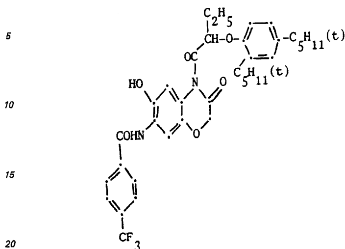
Coupler (5)
