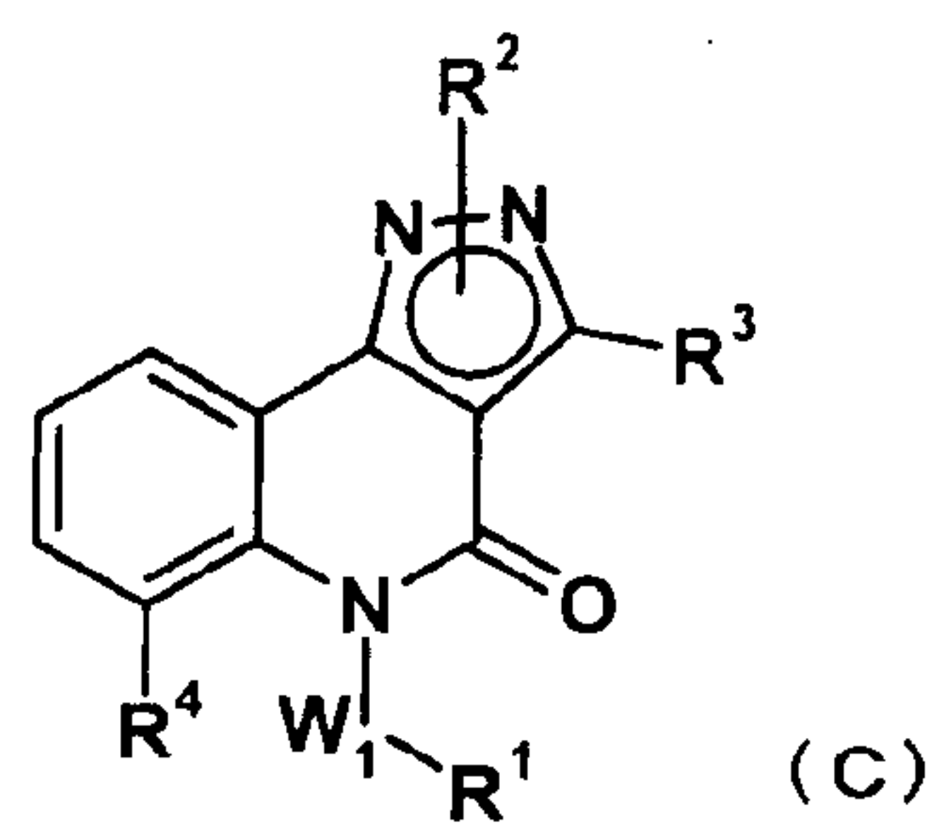
[Chem. 4]
