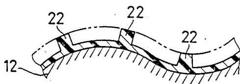
FIG. 15 PRIOR ART
