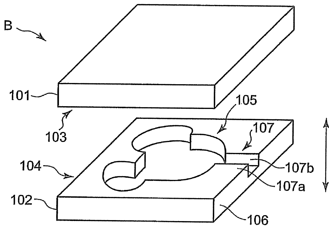
FIG. 13 Prior Art
