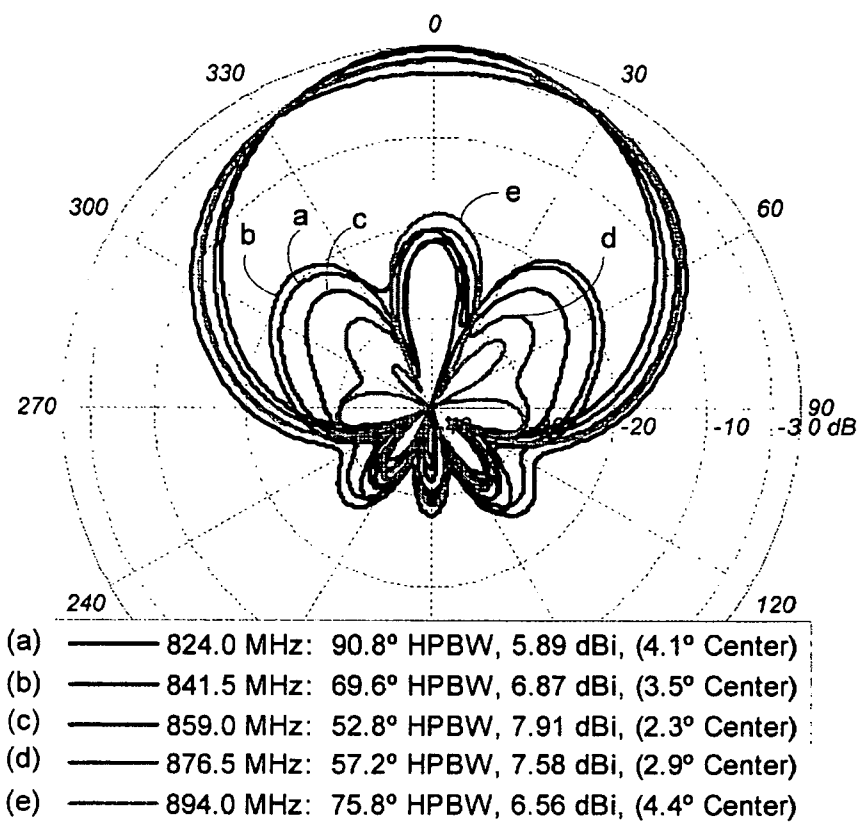
Fig. 11 - Prior Art
