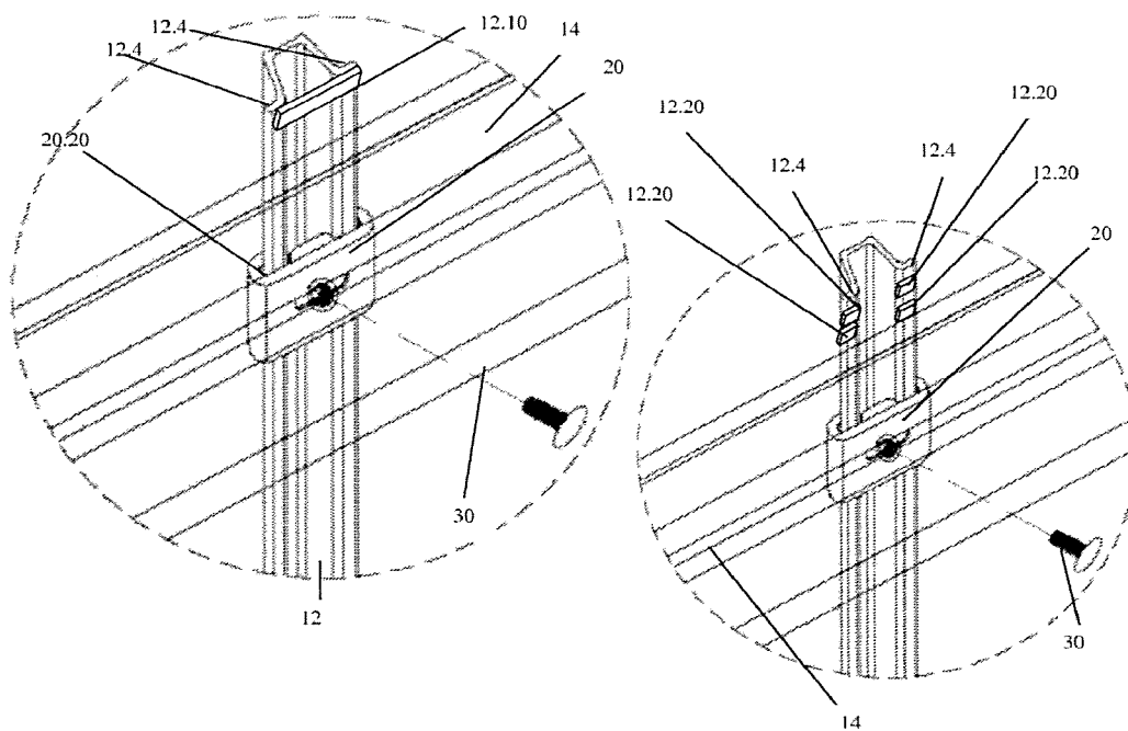
FIGURE 7 – PRIOR ART
