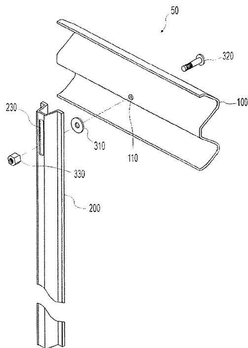
FIGURE 4 – PRIOR ART
