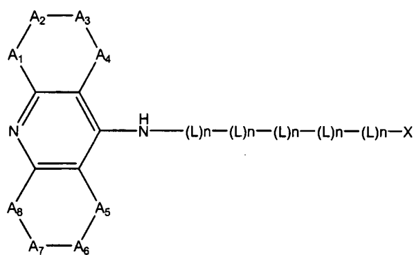
Formula I
