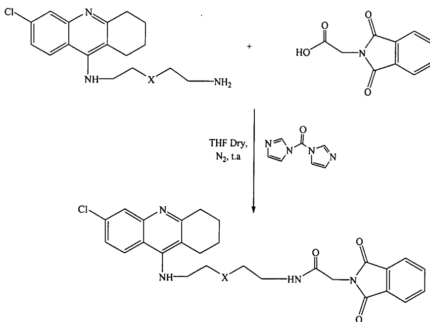
SCHEME 5
