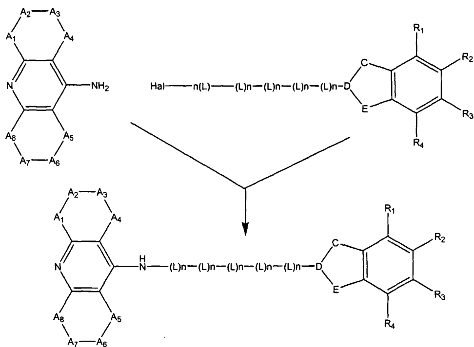
SCHEME 1b
