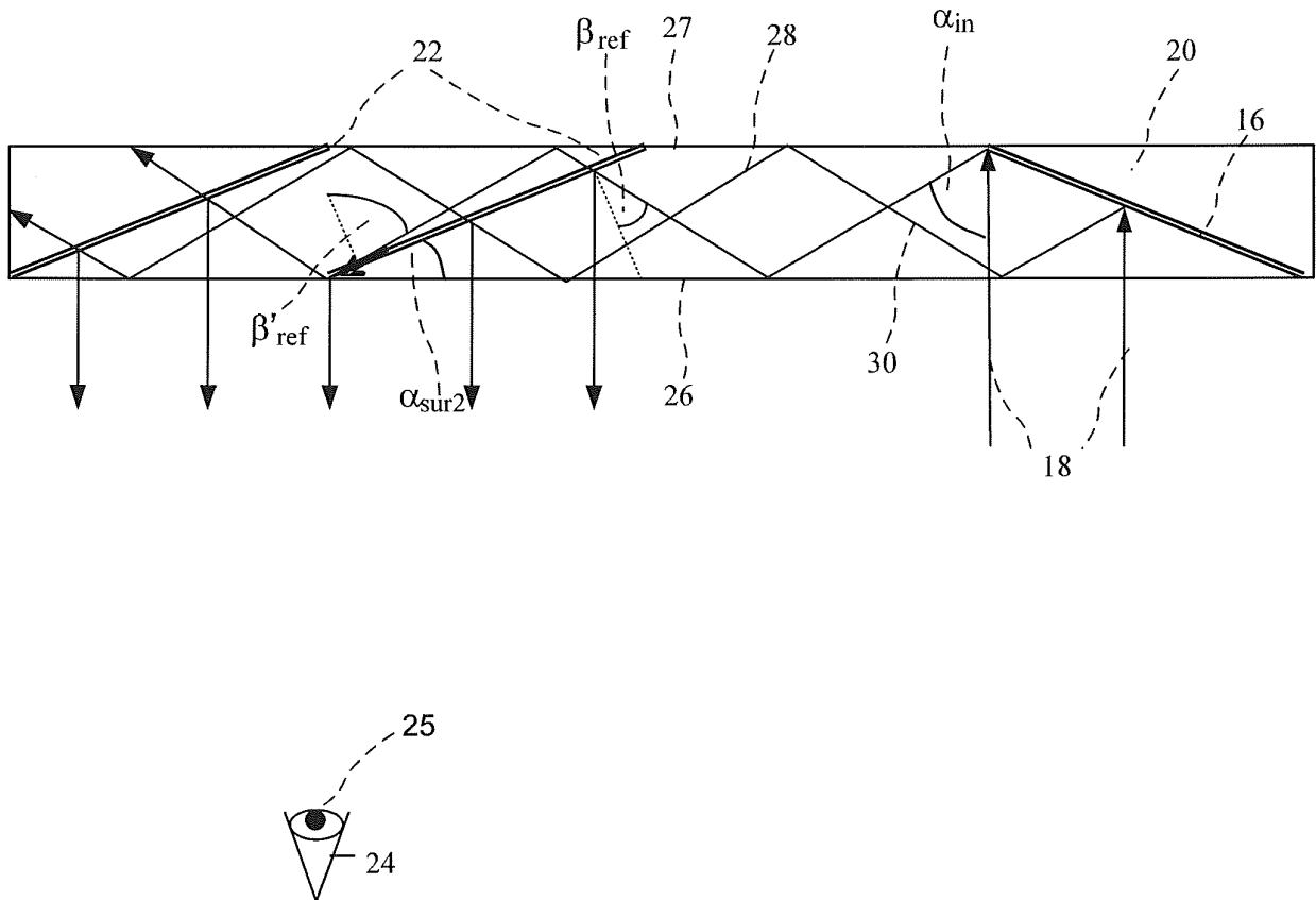
FIG. 1 (PRIOR ART)
