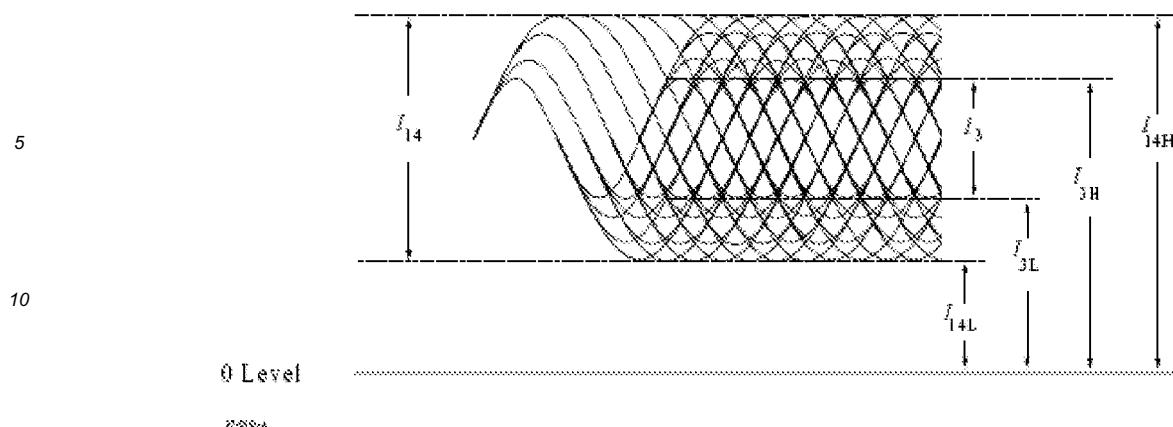
Figure 11 - Modulated amplitude
