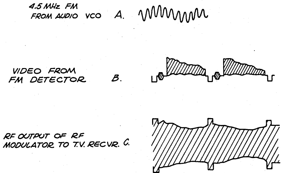
FIG. 25 RF MODULATOR
