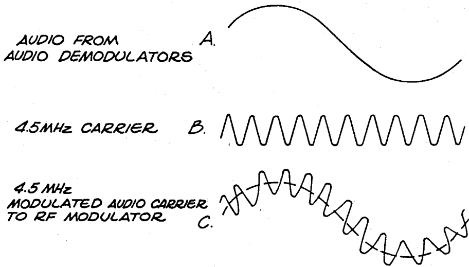
FIG. 23 4.5MHz VCO AUDIO MODULATOR
