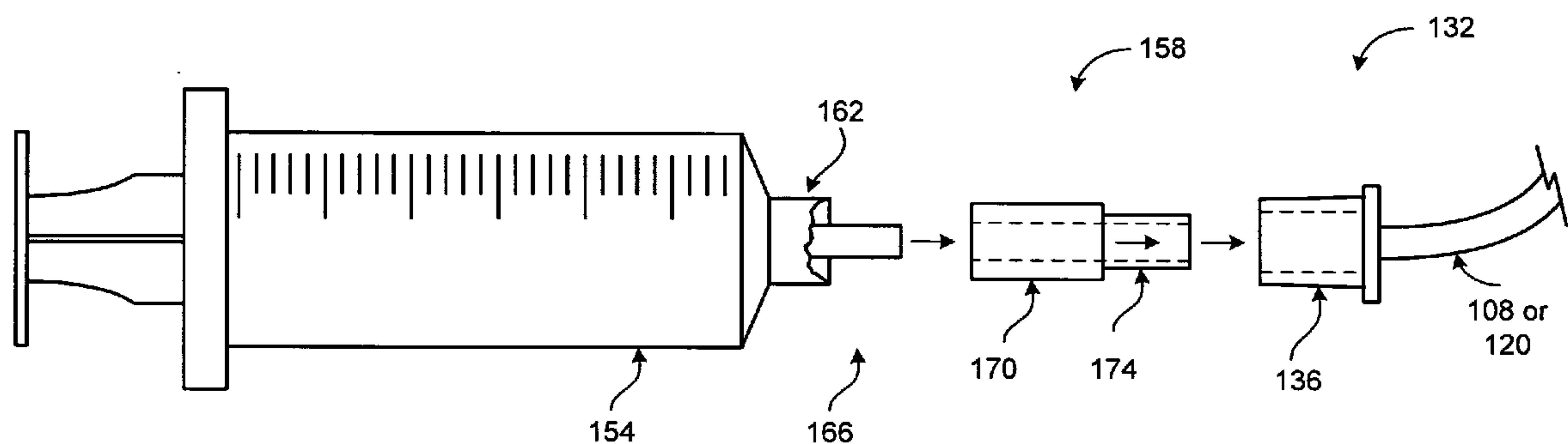
Fluid delivery system 150
