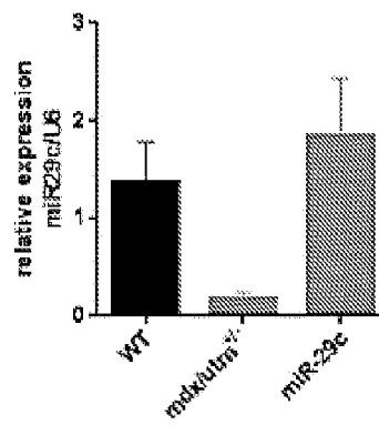
Figure 2C miR-29c
