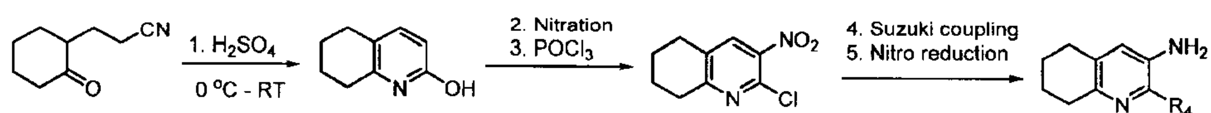
Scheme 5 (Part of this scheme was described in US2008/161340 A1)
