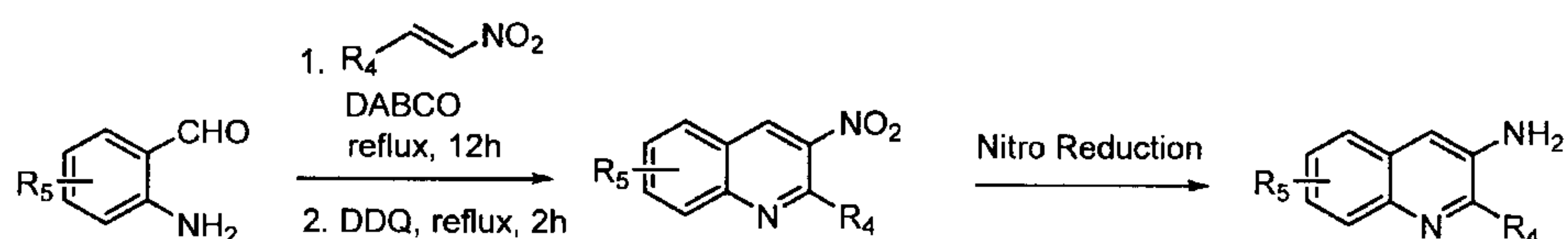
Scheme 3 (This scheme was described in WO2014062667 A1)
