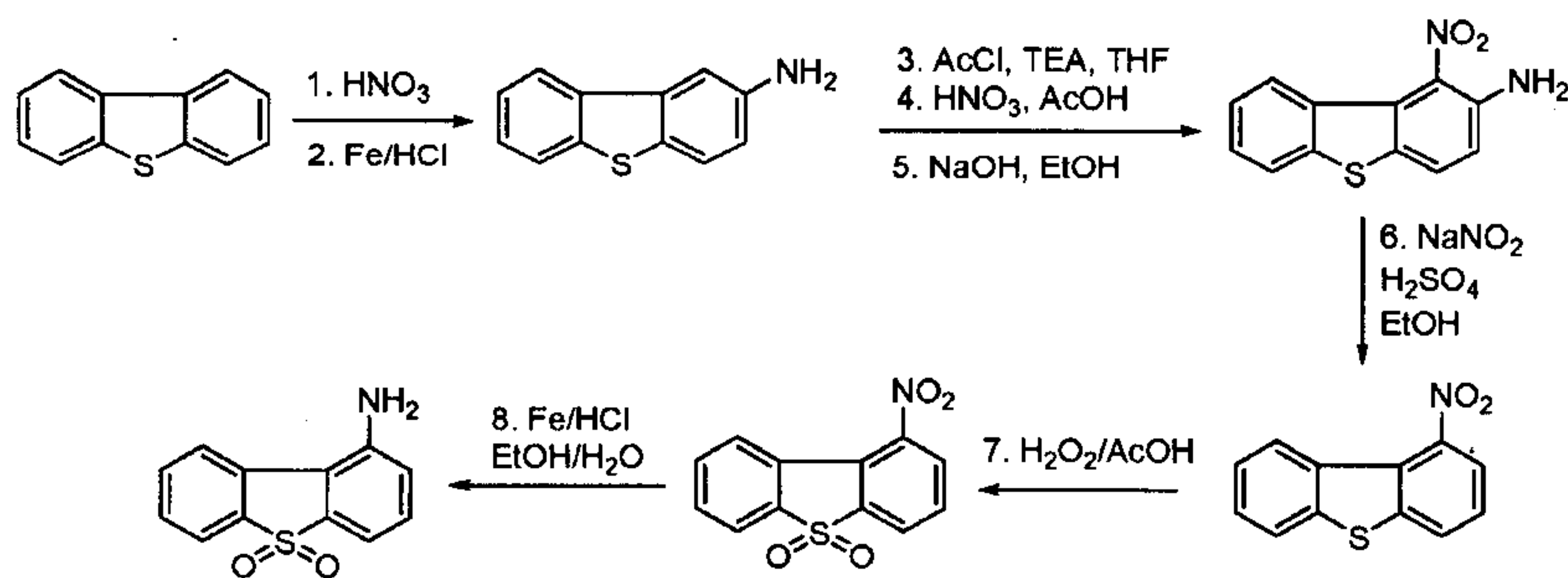
5 Scheme 8 (This scheme was described in J. Am. Chem. Soc. , 1954, 76, 2906–2908)
