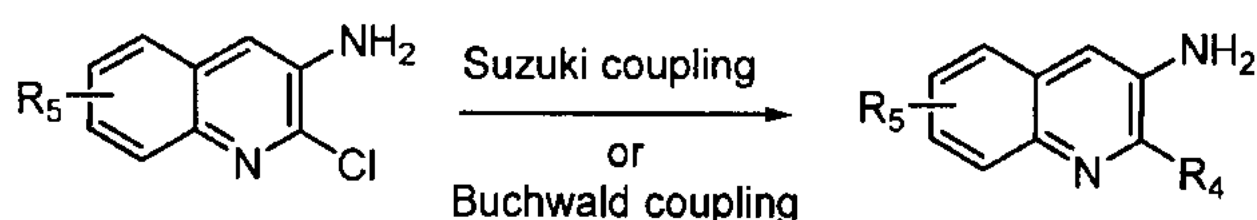
Scheme 5 (Part of this scheme was described in US2008/161340 A1)
