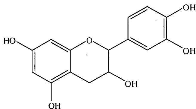
(2 R ,3 S )-2-(3,4-dihydroxyphenyl)-3,4-dihydro-2 H -chromene-3,5,7-triol
