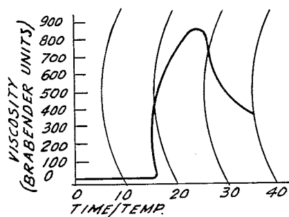
AMYLOGRAPH CURVE OF TAPIOCA STARCH.
