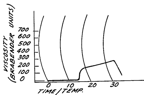
AMYLOGRAPH CURVE OF CHEMICALLY MODIFIED TAPIOCA STARCH.
