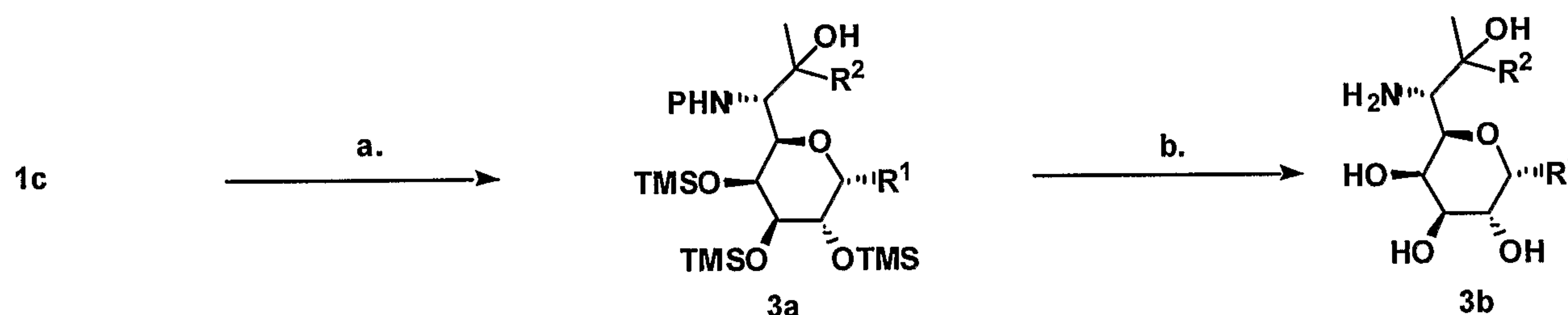
Scheme 3. General synthesis of lincosamine intermediate 3b.
