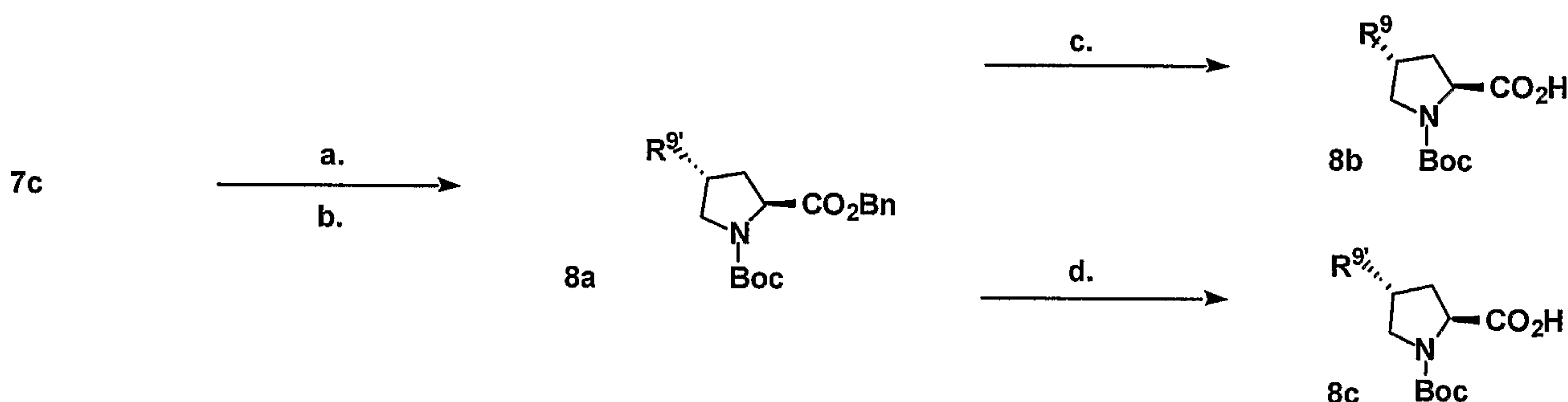
Scheme 8. General synthesis of trans - \text{R}^9 -substituted prolines 8c , wherein \text{R}^9 is alkenyl or substituted alkenyl, and 8b wherein \text{R}^9 is the saturated form of \text{R}^9 .
