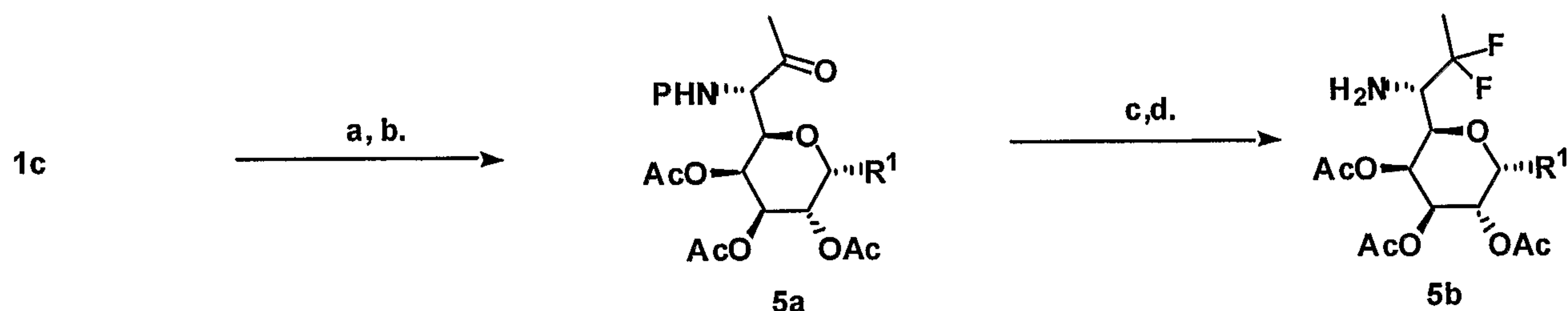
Scheme 5. General synthesis of 7-deoxy-7,7-difluorolincosamines 5b.
