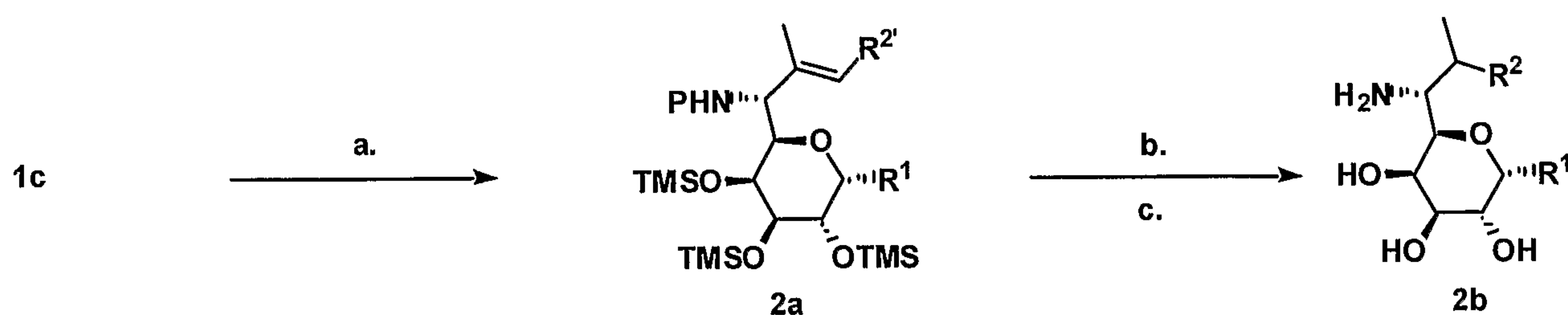
Scheme 2. General synthesis of lincosamine intermediate 2b.
