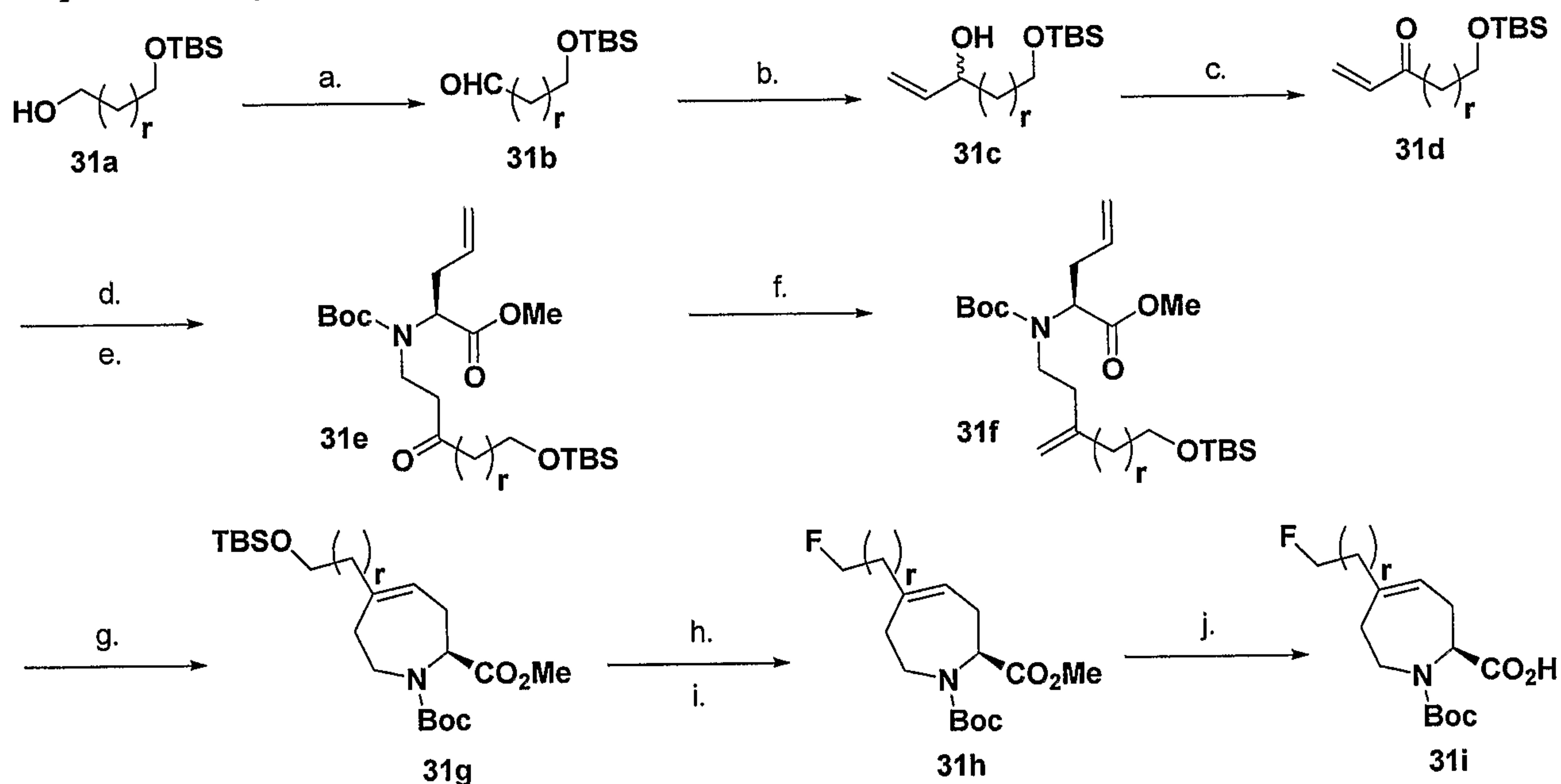
Scheme 31. Synthesis of 5-( \omega -Fluoro-alkyl)-azepane-2-carboxylic acid ( 31i ), r = 0-7 .
