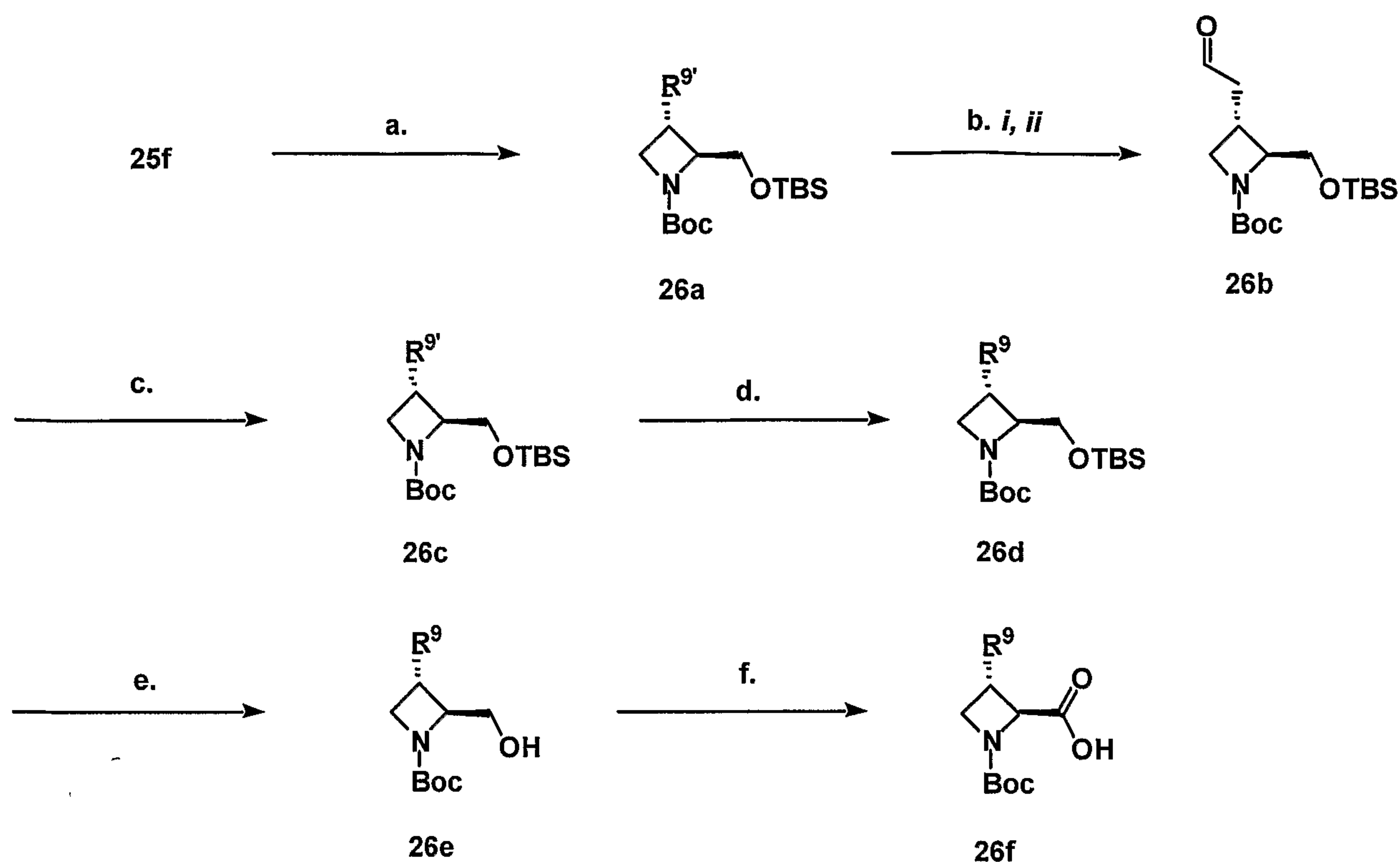
Scheme 26. General synthesis of trans -alkylazetidinecarboxylic acids via aldehyde.
