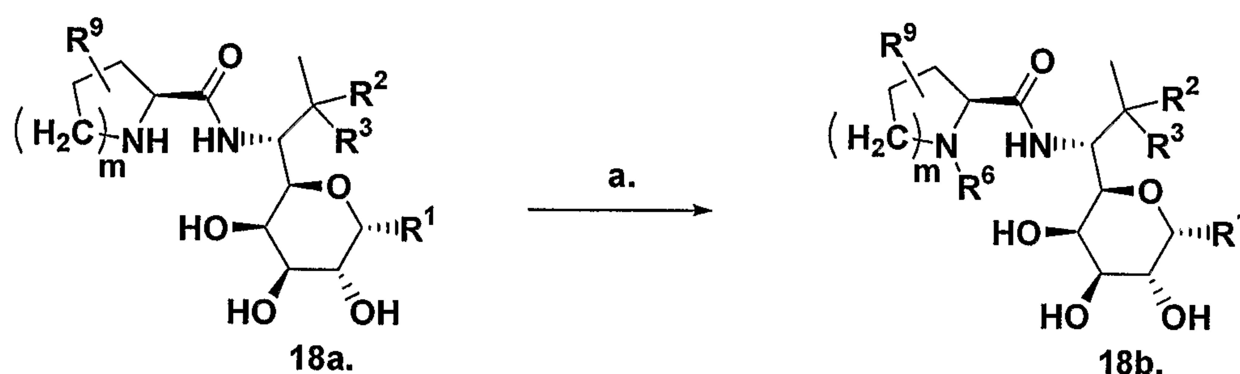
Scheme 19. General synthesis of 1'- N -substituted lincosamides. (a) alkylating agents
