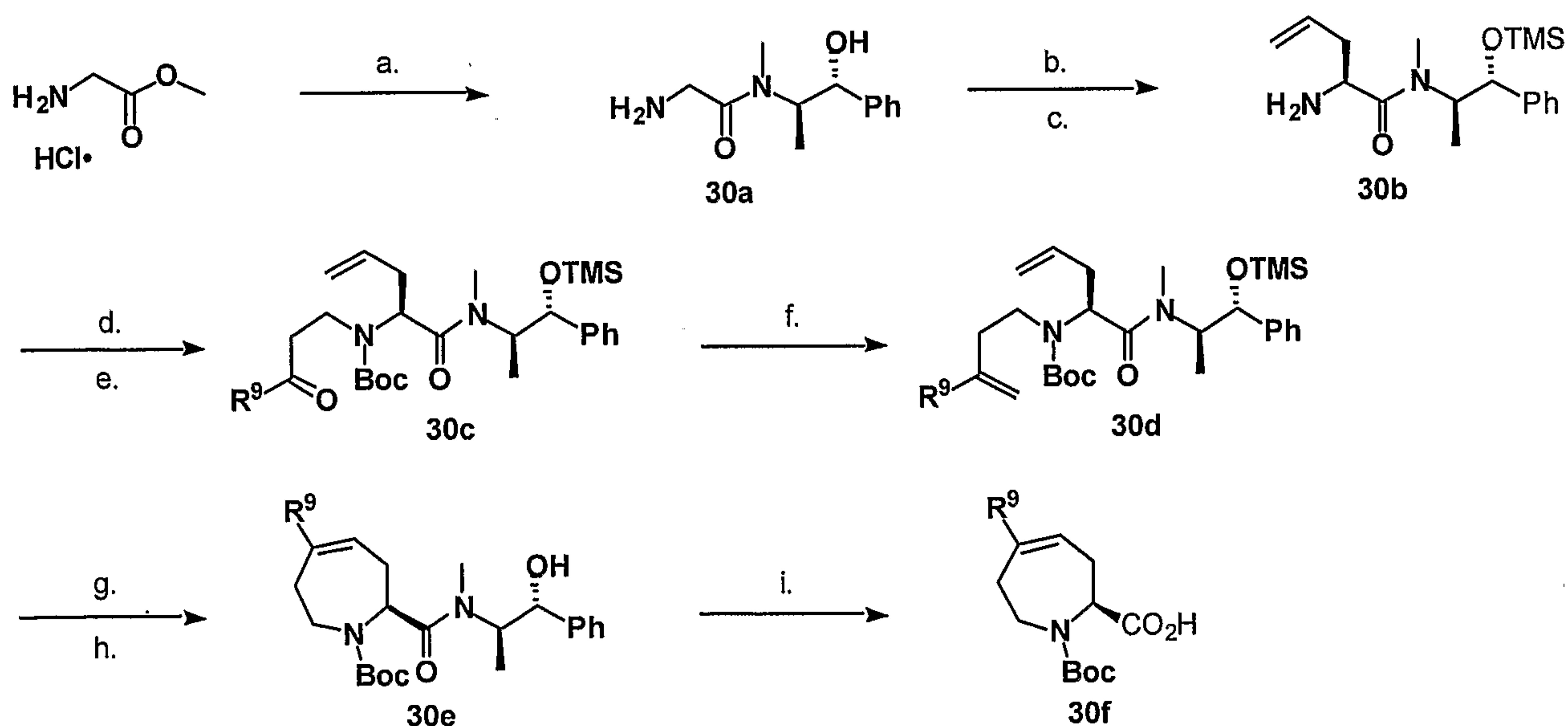
Scheme 30. (a) \text{LiO}t\text{-Bu} , (1R, 2R)-pseudoephedrine, THF (b) allylbromide, \text{LiHMDS} , \text{LiCl} , THF, 0^\circ\text{C} . (c) \text{TMSCl} , TEA (d) 1-octen-3-one ( R^9 = n\text{-pentyl} ), EtOH; (e) \text{Boc}_2\text{O} ; (f) methyltriphenylphosphonium bromide, t\text{-BuOK} , toluene; (g) (1,3-bis(2,4,6-
