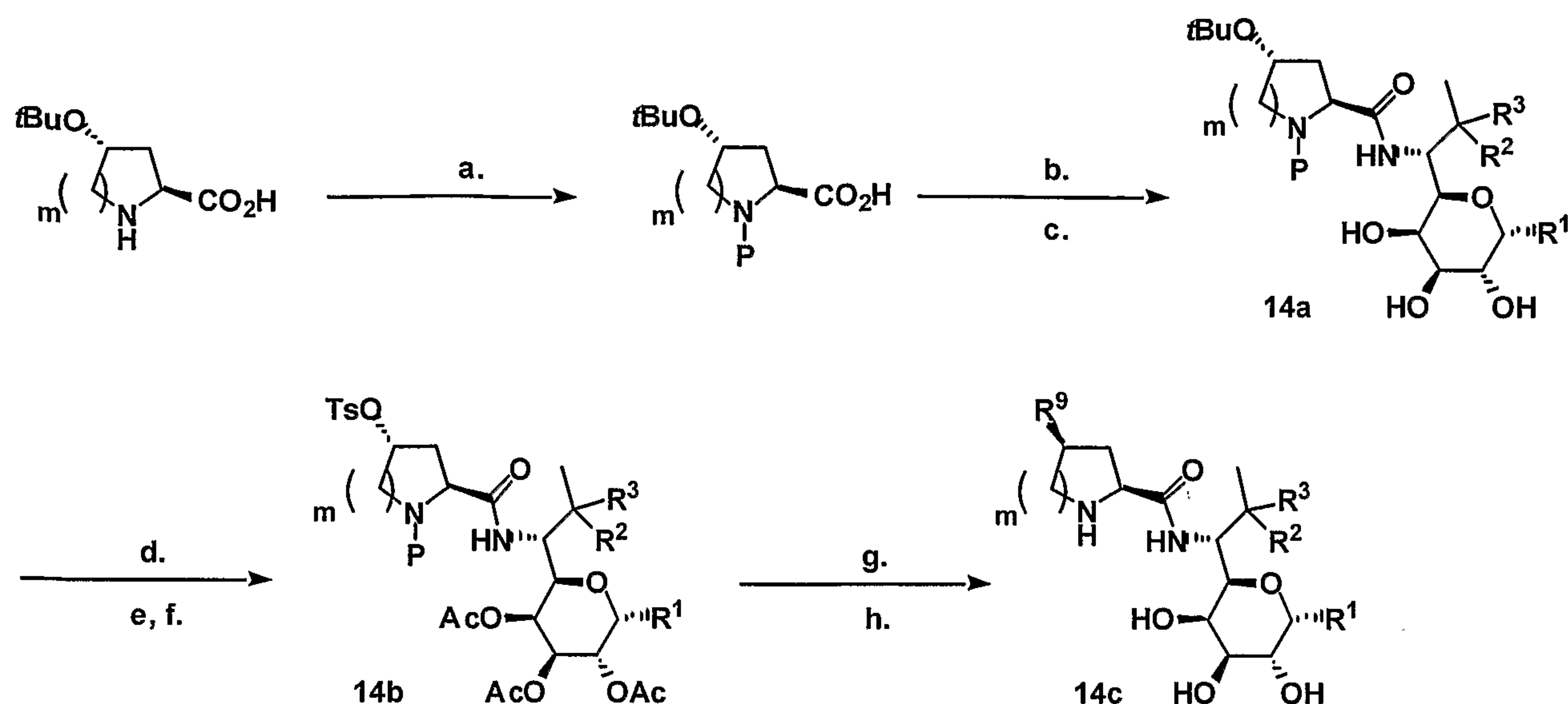
Scheme 14. General synthesis of 4-thioetherlincosamides 14c.
