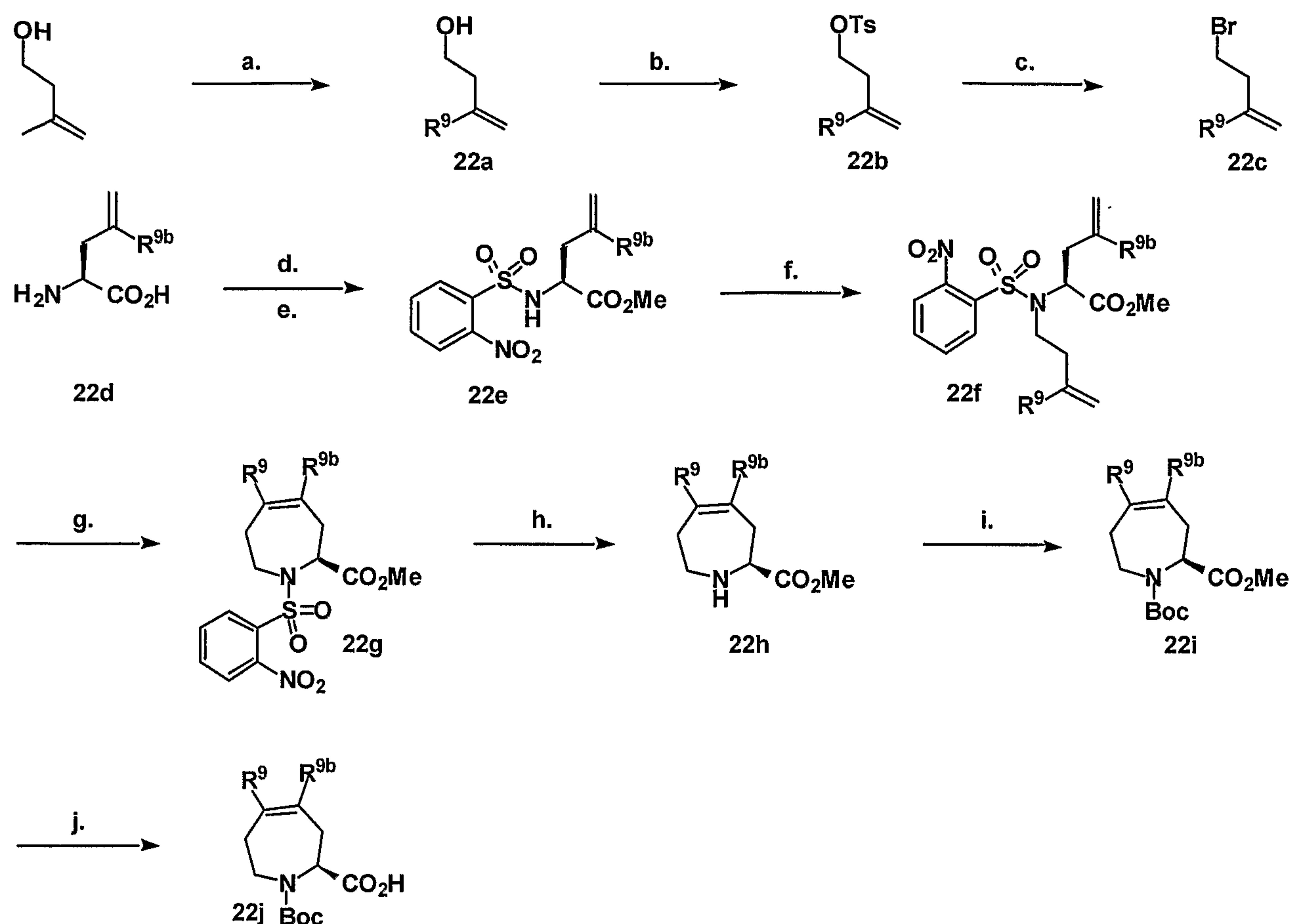
Scheme 22. (a) (i) BuLi, Et 2 O, TMEDA (ii) alkylbromide (b) TsCl TEA, DMAP (c) LiBr (d) H + , MeOH (e) 2-nitrobenzenesulfonyl chloride, Et 2 O-aq. NaHCO 3 (f) PPh 3 , DIAD, 22a , THF or Cs 2 CO 3 , 22c DMF (g) Benzyldiene [1,3-bis(2,4,6-trimethylphenyl)-2-imidazolidinylidene] dichloro-(tricyclohexylphosphine)ruthenium, DCM (h) Organic base (7-methyl,1,5,7-triazabicyclo[4.4.0]dec-5-ene), thiophenol, DMF (i) (Boc) 2 O, THF (j) Aq. LiOH, Dioxane-H 2 O
