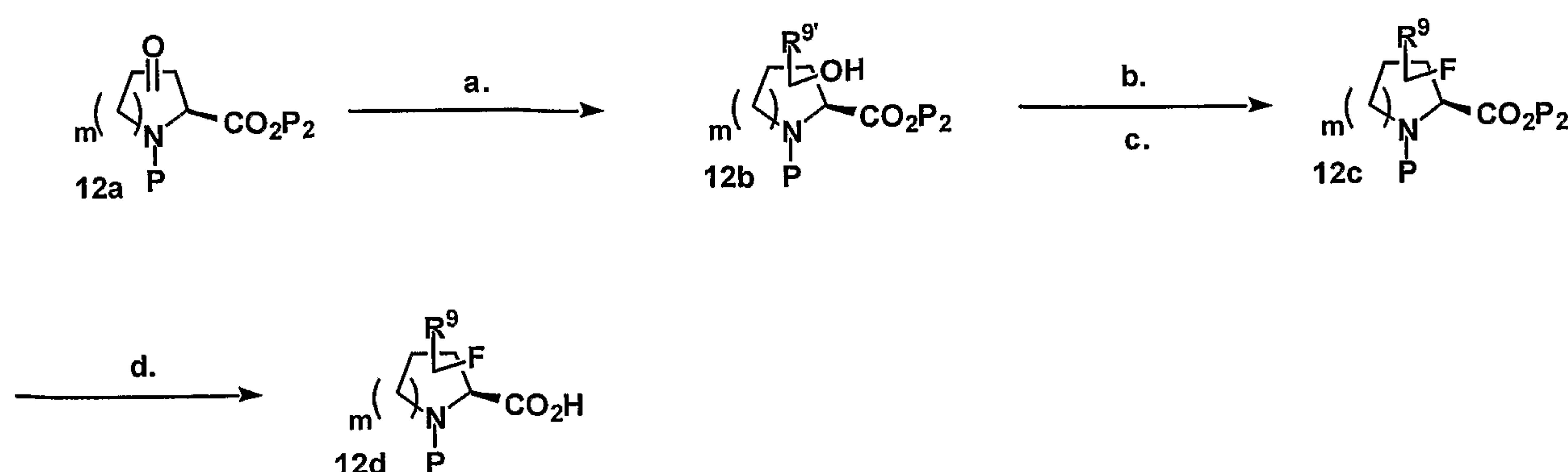
Scheme 12. General synthesis of fluorinated amino acid intermediate 12d from ketopyrrolidines ( m = 1 ), ketopiperidines ( m = 2 ), and ketoazepanes ( m = 3 ) 12a.
