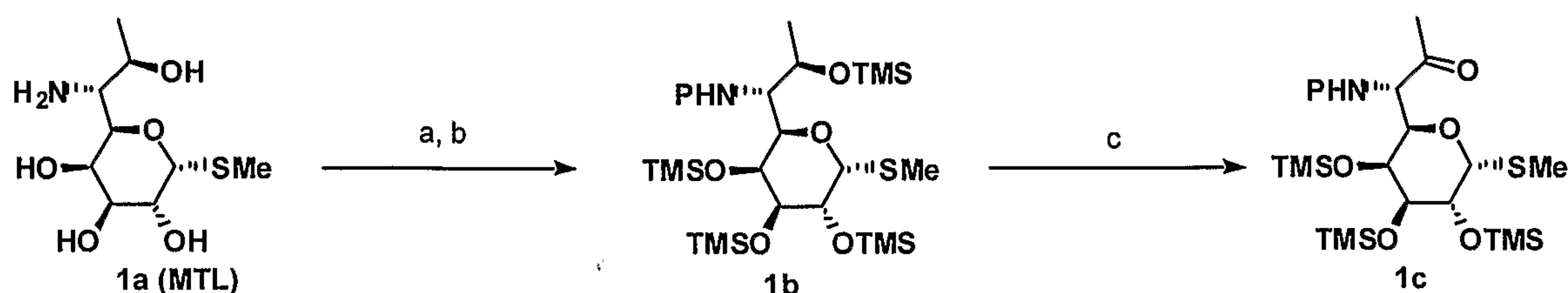
Scheme 1. General synthesis of lincosamine intermediate 1c.
