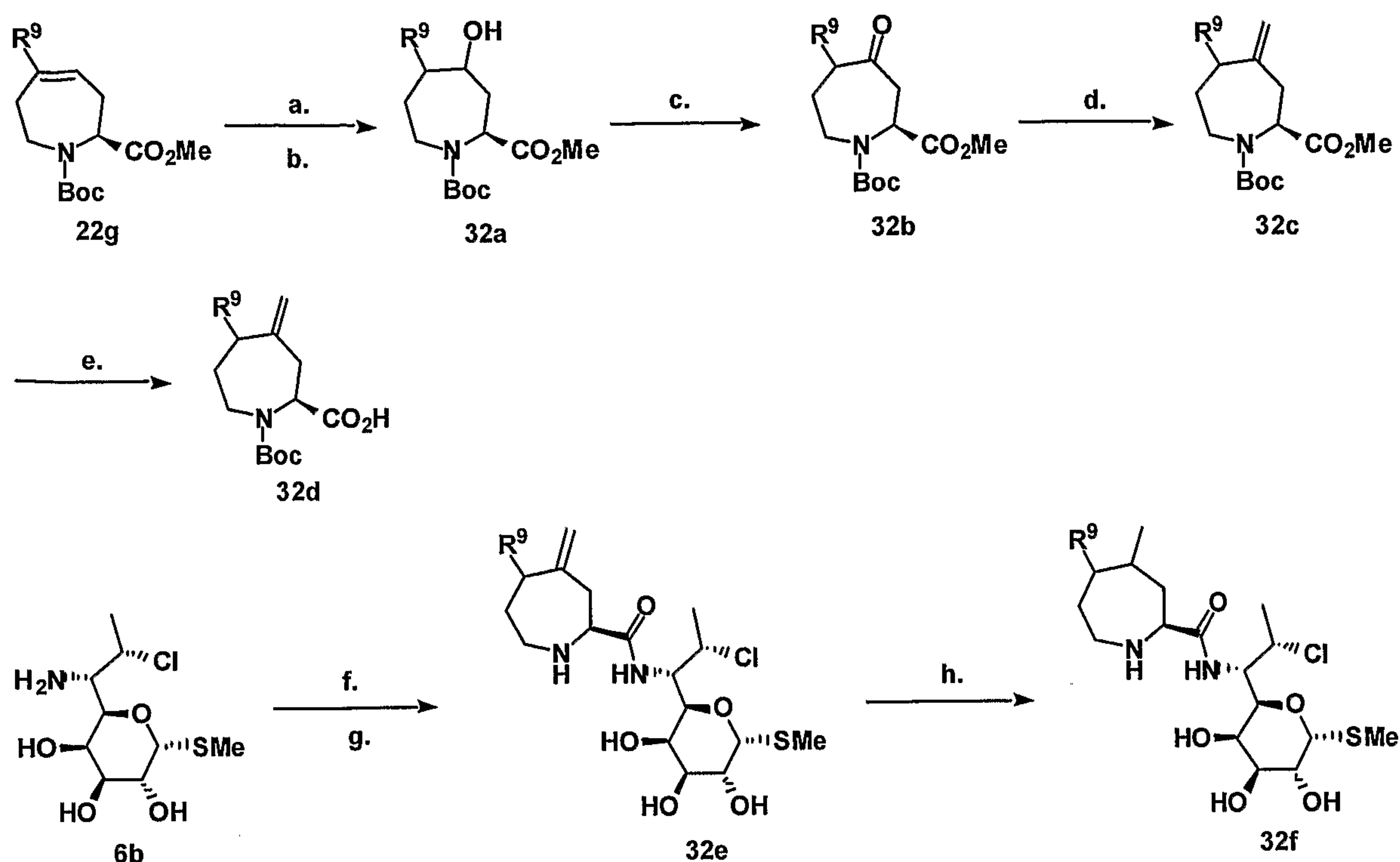
Scheme 32. Synthesis of 4-methyl-5-propyl-azepane-2-carboxylic acid [2-chloro-1-(3,4,5-trihydroxy-6-methylsulfanyl-tetrahydro-pyran-2-yl)-propyl]-amide (32f).
