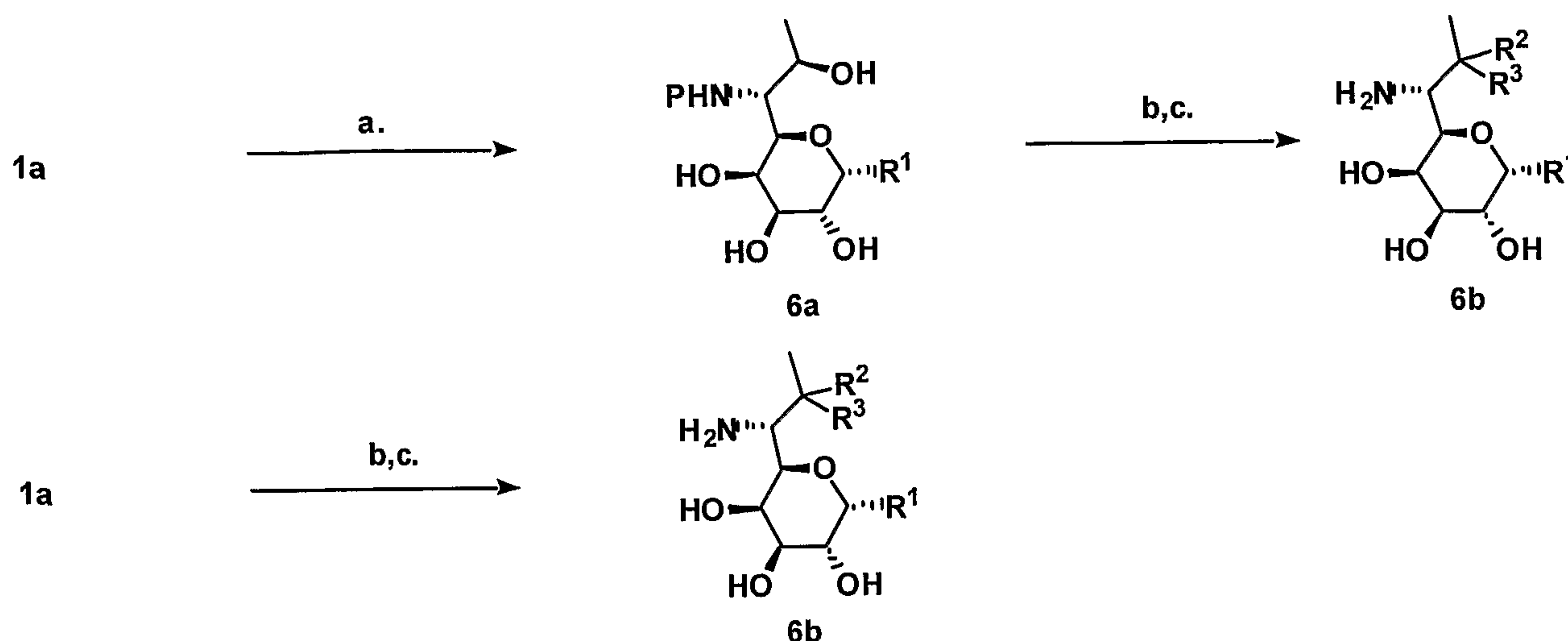
Scheme 6. General synthesis of 7-deoxy-7-halolincosamines 6b.
