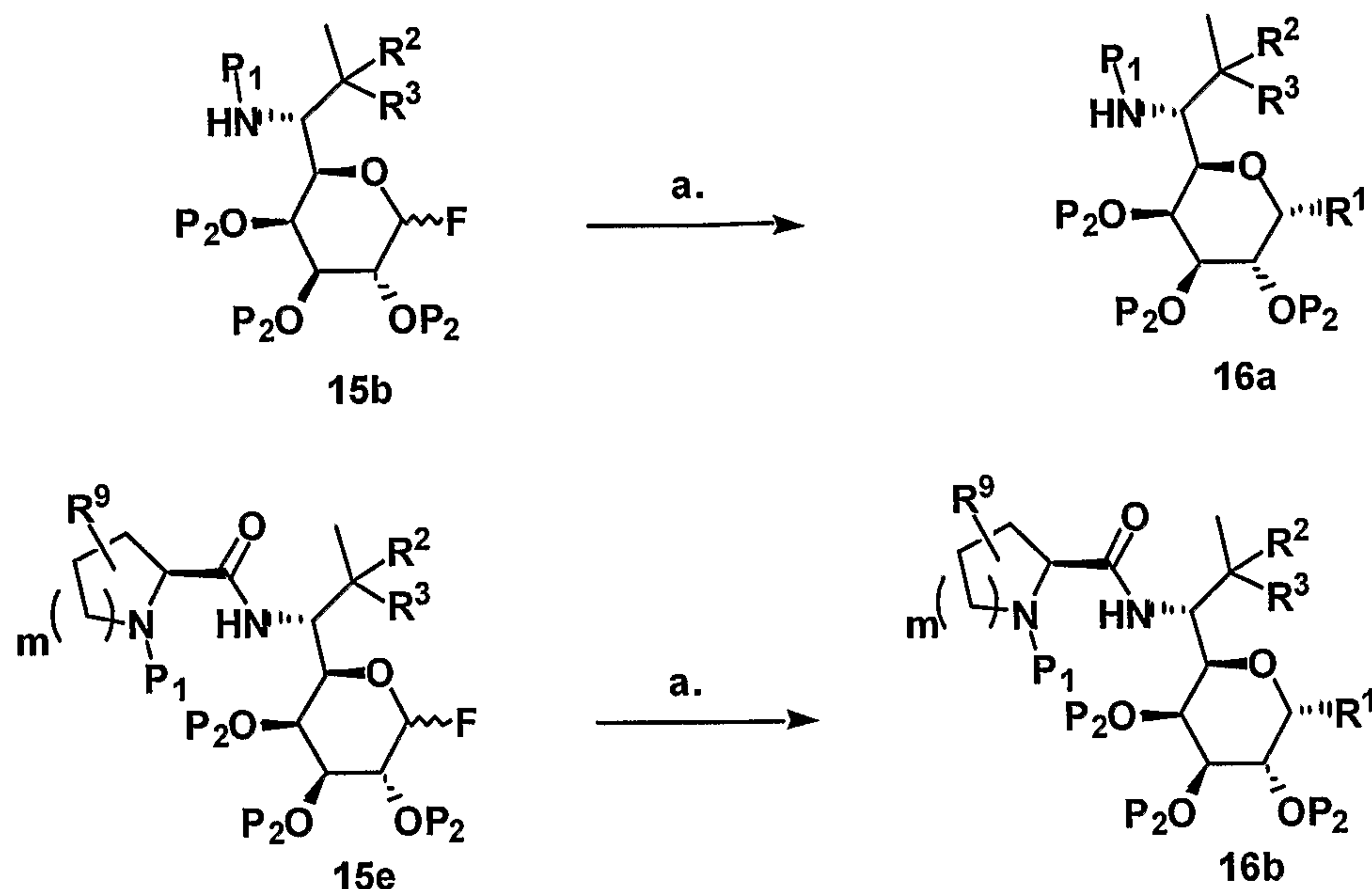
Scheme 16. Displacement of Fluoro by Sulfanyl Moiety
