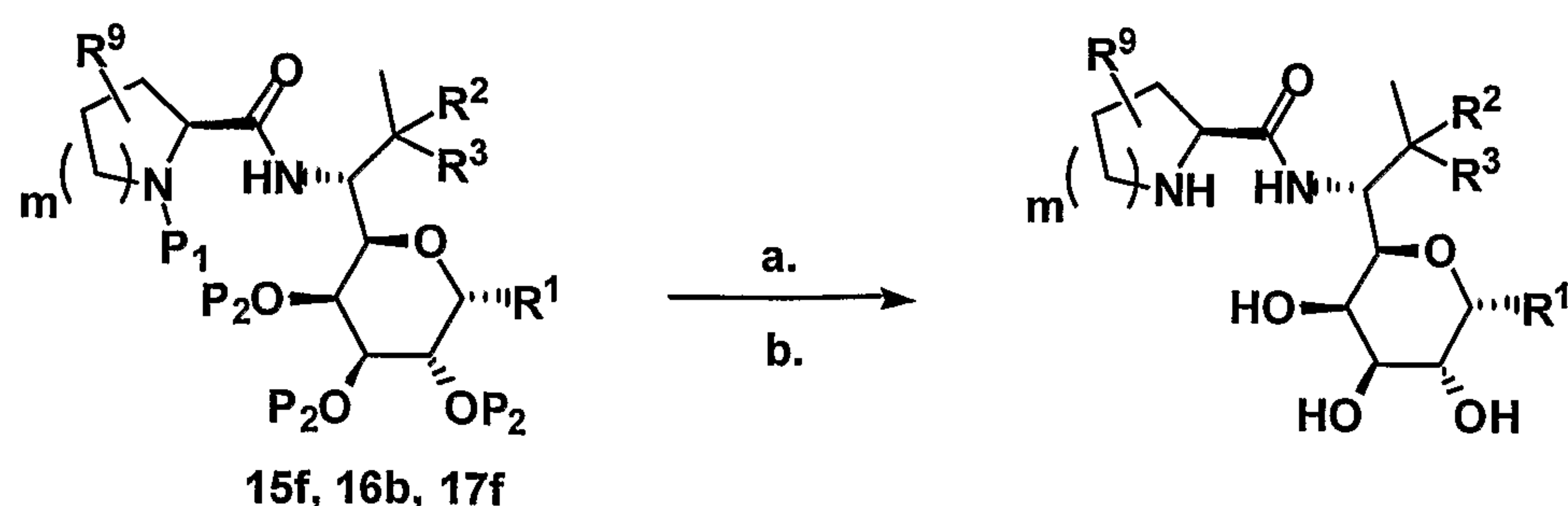
Scheme 18. Global deprotection 15f, 16b, and 17f to compounds of formula (I).
