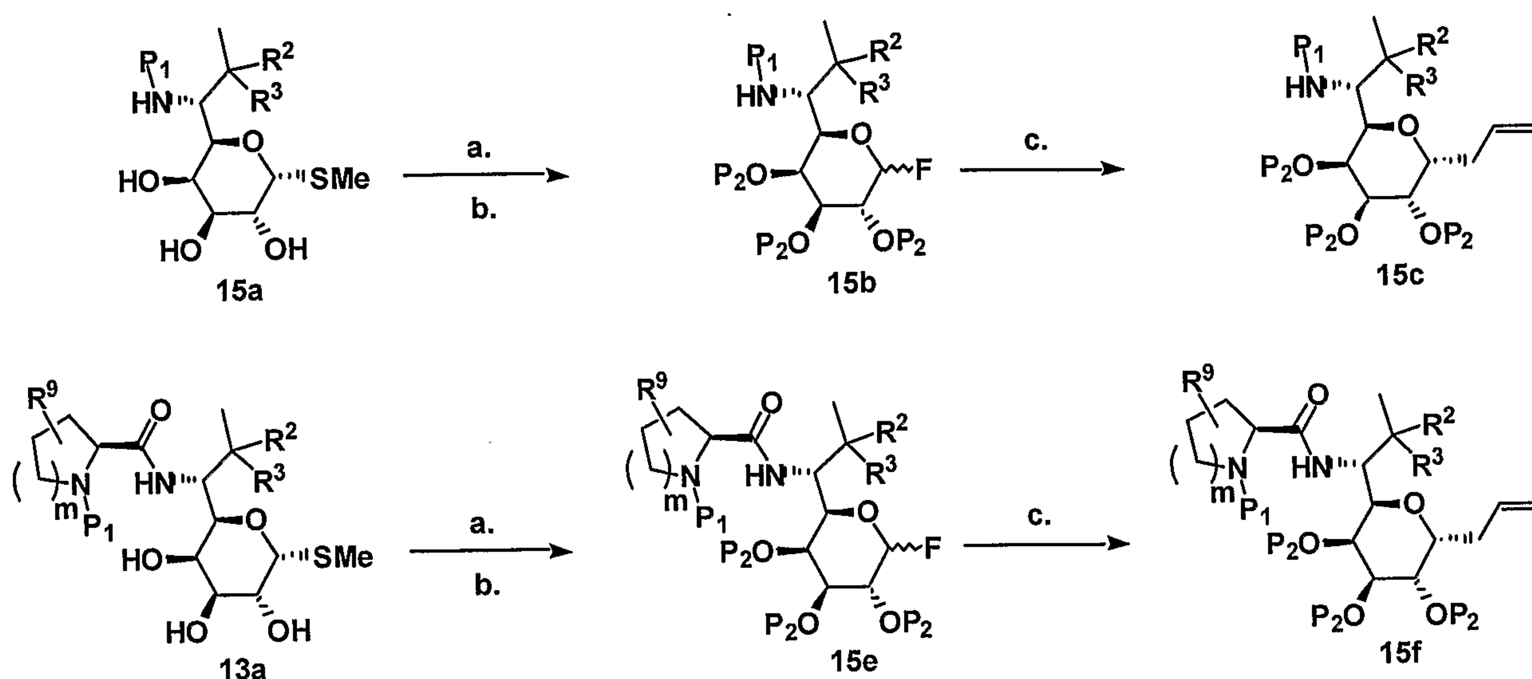
Scheme 15. General synthesis of protected 1-allylic intermediates 15b, 15c, 15e, and 15f.
