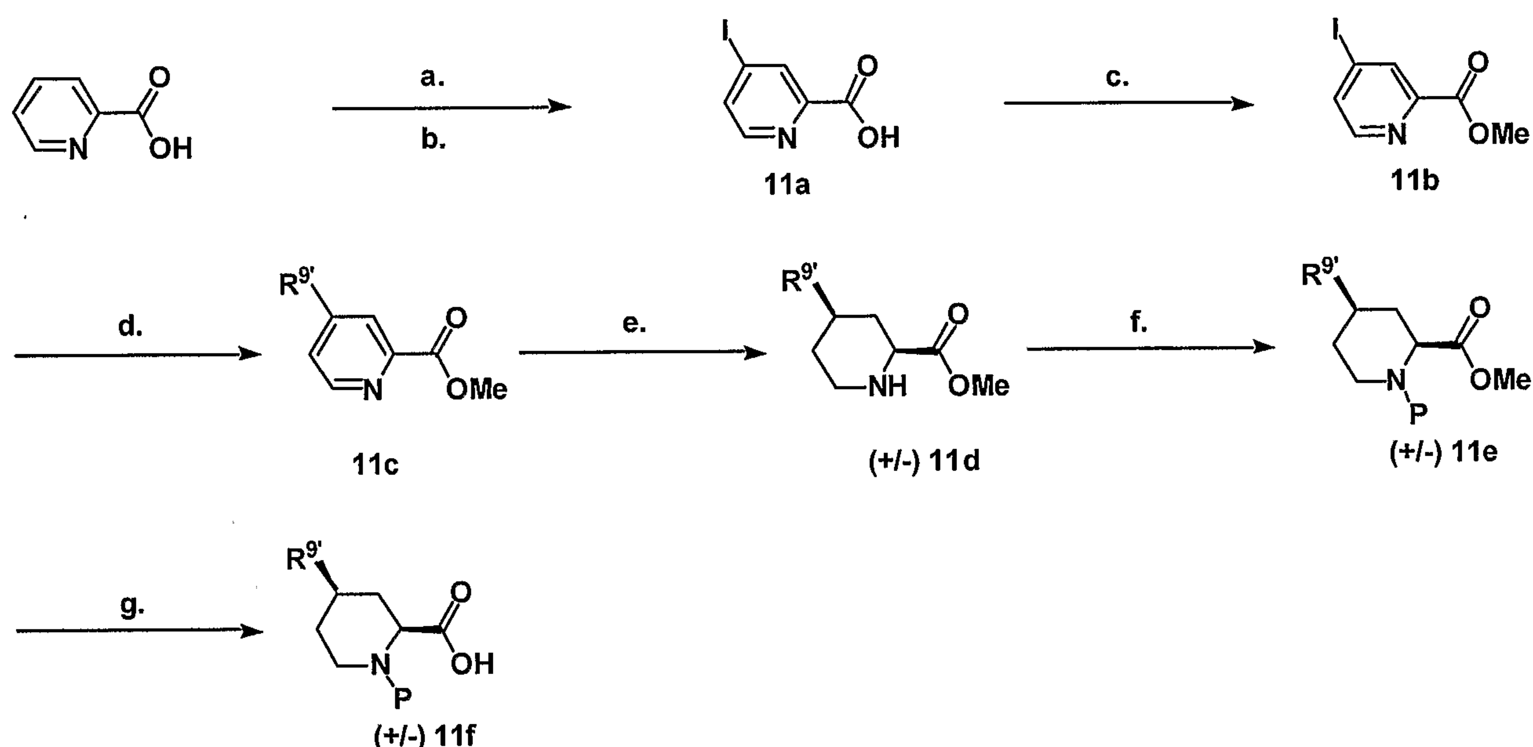
Scheme 11. General synthesis of 4-substituted intermediates 11c , 11d , and 11e .
