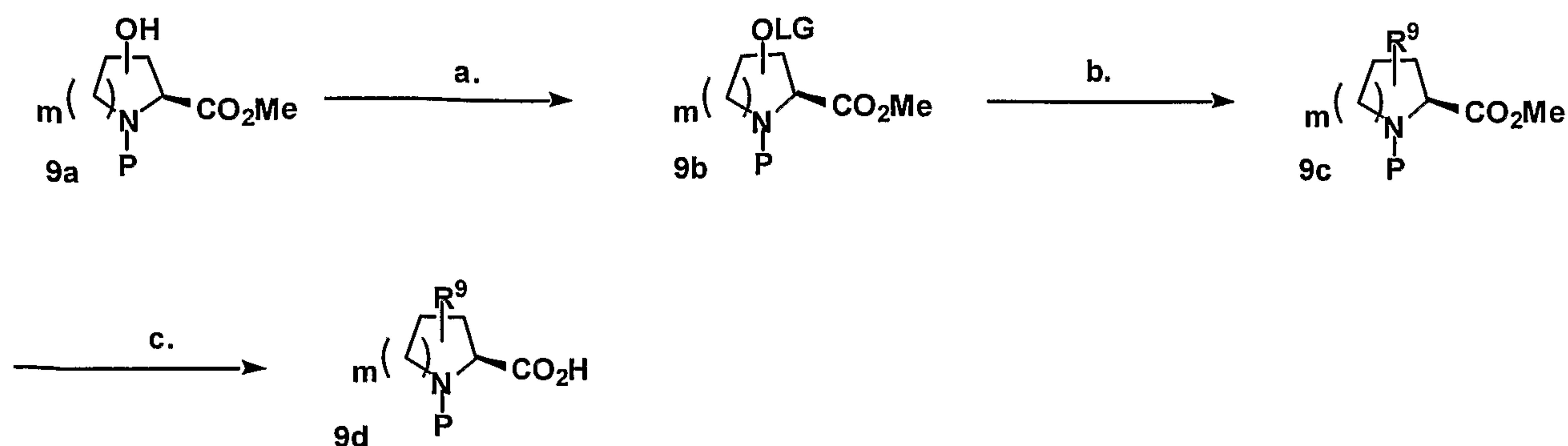
Scheme 9. General synthesis of cis -R 9 or trans -R 9 substituted cyclic amino acids 9d.(a)
