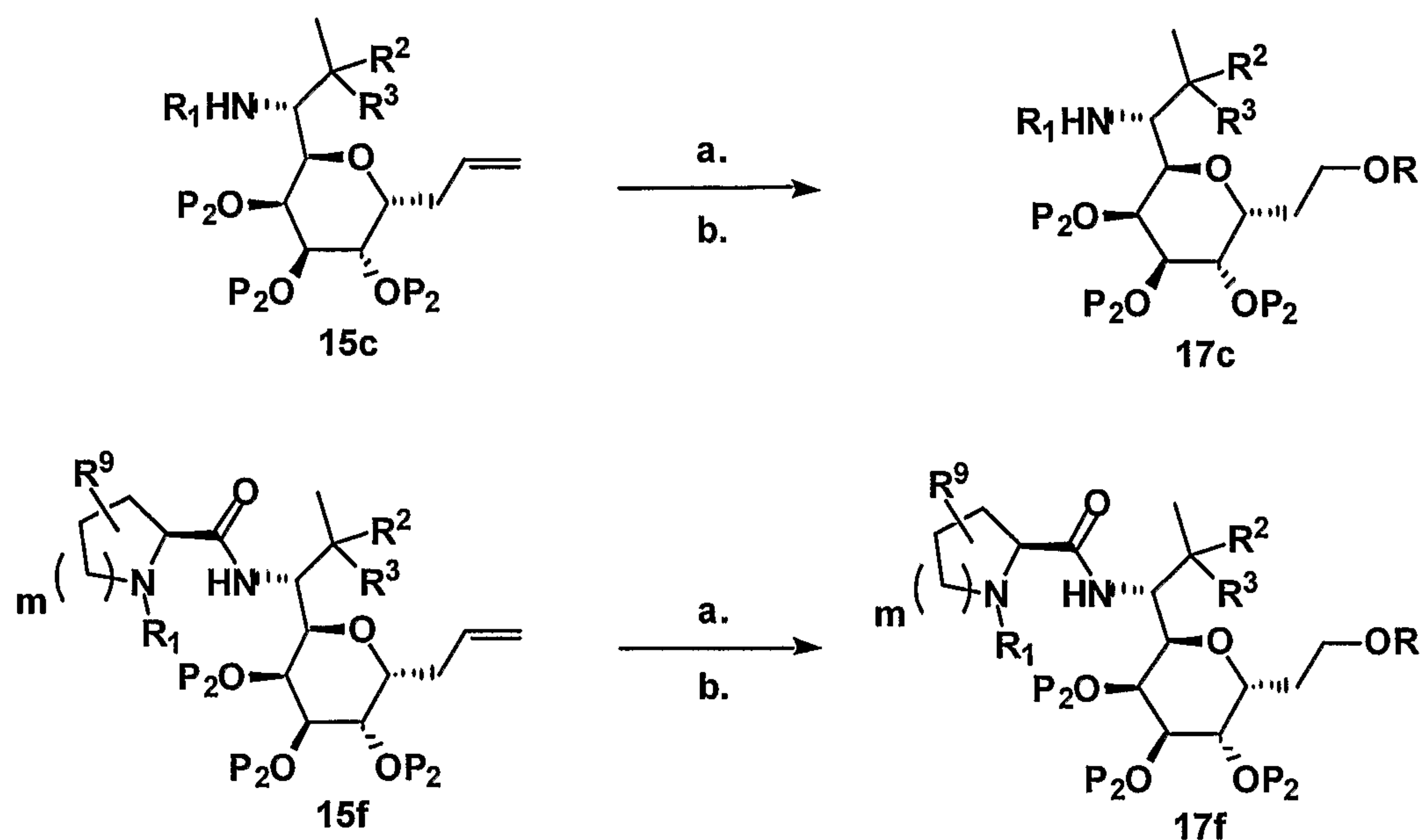
Scheme 17. General synthesis of alcohol and ether 1-position lincosamine derivatives
