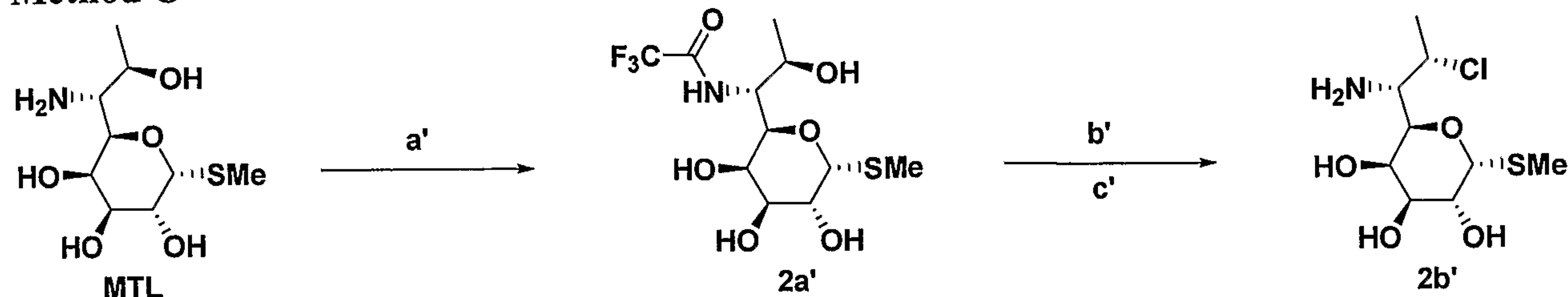
Scheme 2'. Preparation of 7-Chloro MTL (2b'). a. Methyl trifluoroacetate, TEA, MeOH. b. Chloromethylene piperidinium chloride. c. NaOH, aq. MeOH.
