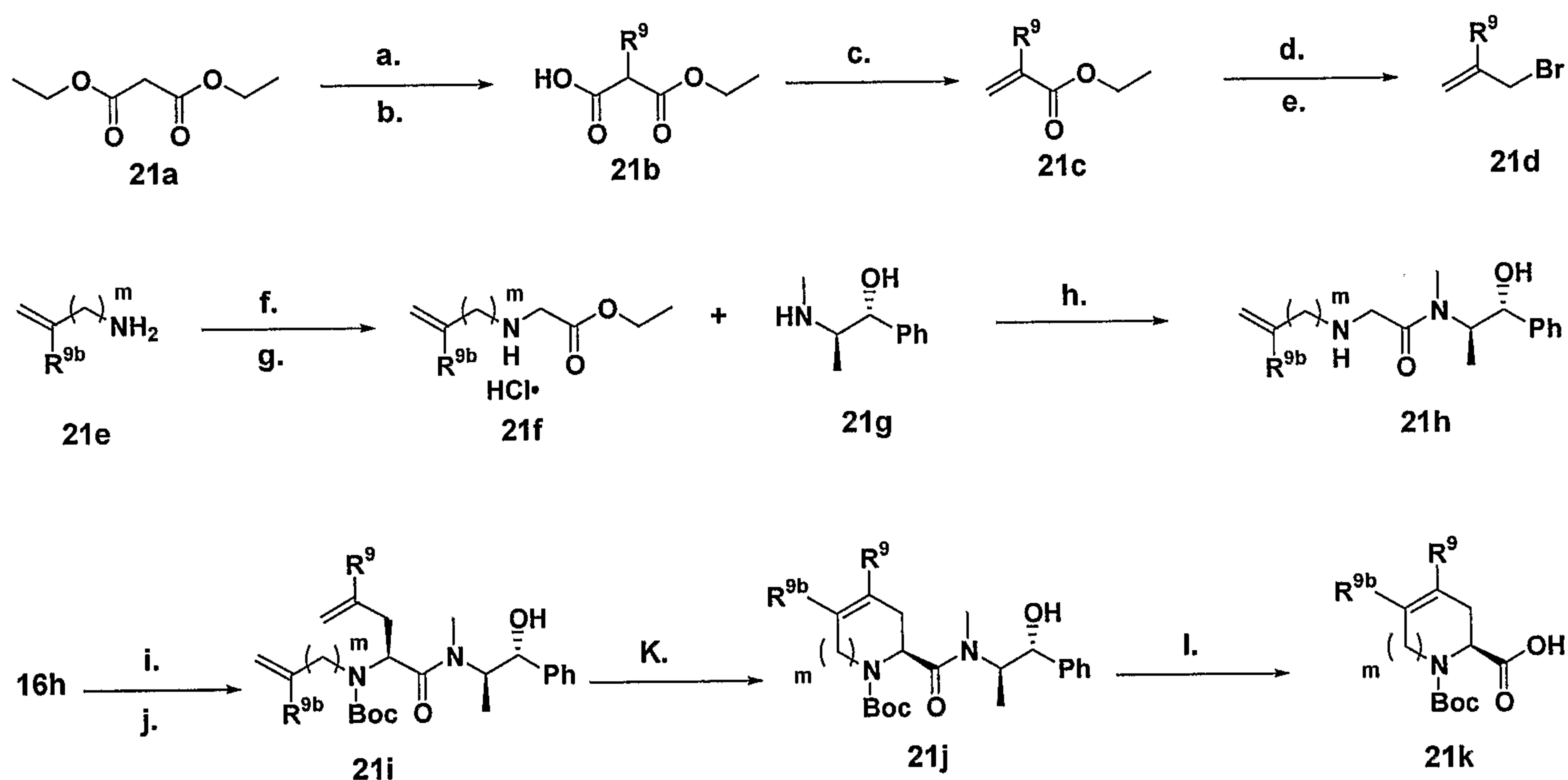
Scheme 21. (a) NaH, R^9 Br, DMF (b) KOH, H 2 O, EtOH (c) CH 2 O (aq), Piperidine, EtOH (d) DIBALH, CH 2 Cl 2 (e) PBr 3 , Et 2 O (f) ethyl bromoacetate (g) HCl/dioxane (h) LiOt-Bu, THF (i) 21d, LiHMDS, LiCl, THF, 0 °C (j) Boc 2 O, Et 3 N, CH 2 Cl 2 (k) olefin metathesis catalyst CH 2 Cl 2 (l) 1M NaOH (aq), MeOH.
