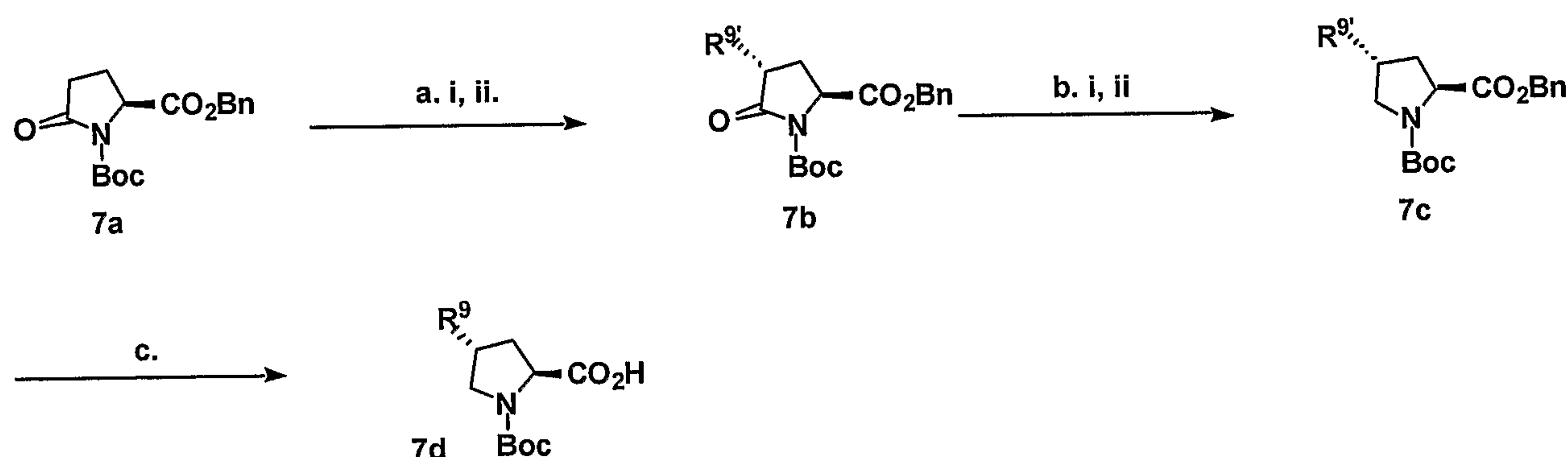
Scheme 7. General synthesis of trans -alkylprolines 7d .
