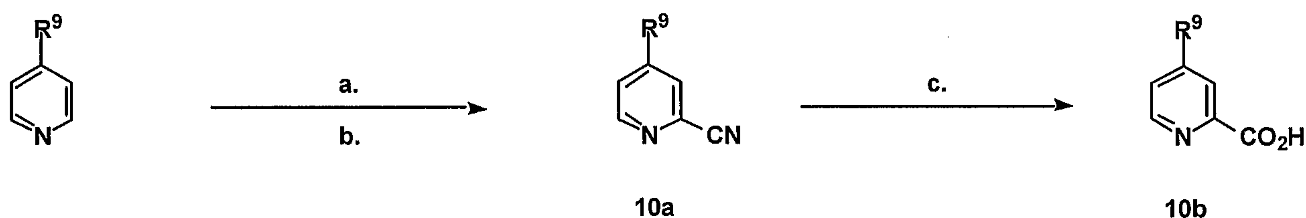
Scheme 10. General synthesis of substituted pyridin-2-yl carboxylic acids 10b.
