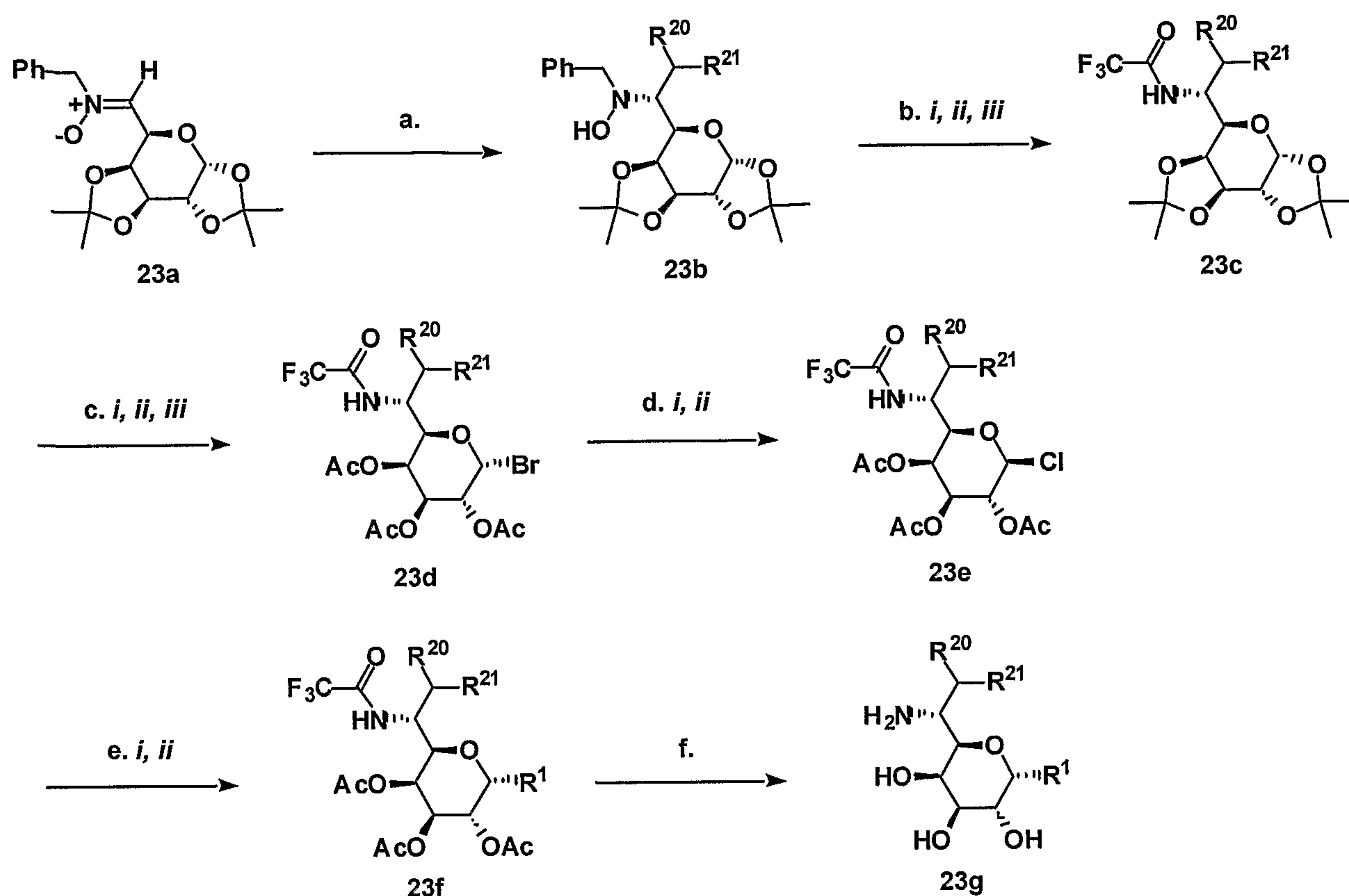
Scheme 23. General synthesis of C6 lincosamine derivatives.
