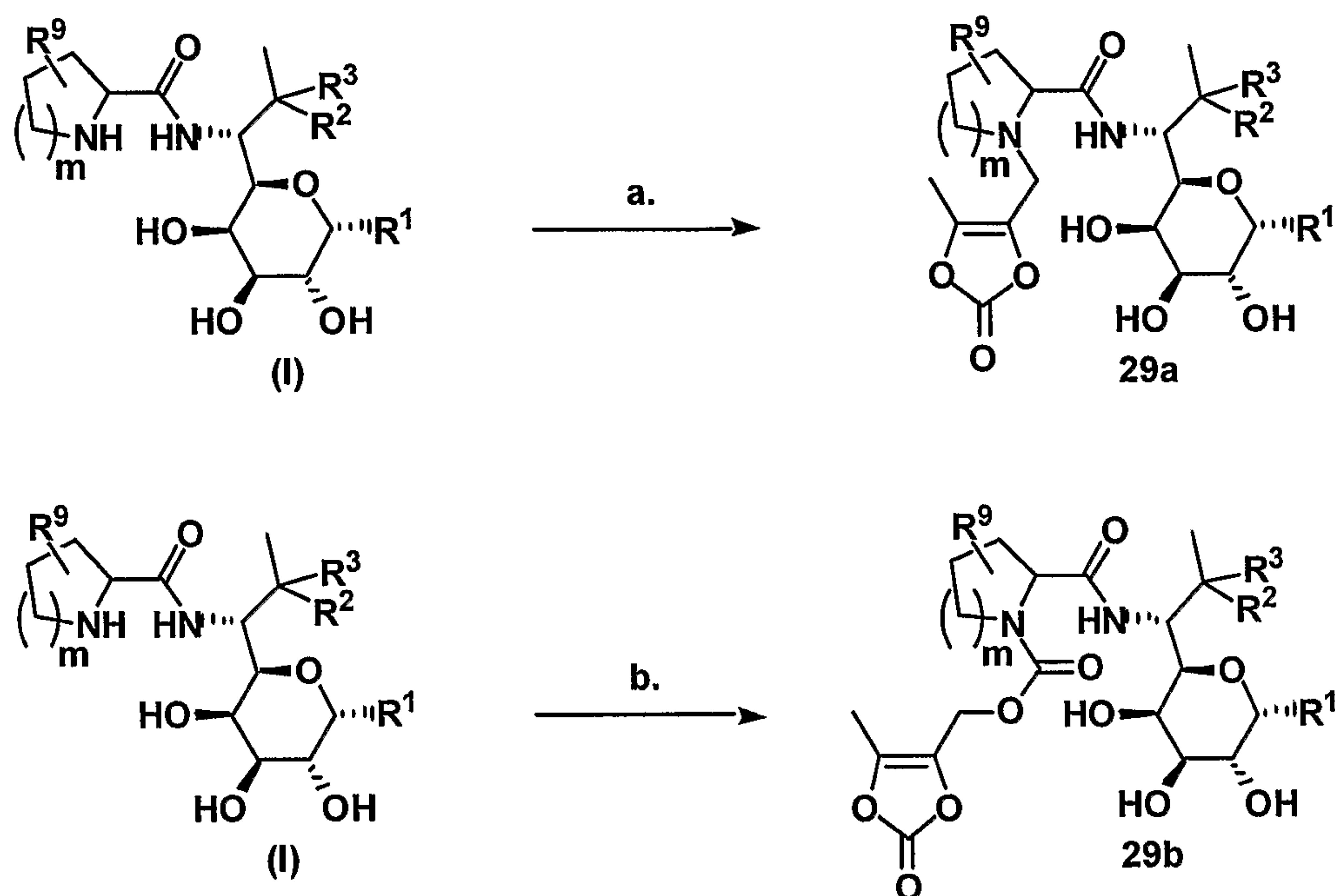
Scheme 29. general synthesis of R^6 dioxalinone prodrugs
