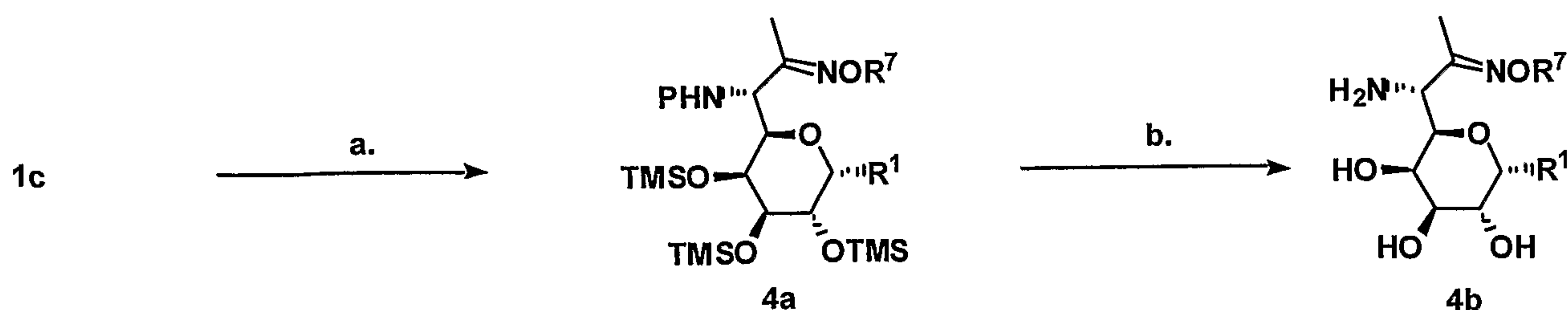
Scheme 4. General synthesis of 7-oxime-lincosamines 4b.
