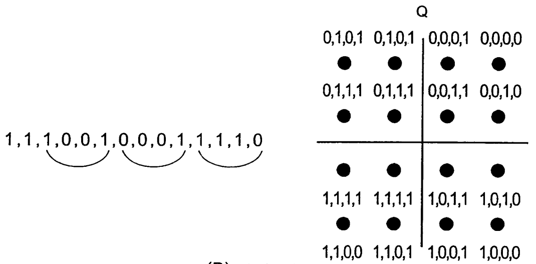
(B) 16QAM
