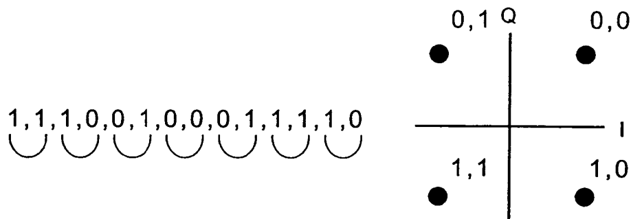
(A) QPSK
