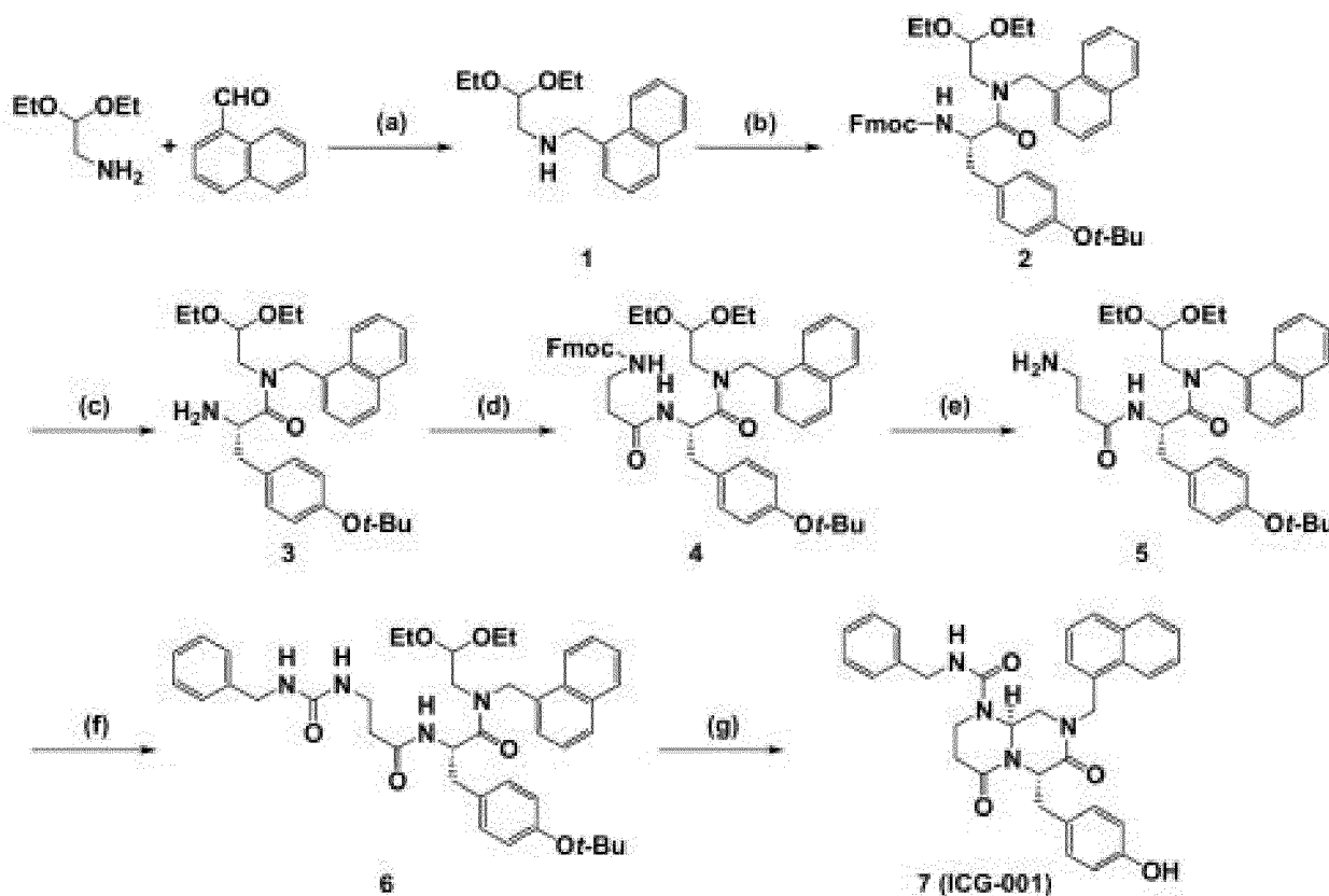
(Scheme 1) Synthesis of ICG-001 (a) \text{NaBH}_4 , EtOH (b) Fmoc-L-Tyr( t -Bu)-OH, HATU, DIEA, DMF (c) DEA, \text{CH}_2\text{Cl}_2 (d) Fmoc- \beta -Ala-OH, HATU, DIEA, DMF (e) DEA, \text{CH}_2\text{Cl}_2 (f) \text{BnNCO} , \text{CH}_2\text{Cl}_2 (g) \text{HCO}_2\text{H}
