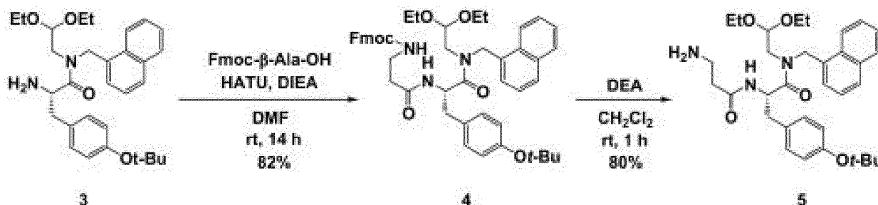
(1-4) Synthesis of Compound 5
