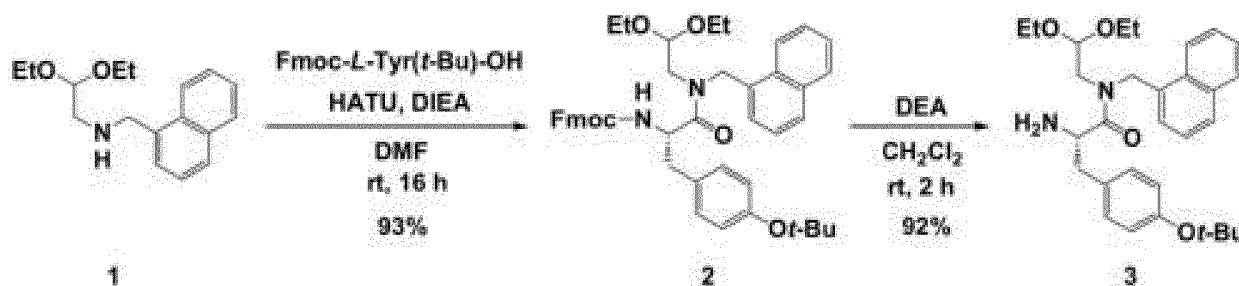
(1-3) Synthesis of Compound 3
