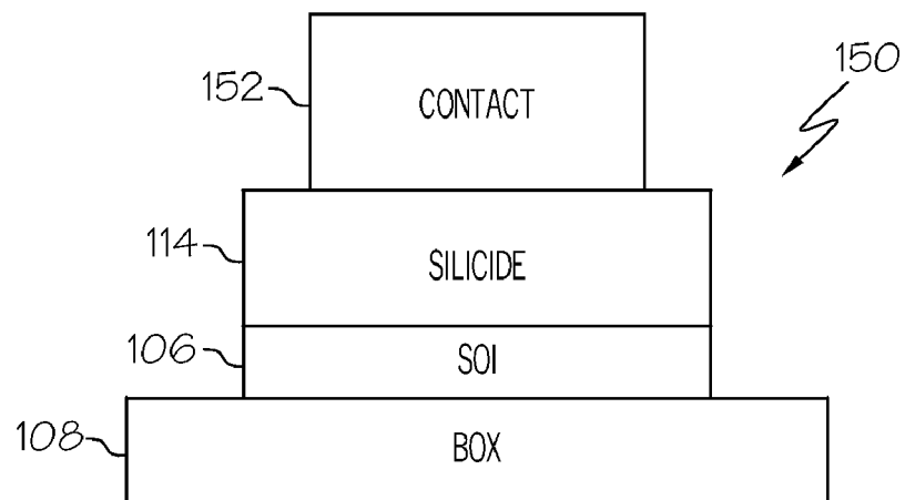
FIG. 4 (PRIOR ART)
