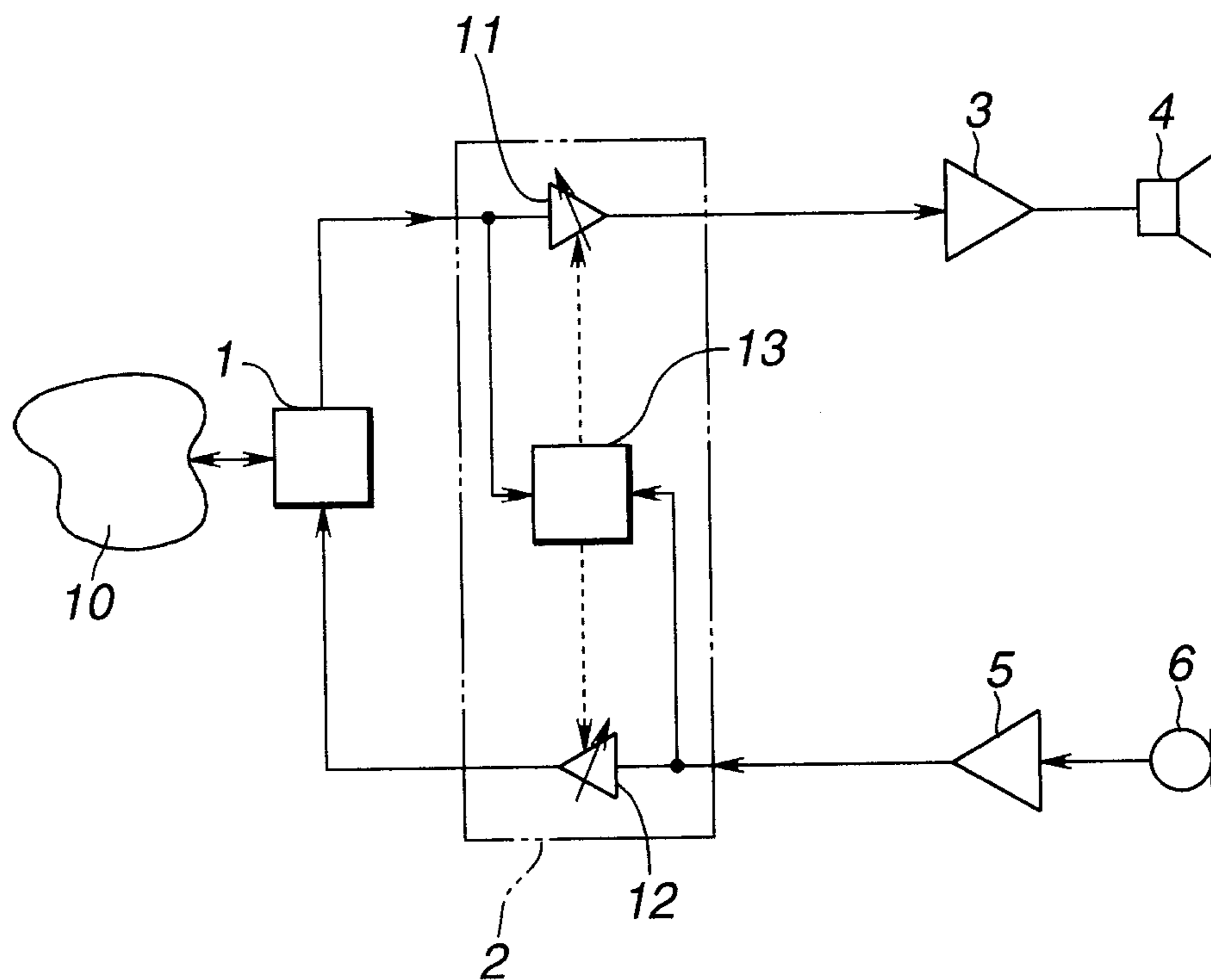
FIG.17 (PRIOR ART)
