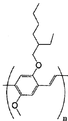
Poly(2-methoxy-5-(2'-ethyl)hexyloxy-p-phenylenevinylene)
