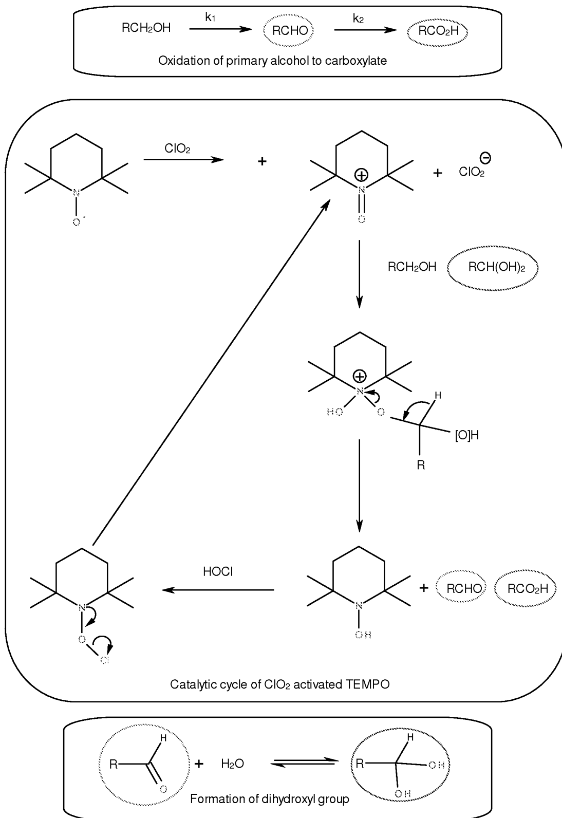
Scheme 2 TEMPO –catalyzed bleach-oxidation of alcohols using chlorine dioxide as activator
