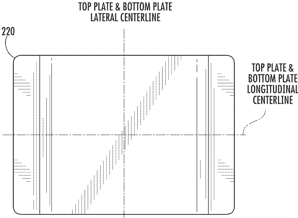
STATIC TOP PLATE
