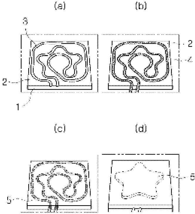
Fig. 3 PRIOR ART
