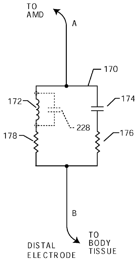
FIG. 20 PRIOR ART
