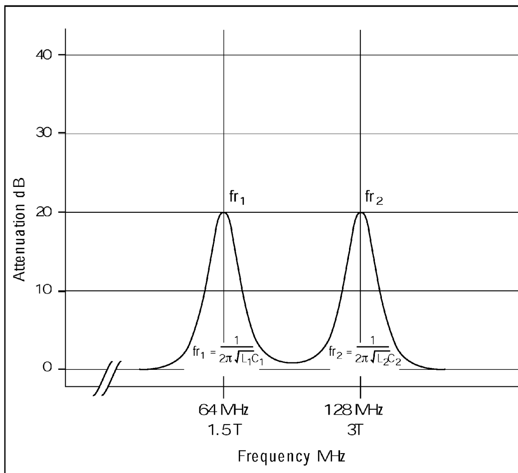
FIG. 24 PRIOR ART
