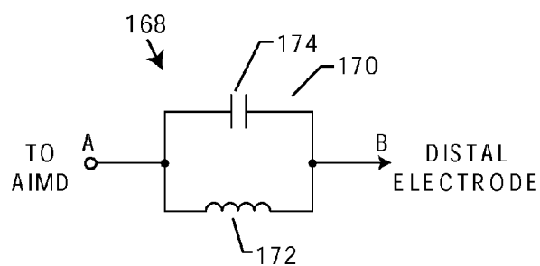
FIG. 16 PRIOR ART
