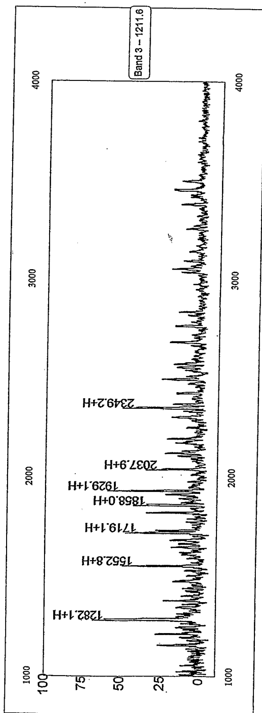
Trypsin Digested Seldi-TOF Spectra FIGURE 2
