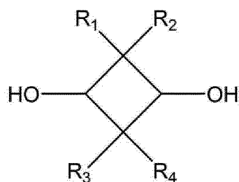
[Chemical Formula 2]
