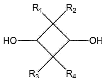
[Chemical Formula 2]
