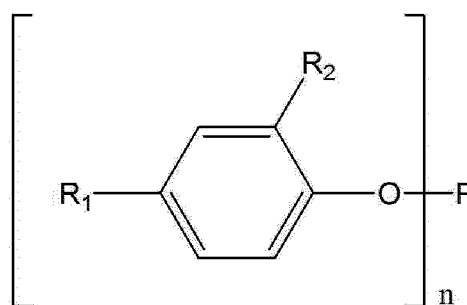
[Chemical Formula 4]
