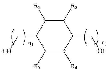
[Chemical Formula 1]
