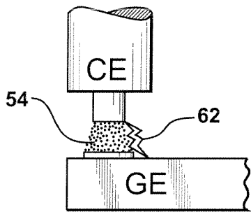
FIG - 4C Prior Art
