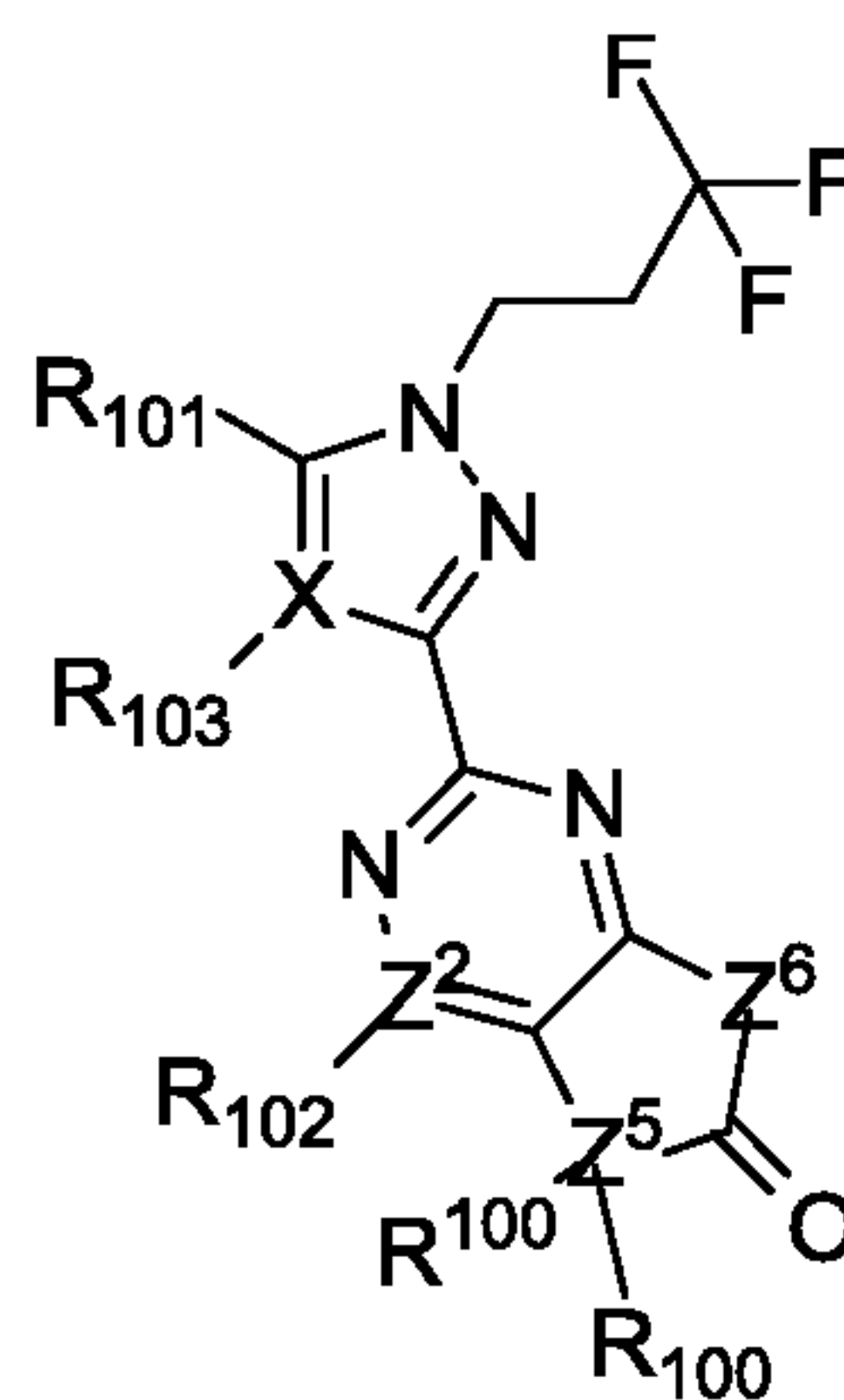
Formula C-2;
