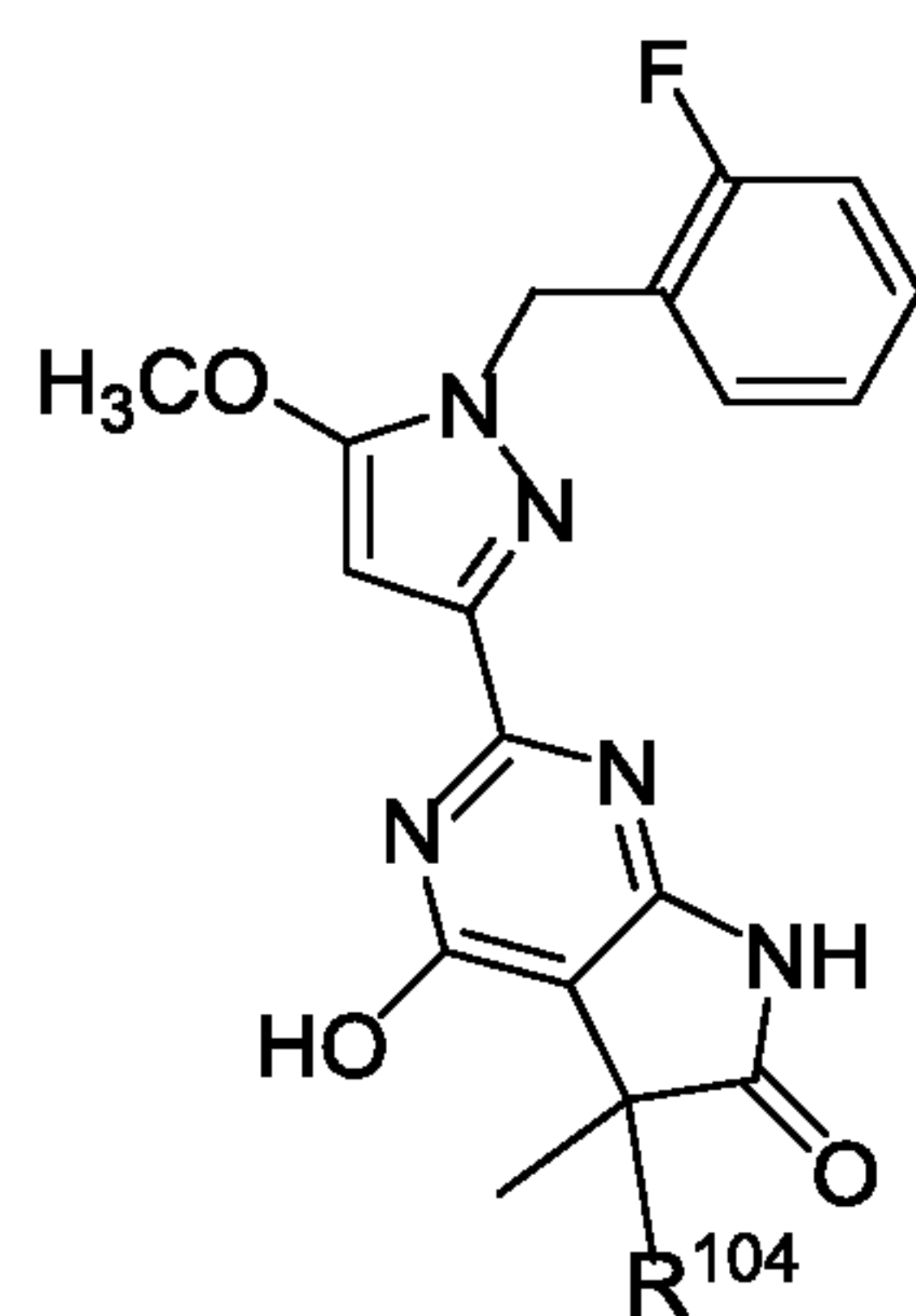
Formula A-2;
