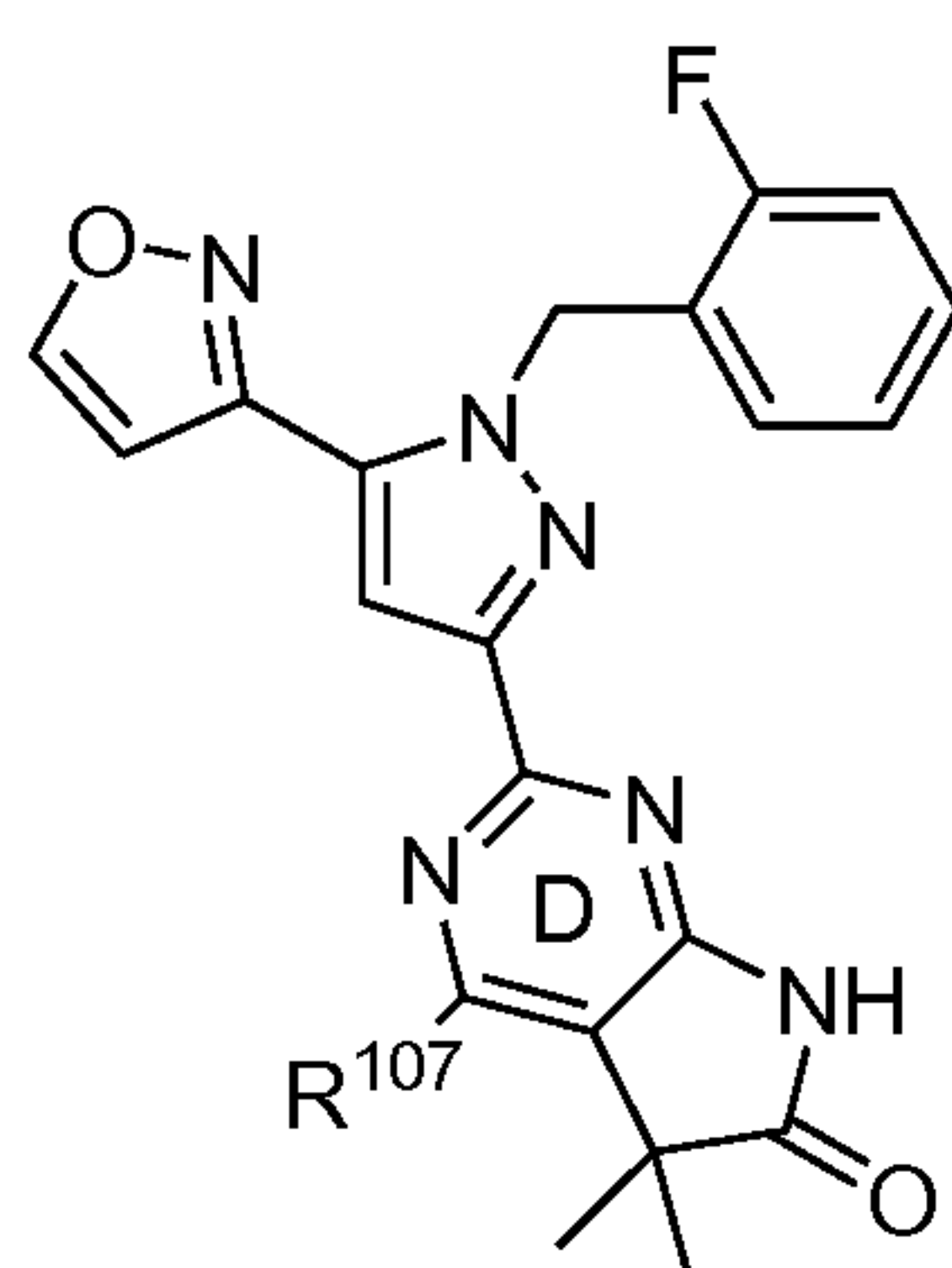
Formula A-4;
