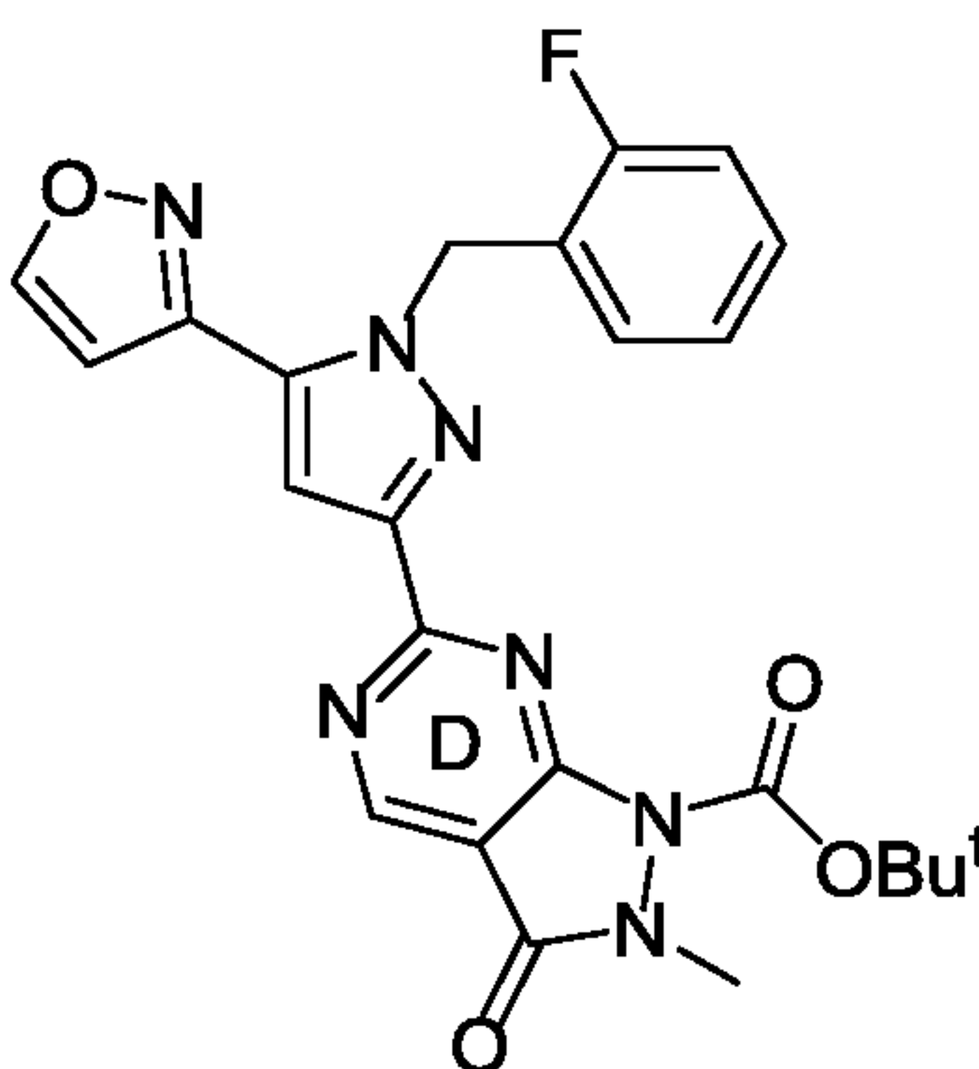
Formula A-8;
