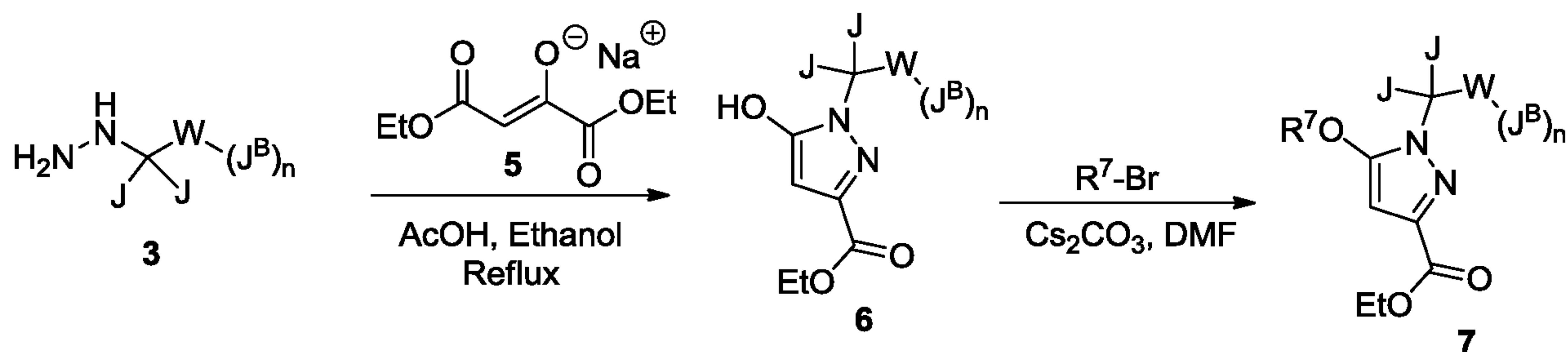
Scheme 2
