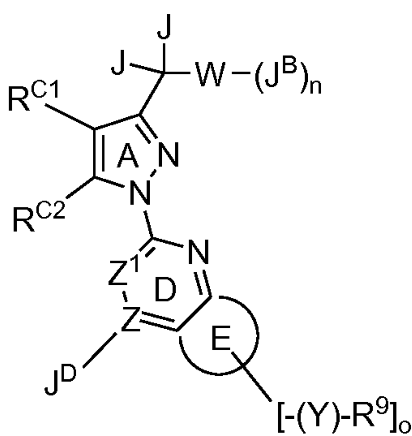
Formula IIB
