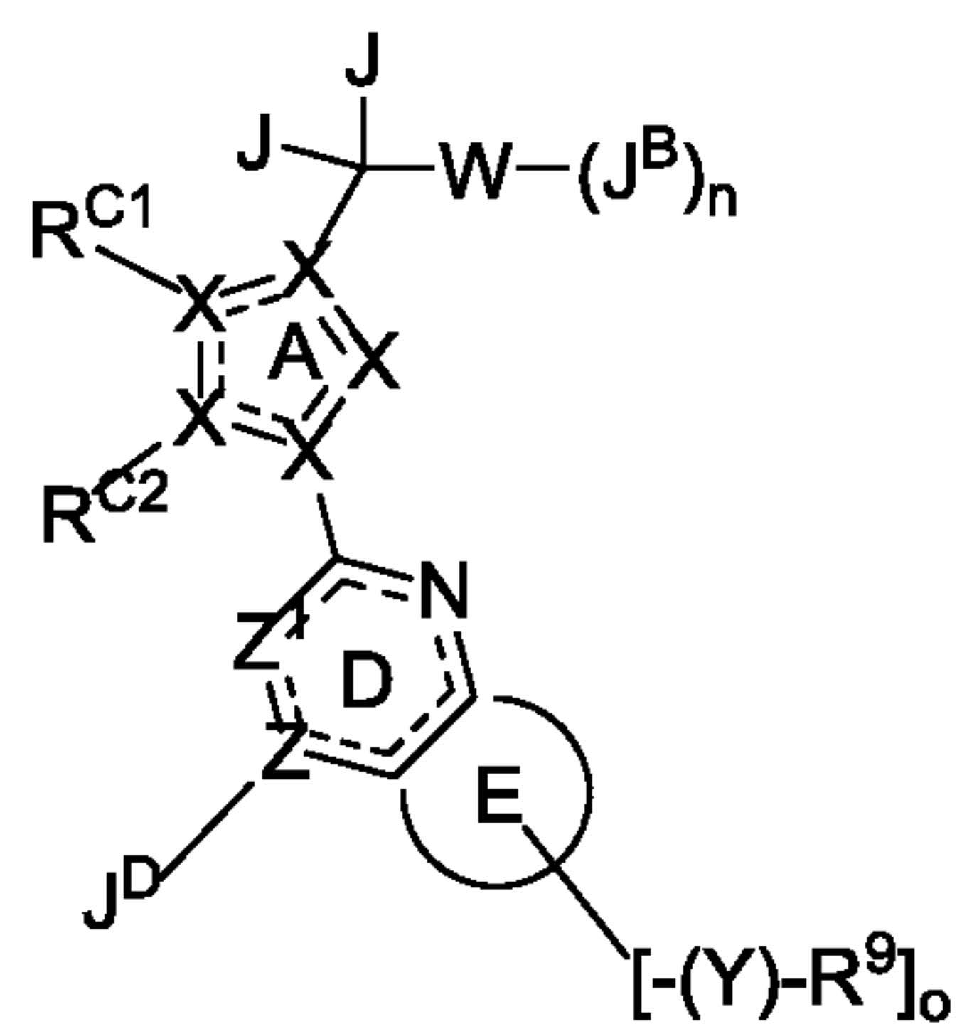
Formula I
