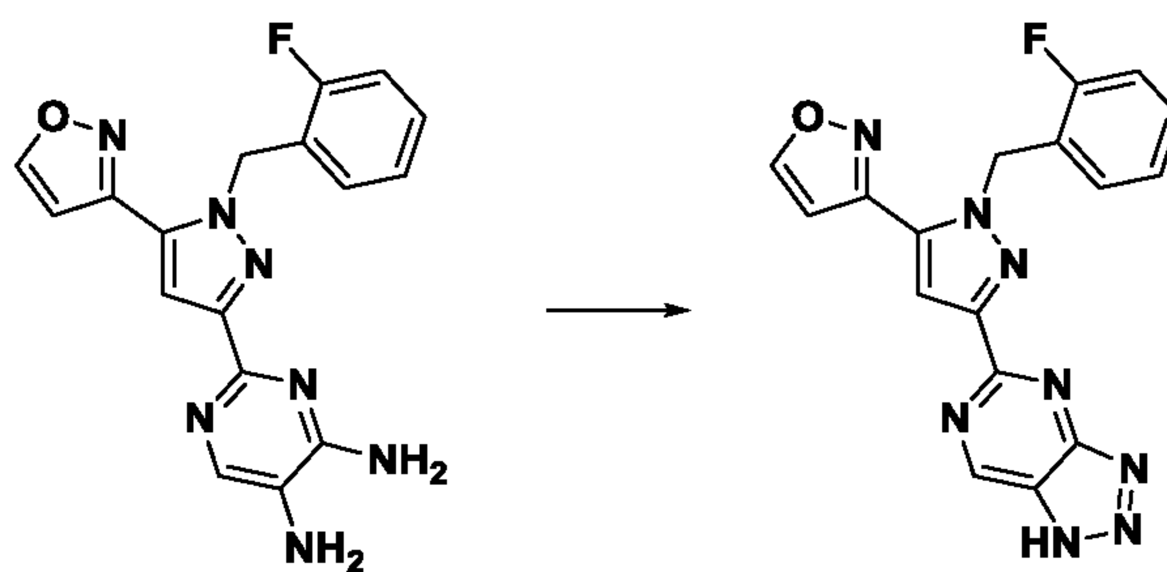
Compound I-15
