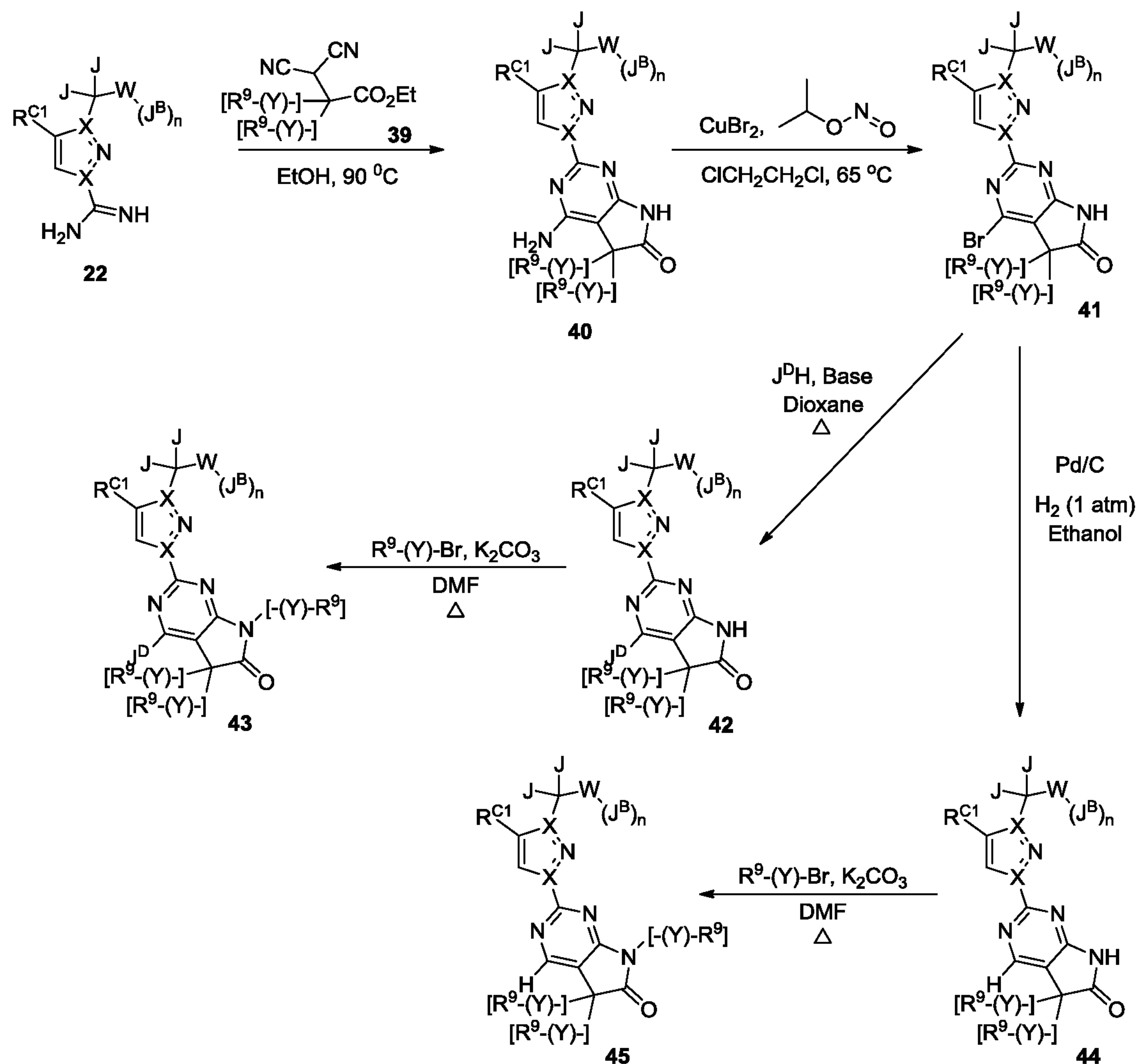
Scheme 7
