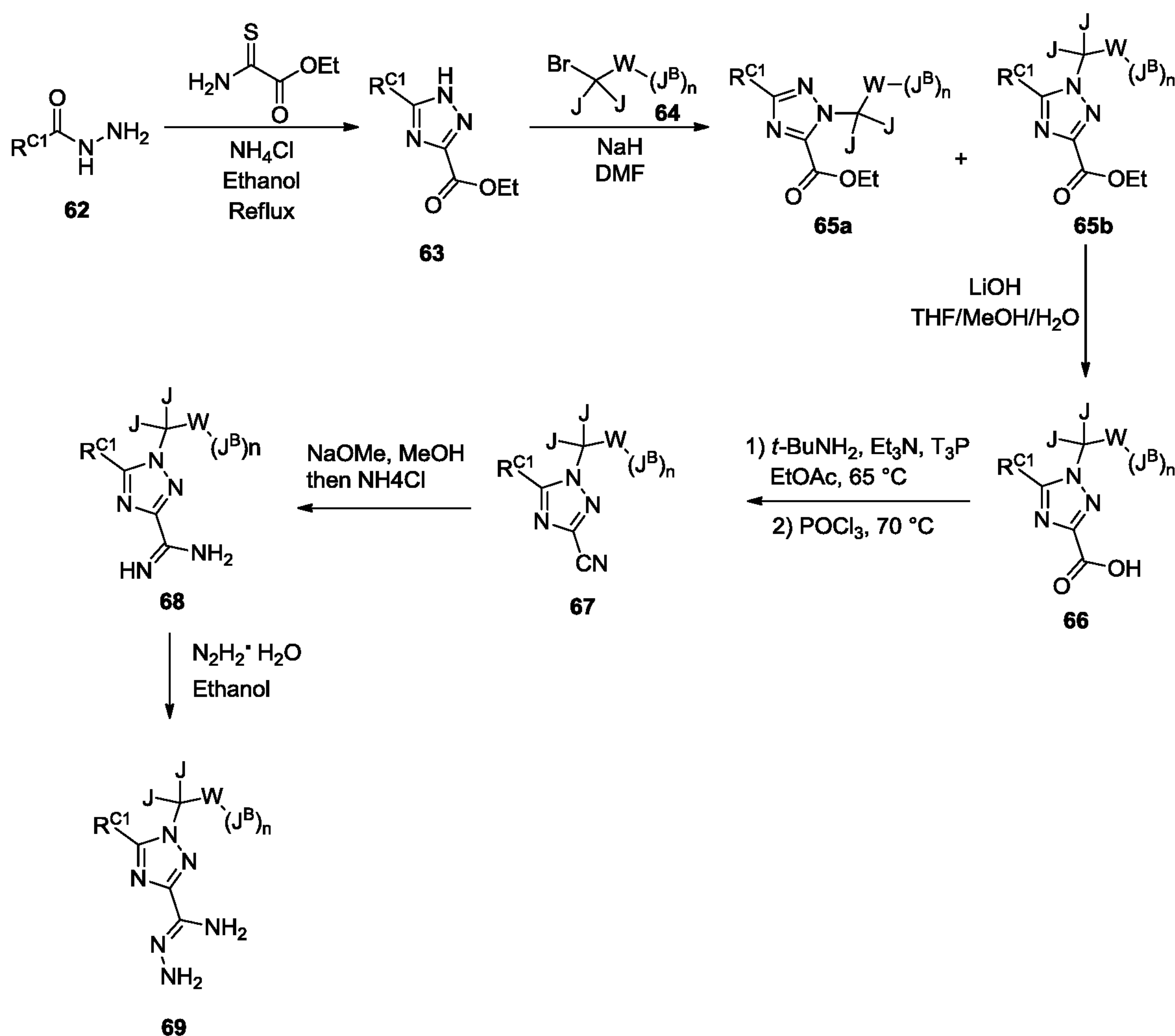
Scheme 12
