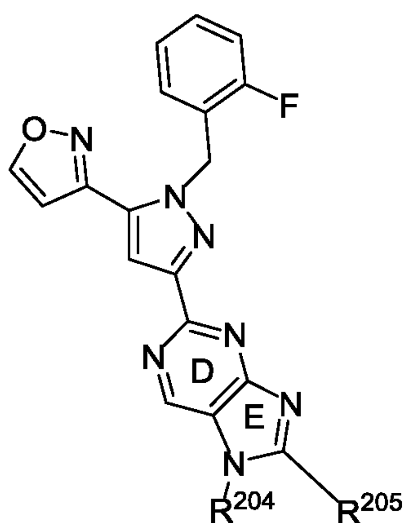
Formula B-2;
