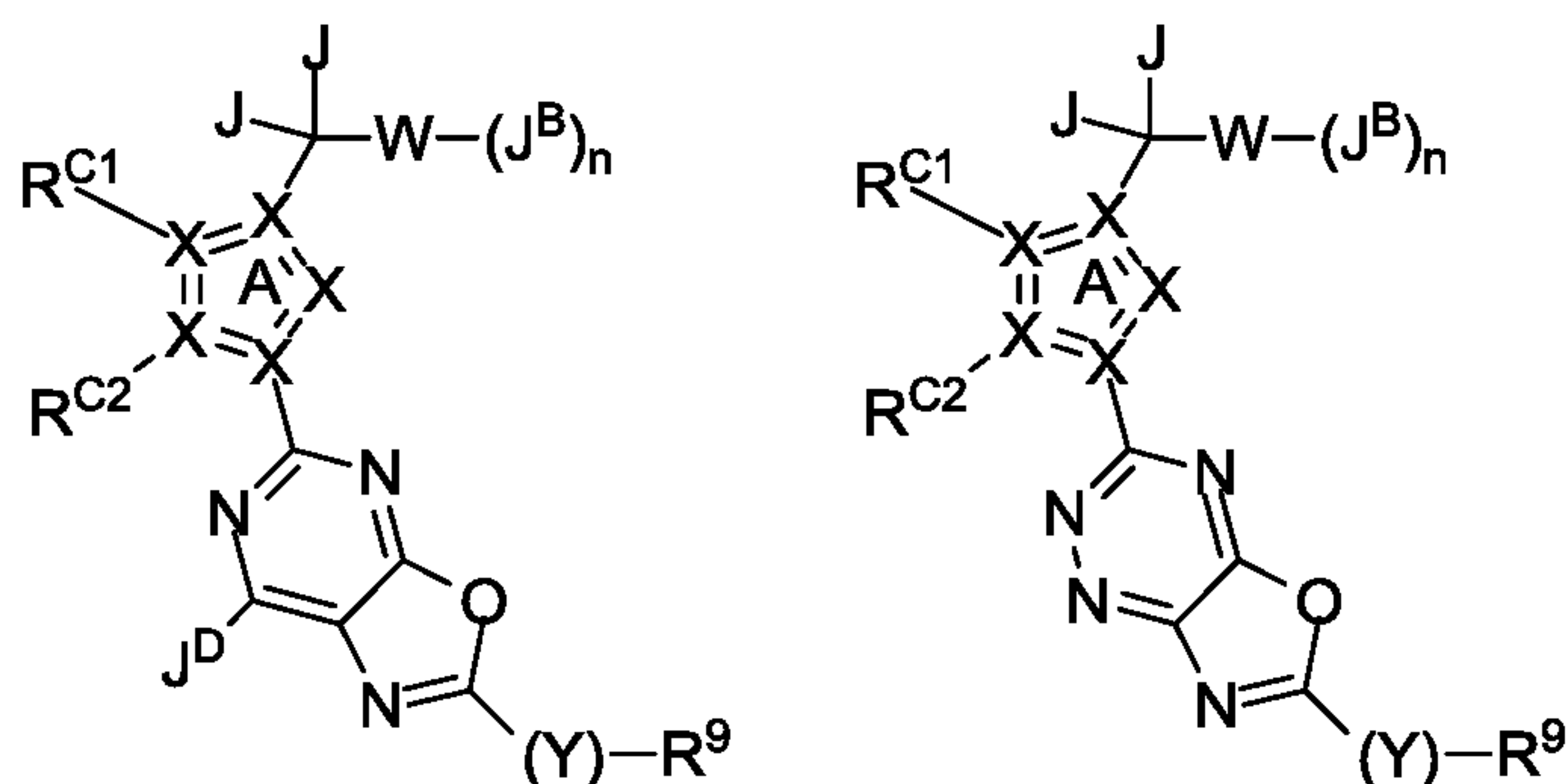
Formula I-p
