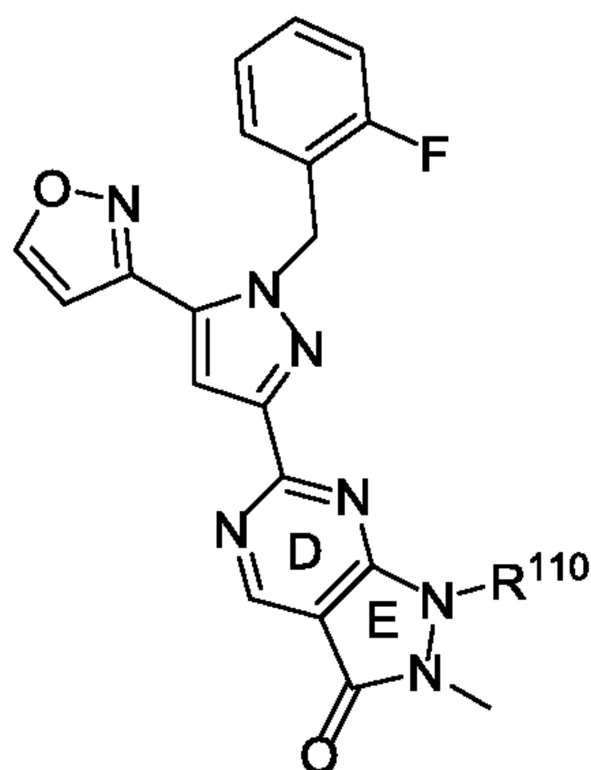
Formula B-4;
