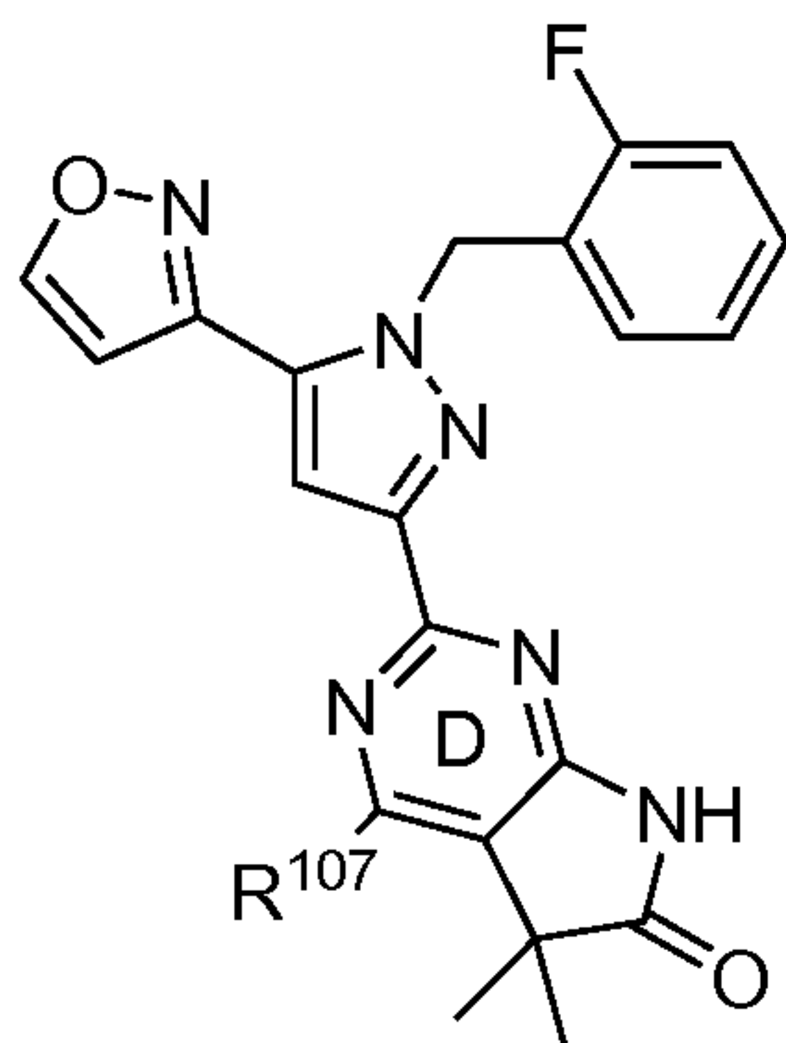
Formula A-4;
