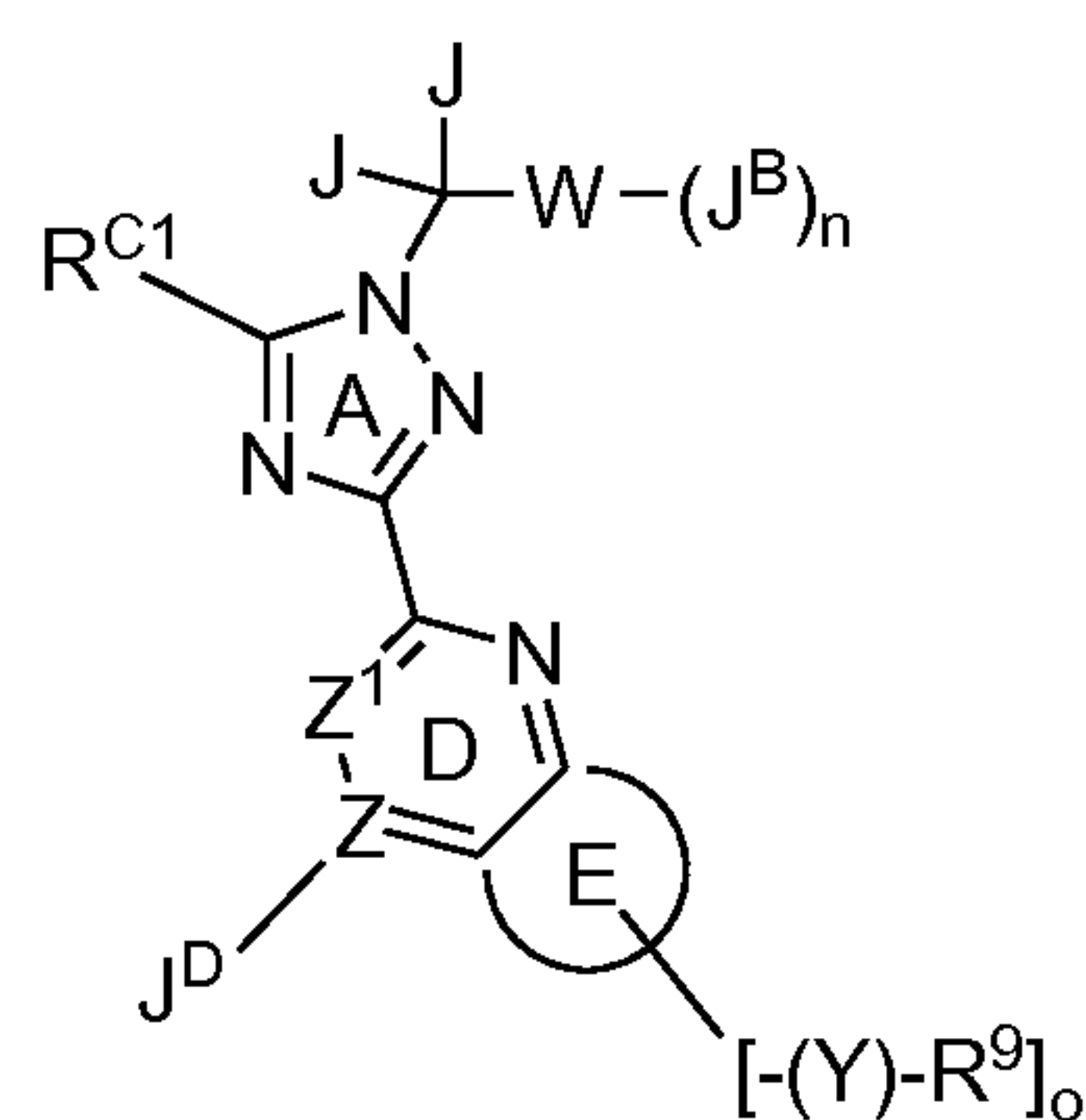
Formula IIC
