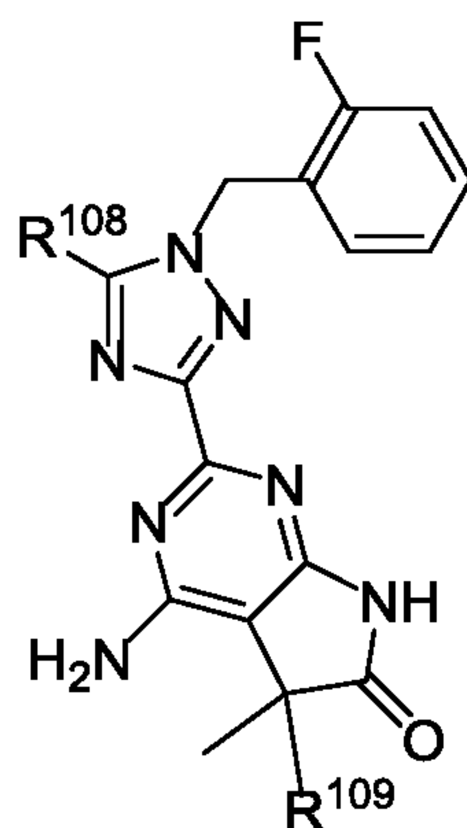
Formula A-6;
