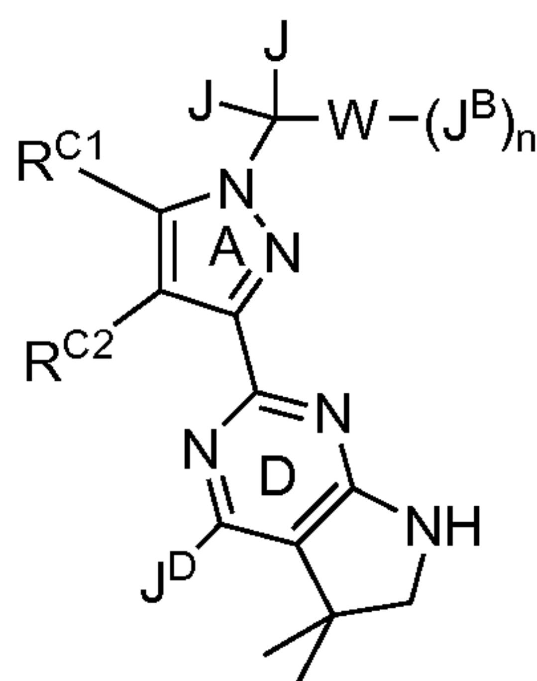
Formula I'''
