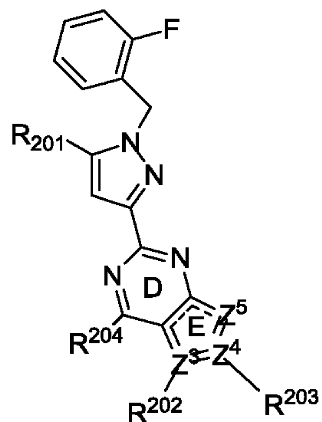
Formula B
