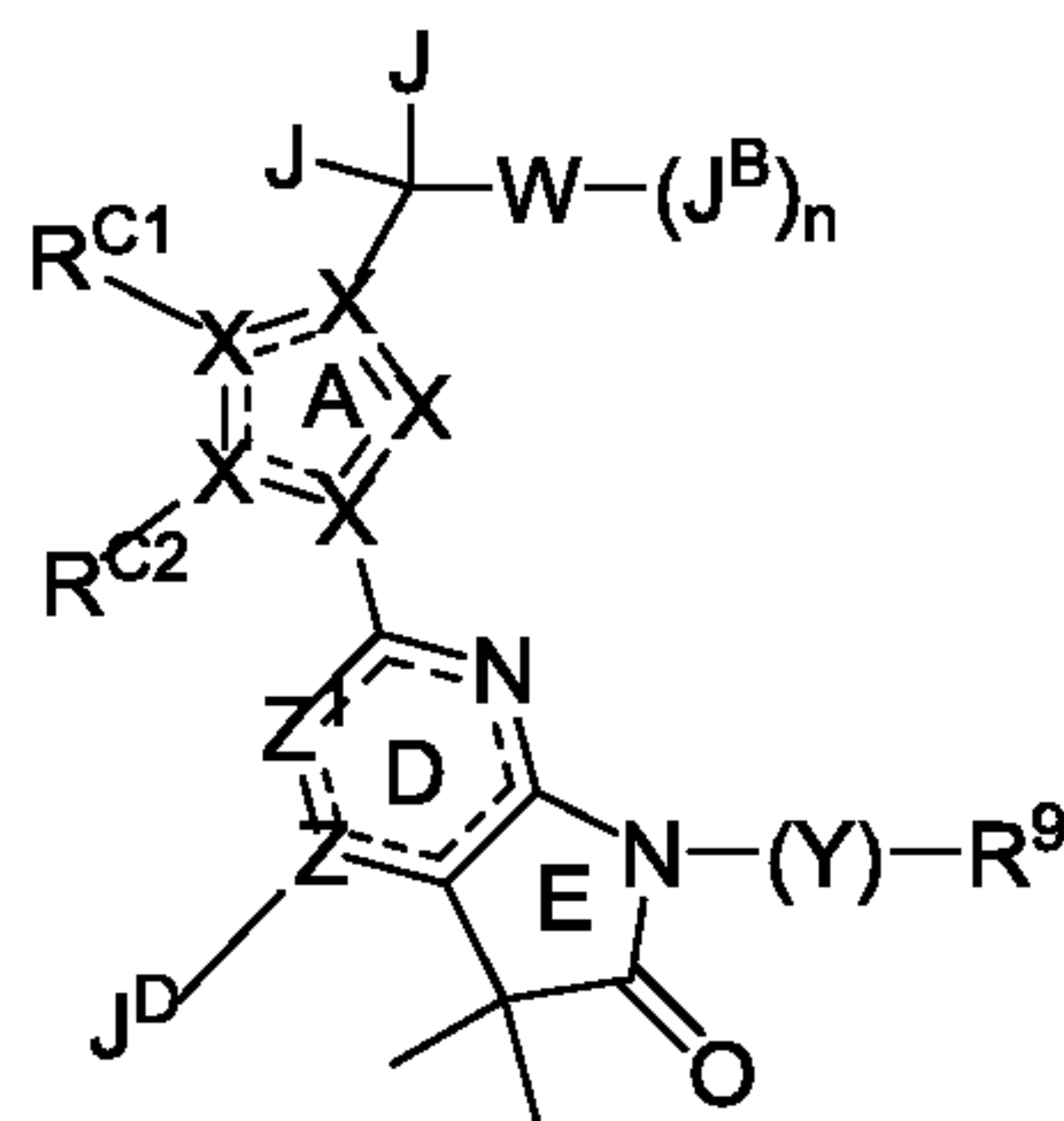
Formula I'C
