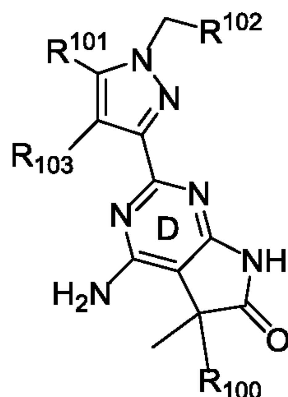
Formula A-1;
