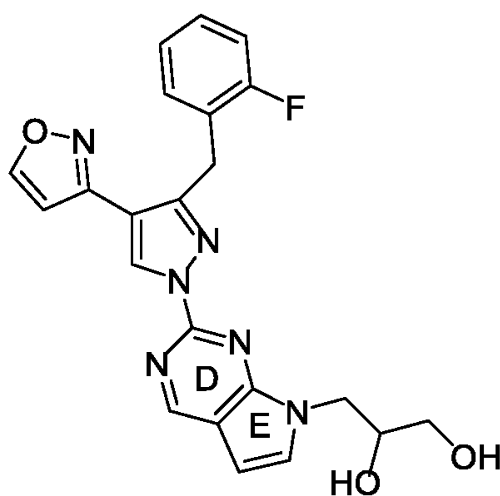
Formula B-5;
