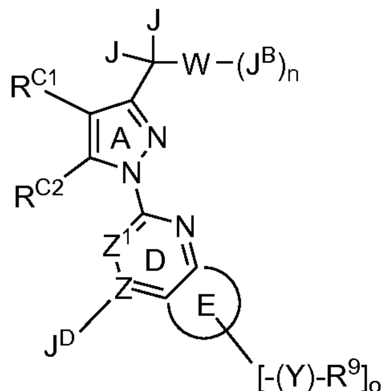
Formula IIB
