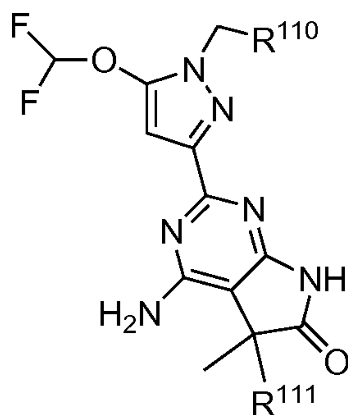
Formula A-7;
