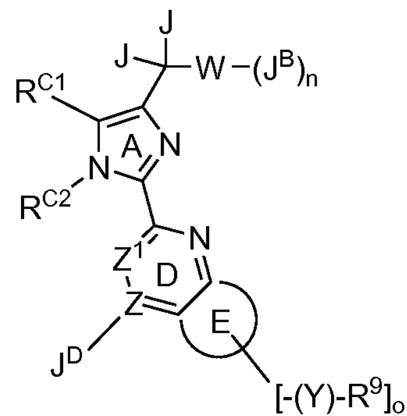
Formula IIF
