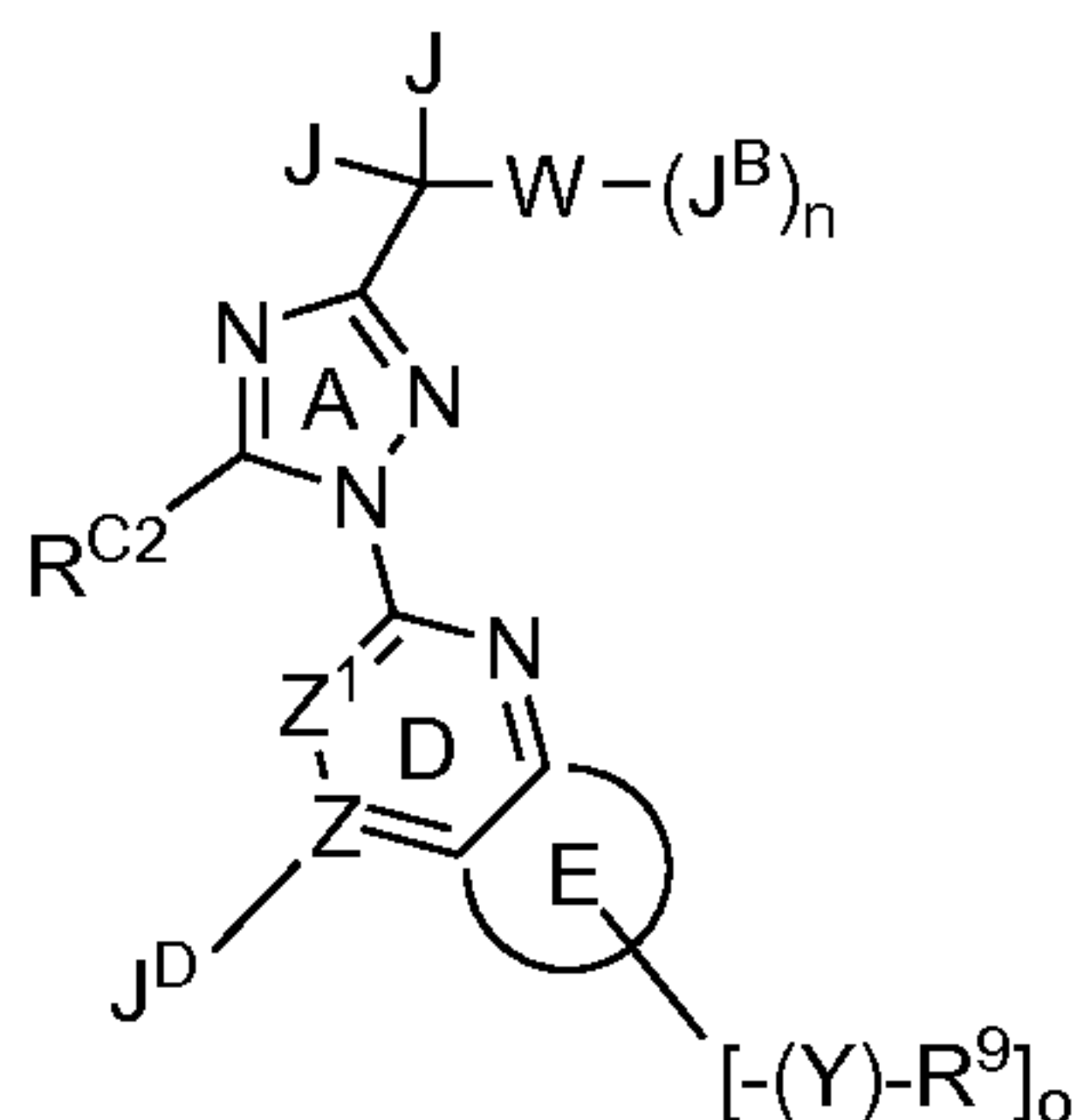
Formula IID
