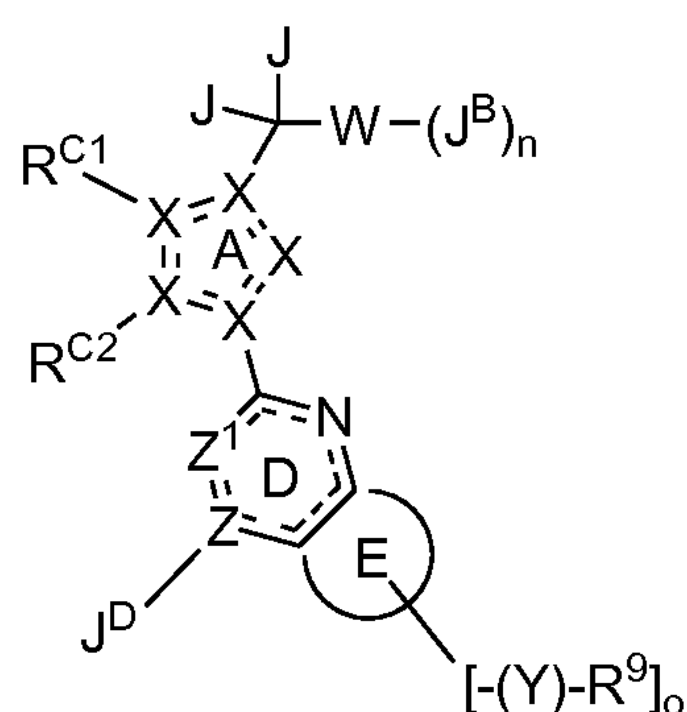
Formula I
