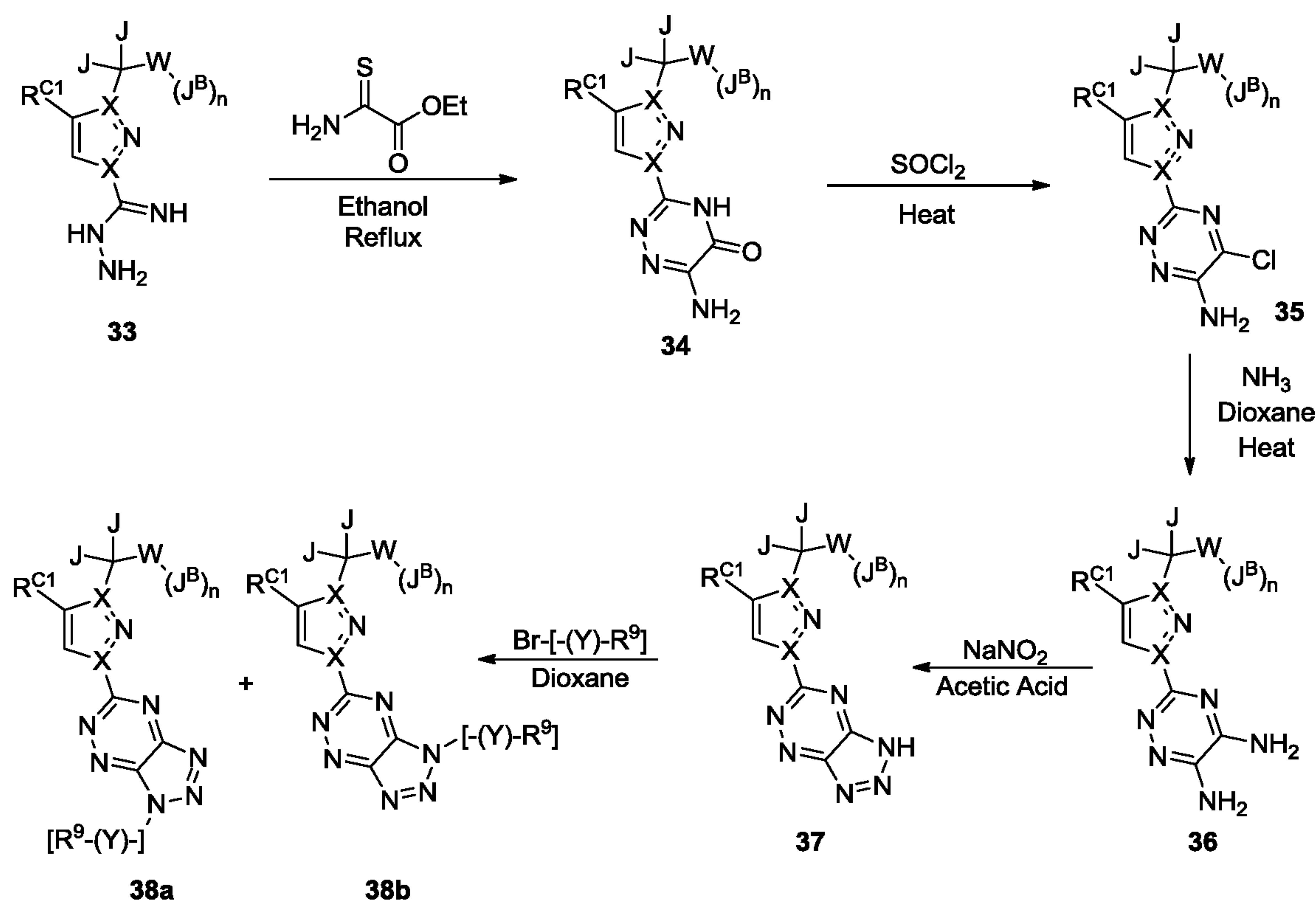
Scheme 6
