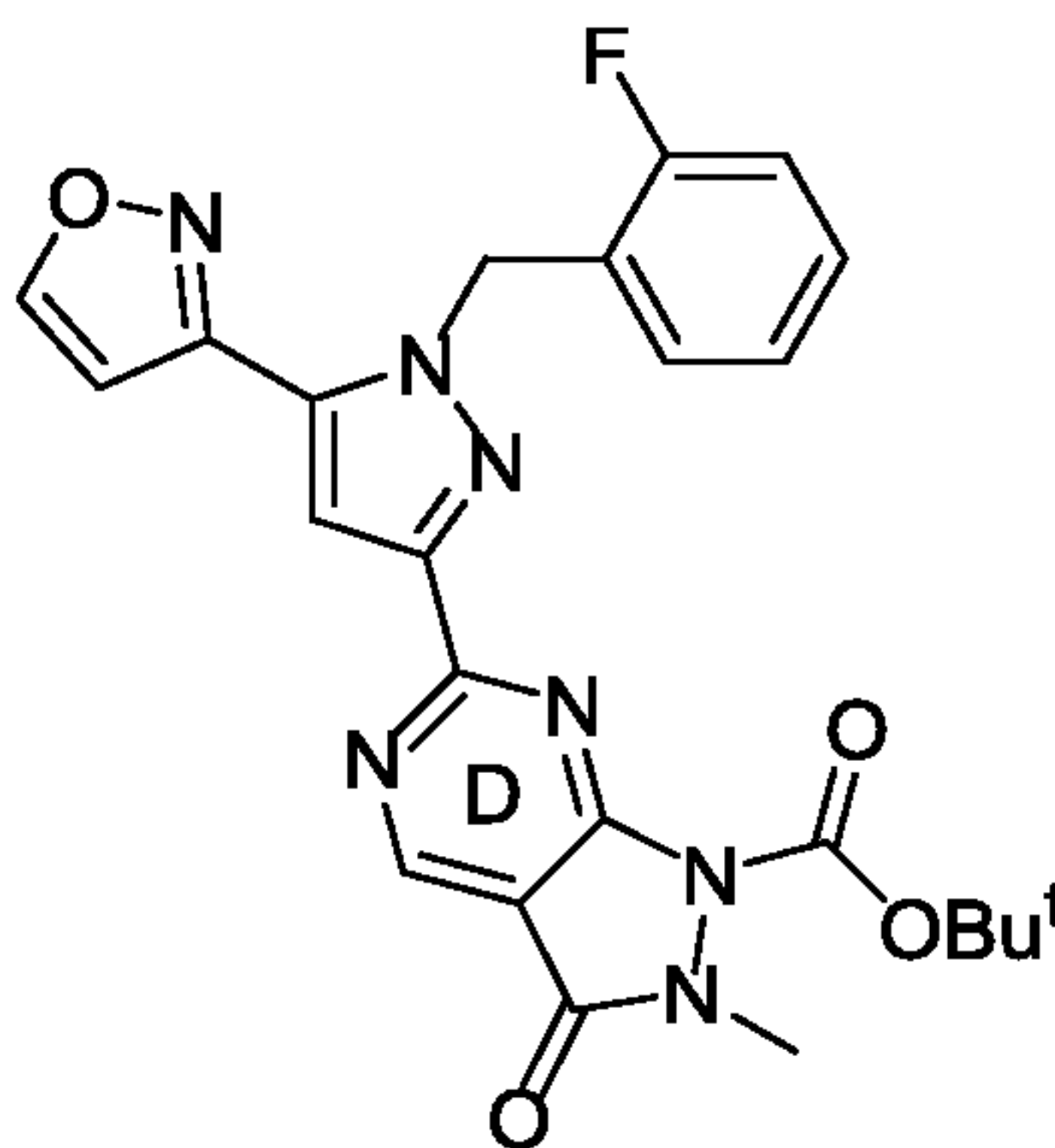
Formula A-8;
