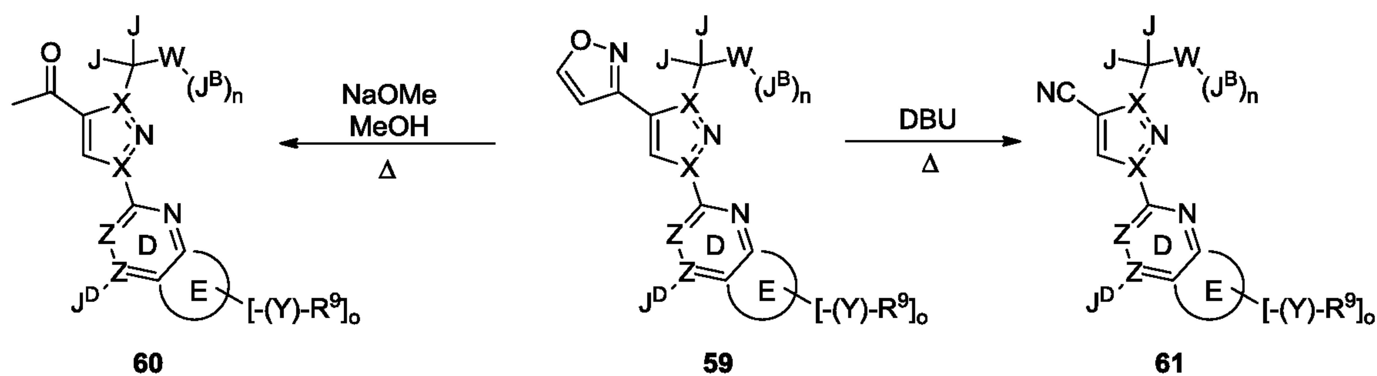
Scheme 11
