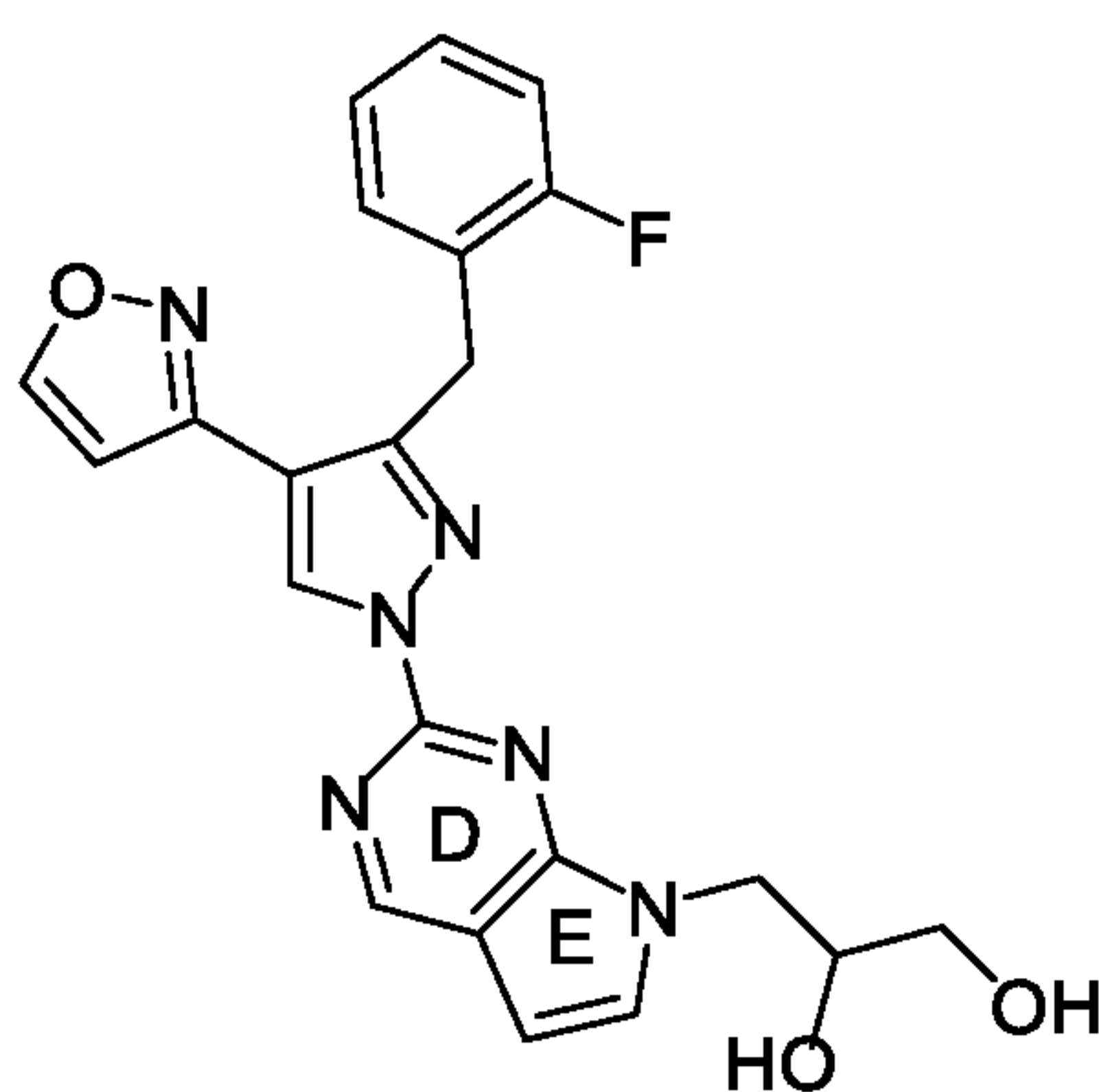
Formula B-5;
