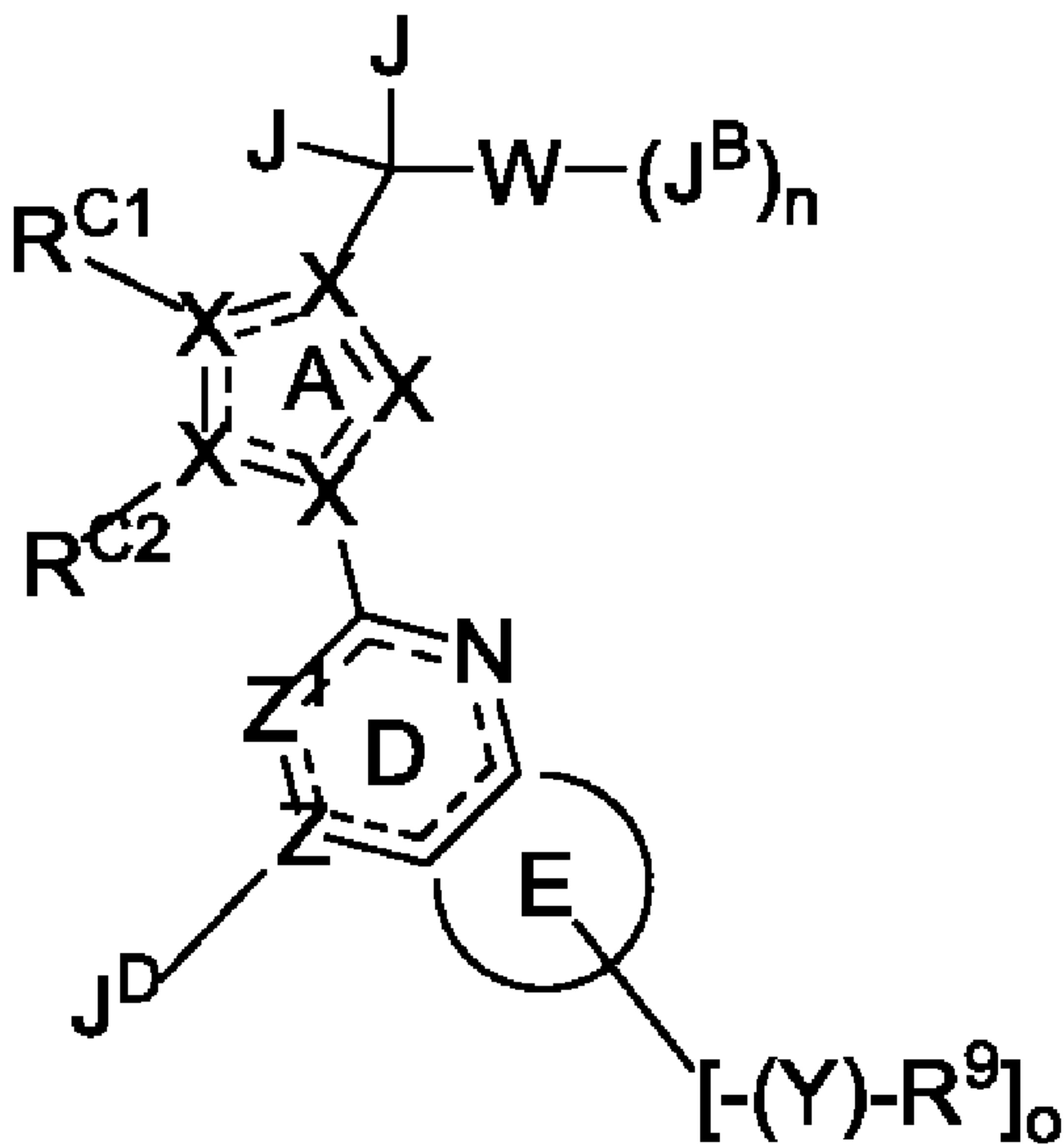
Formula I'
