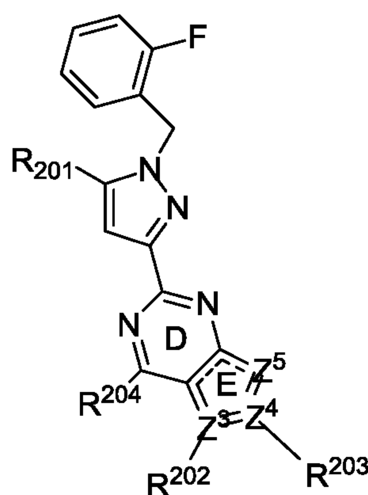
Formula B
