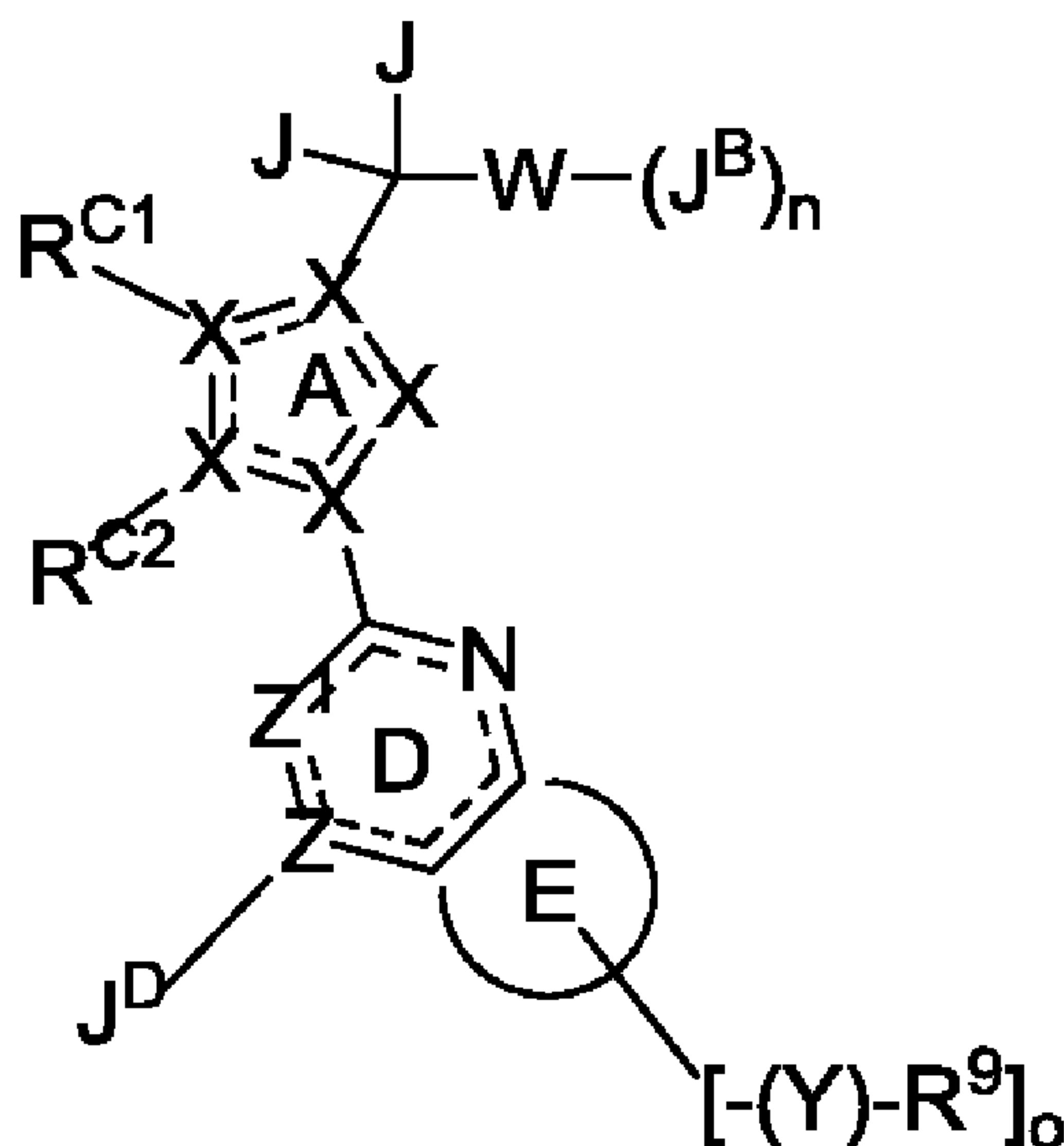
Formula I'
