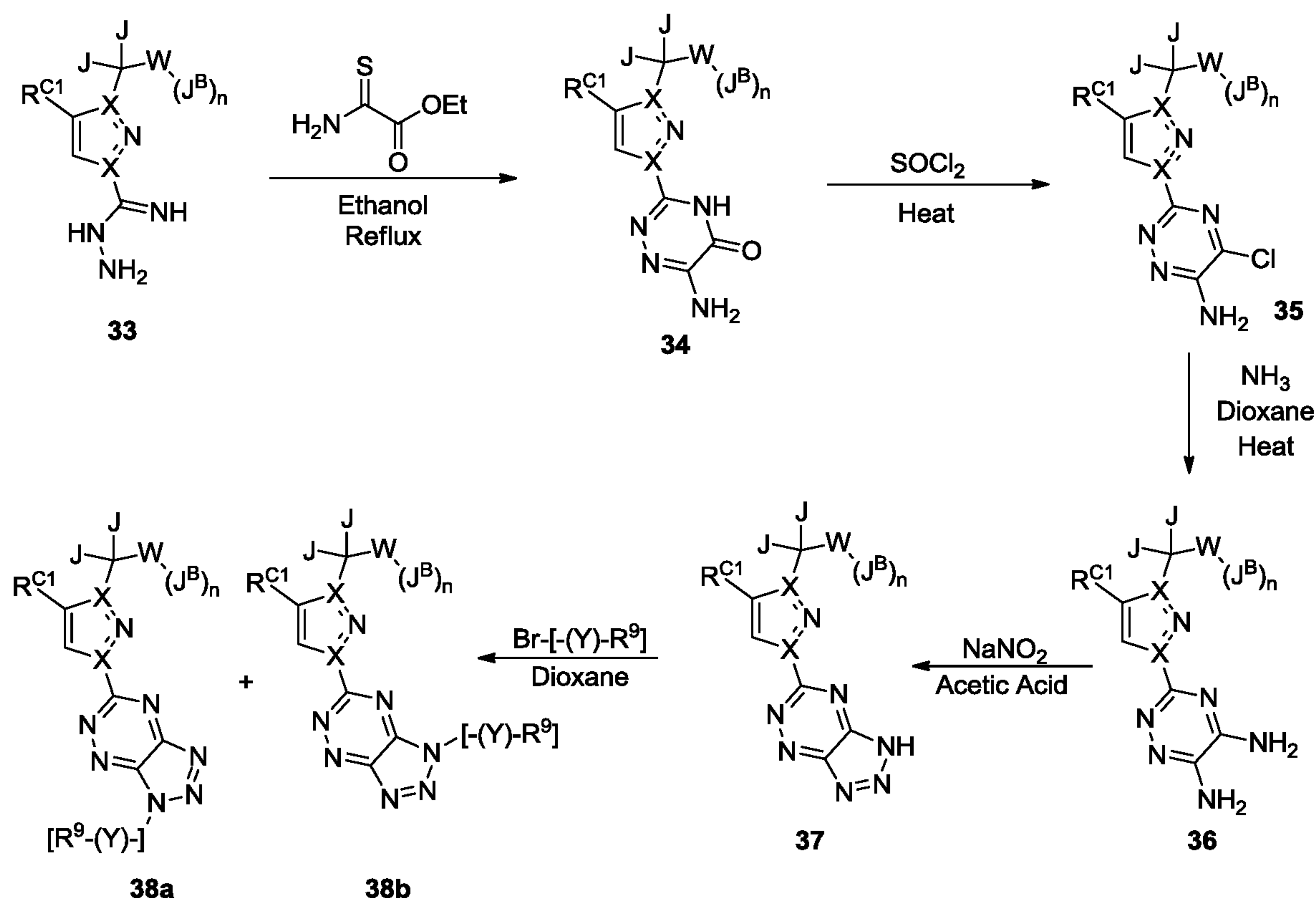
Scheme 6
