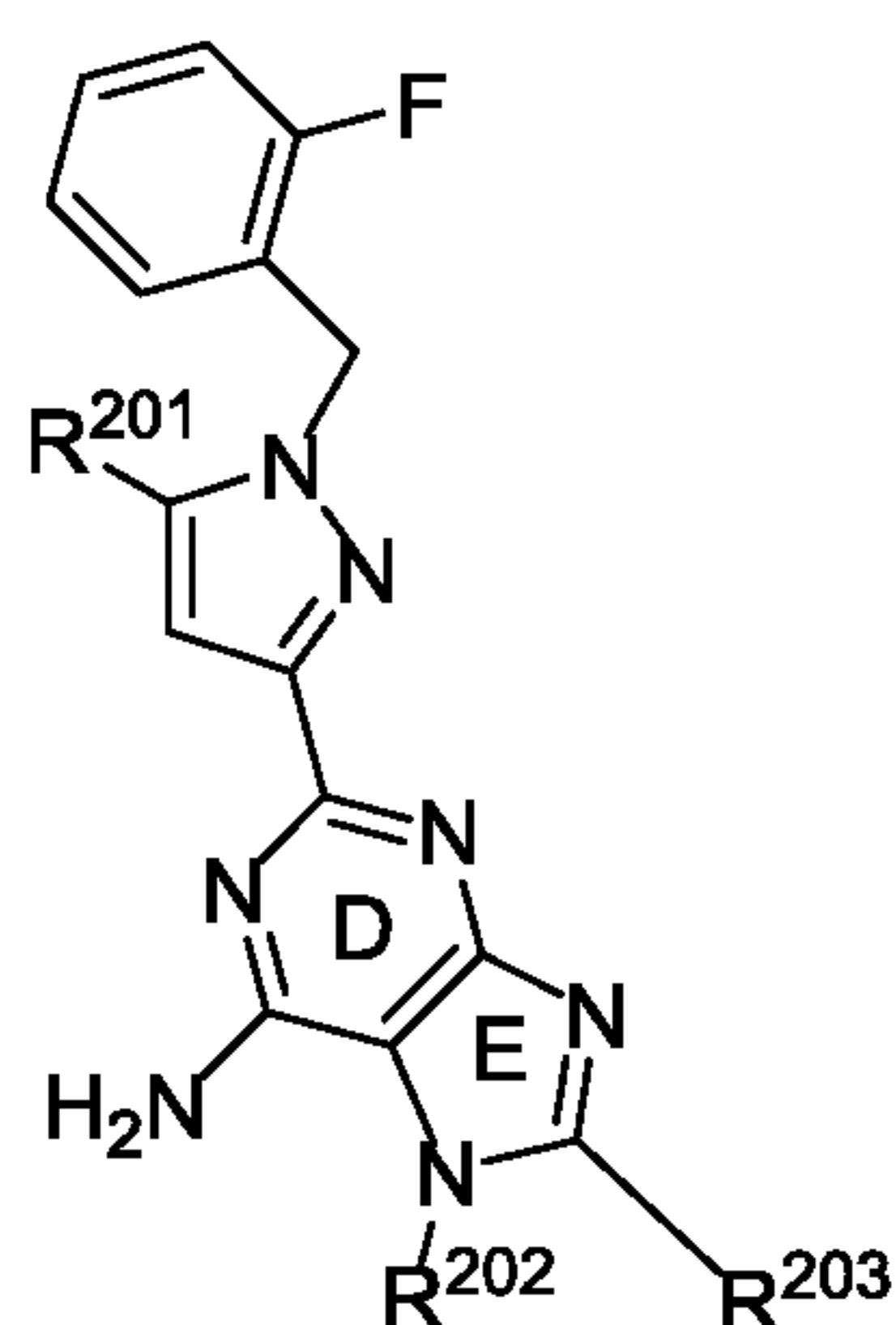
Formula B-1;
