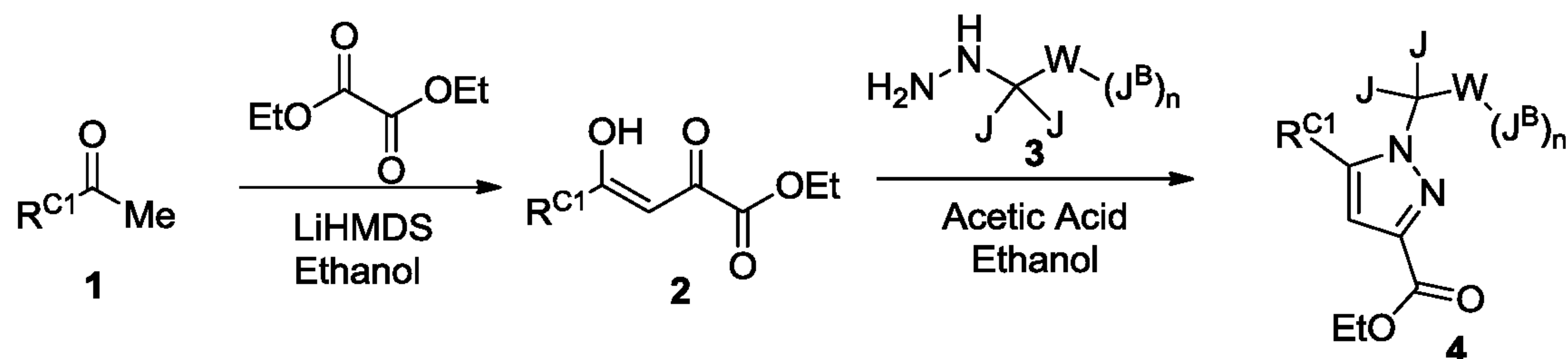
Scheme 1
