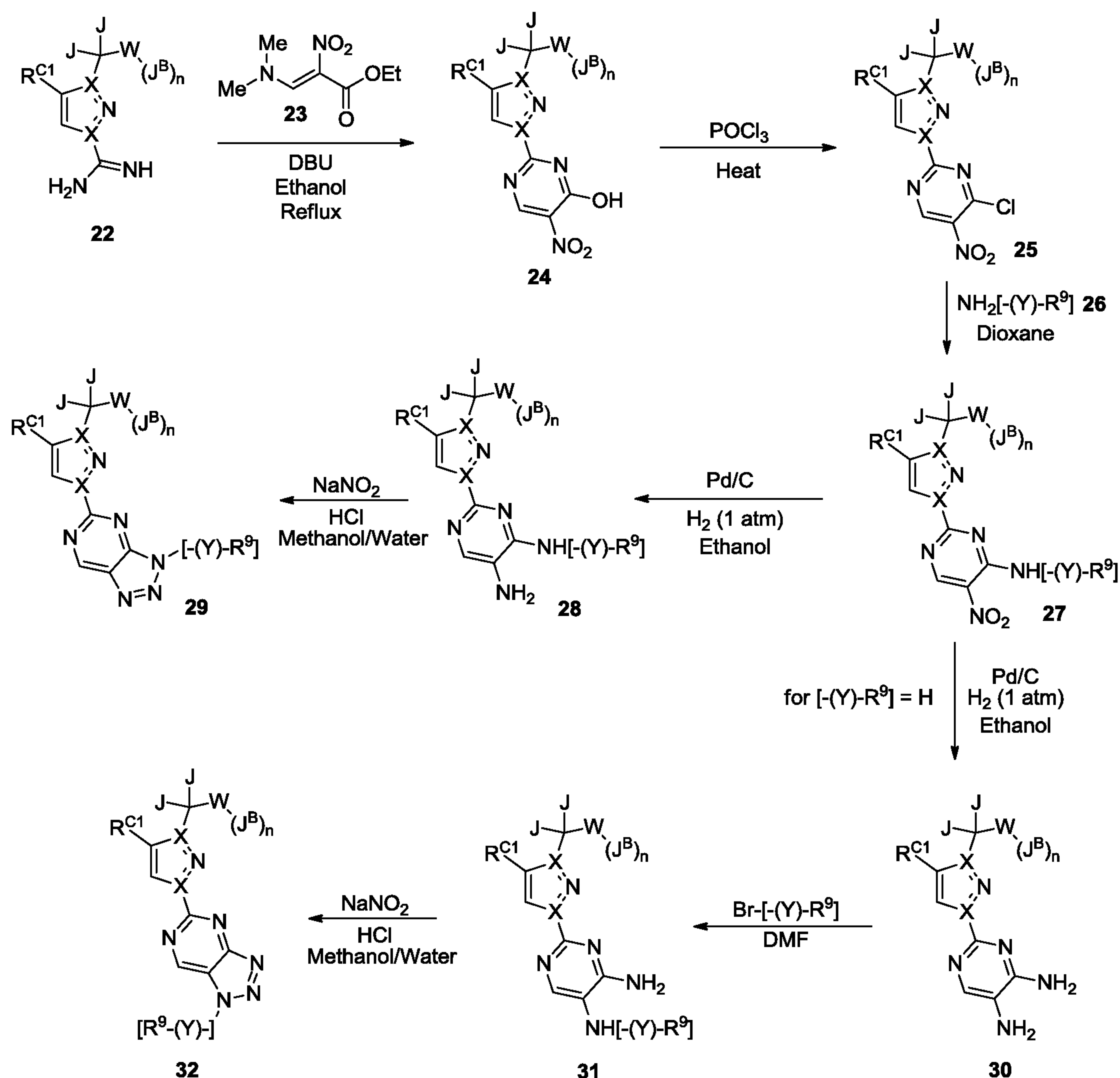
Scheme 5
