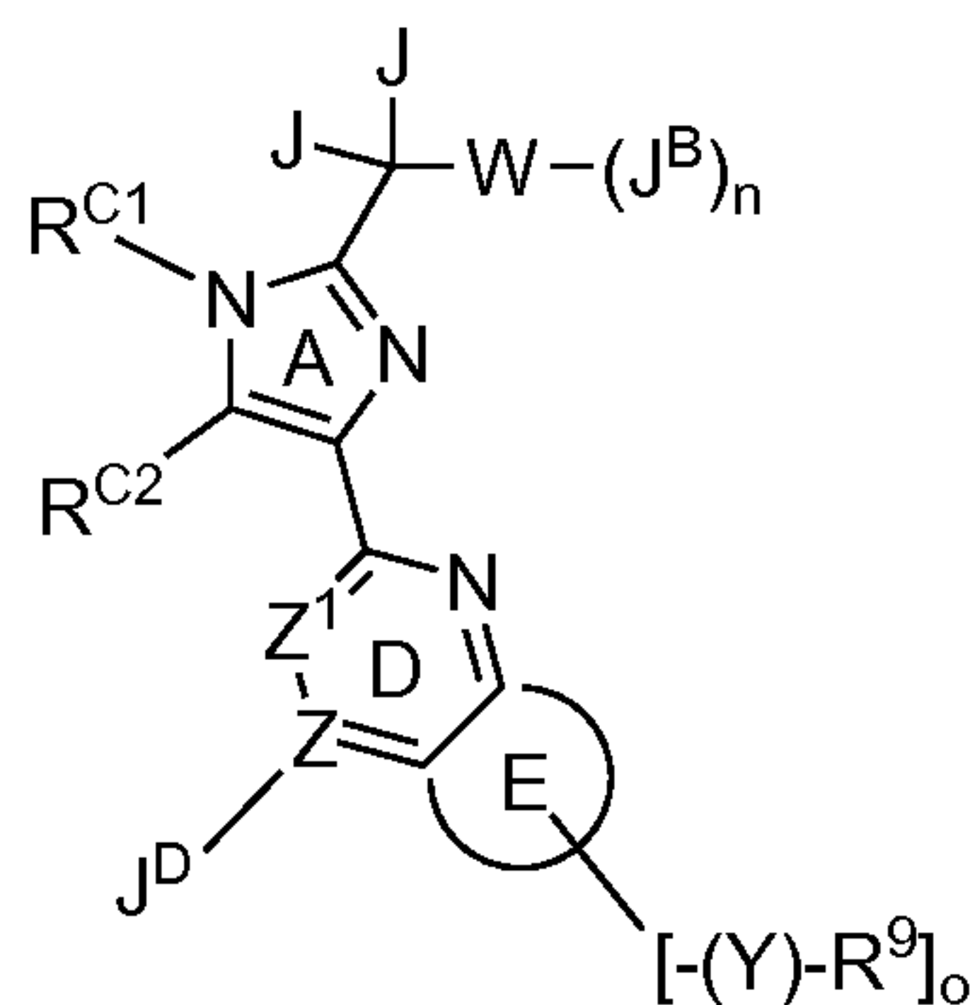
Formula IIE
