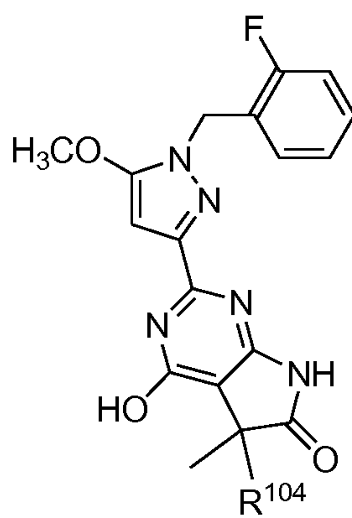
Formula A-2;
