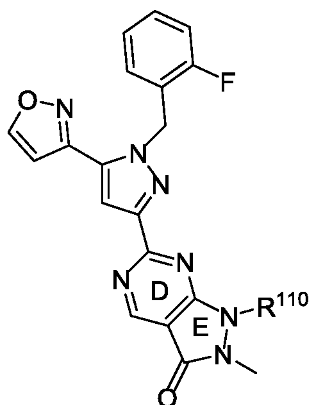
Formula B-4;
