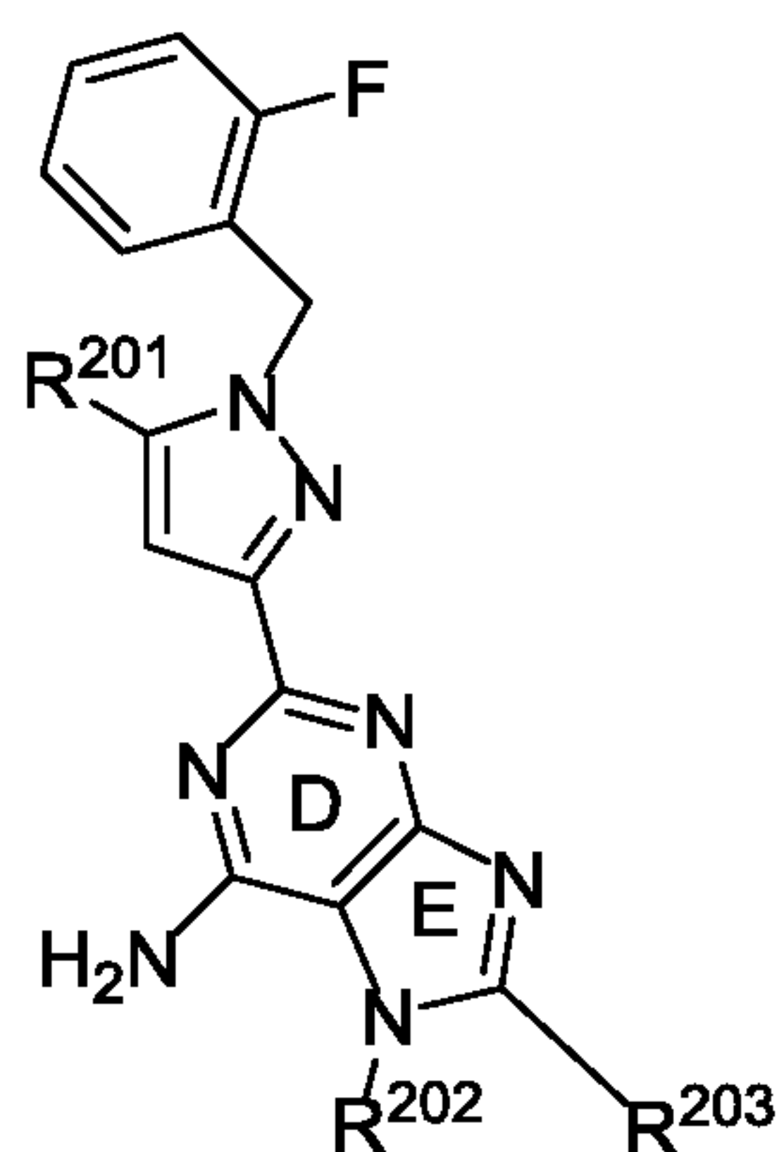
Formula B-1;
