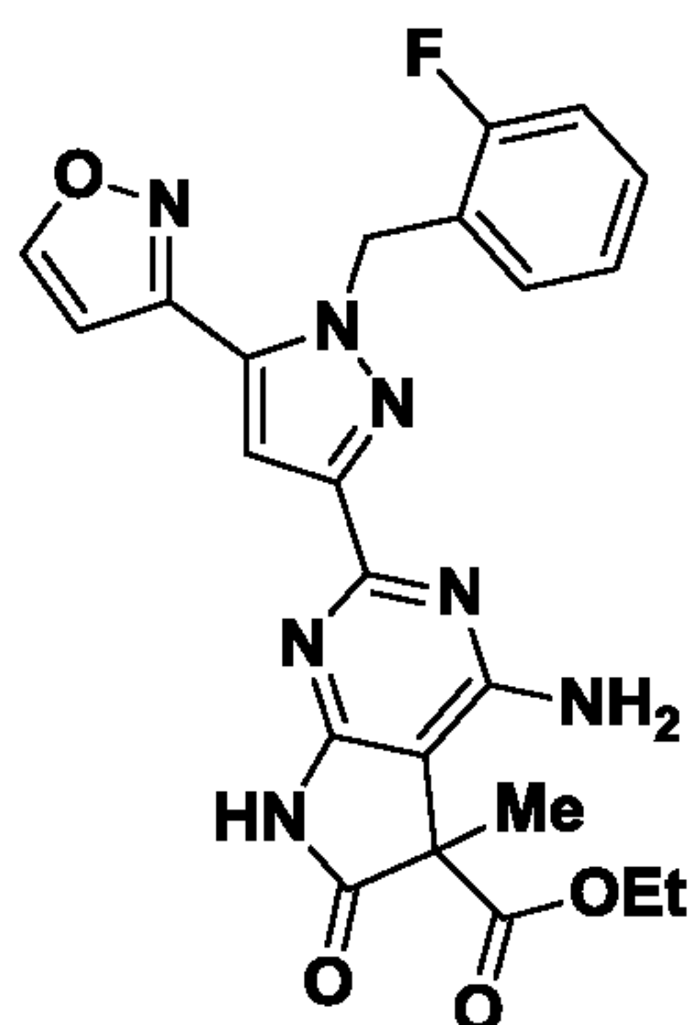
Intermediate-12
