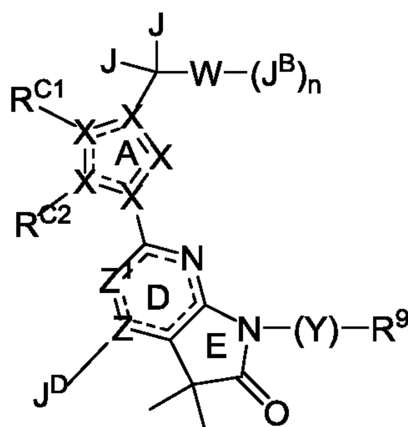
Formula I'C .
