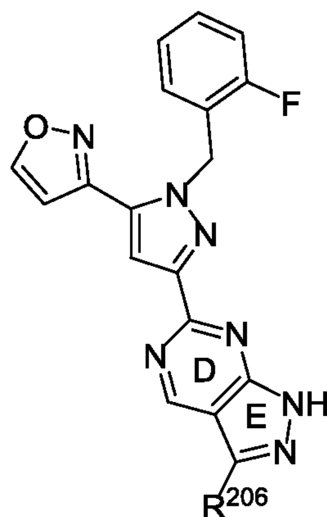
Formula B-3;
