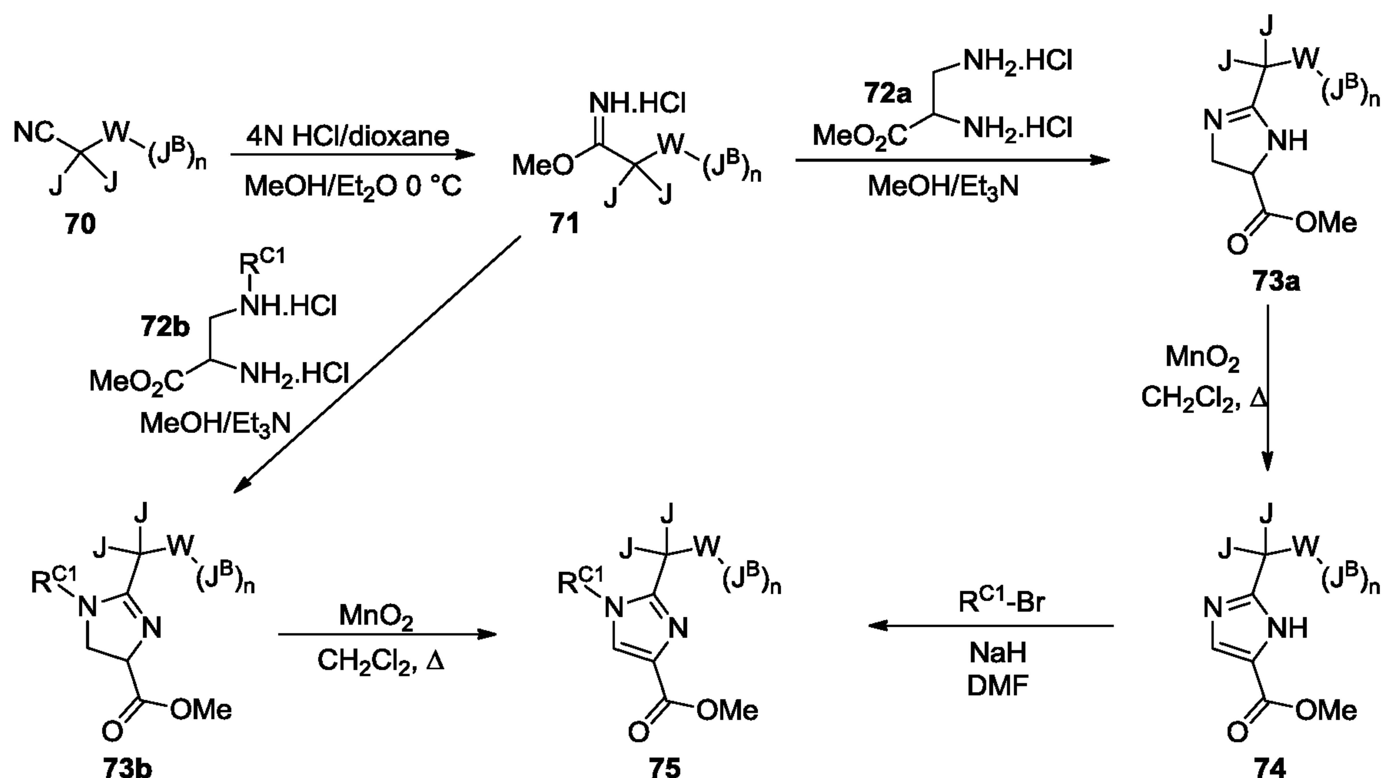
Scheme 13
