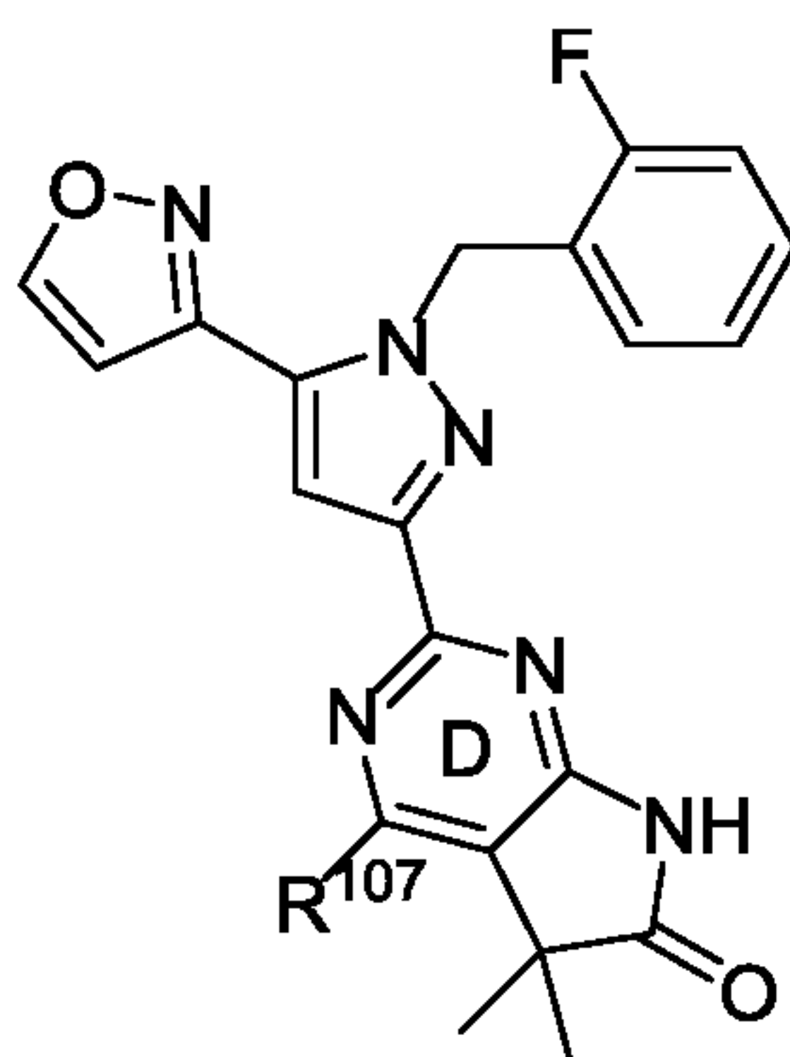
Formula A-4;
