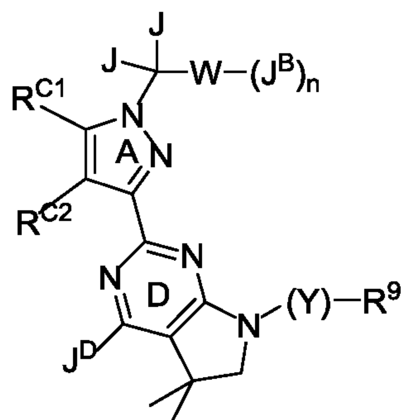
Formula I''
