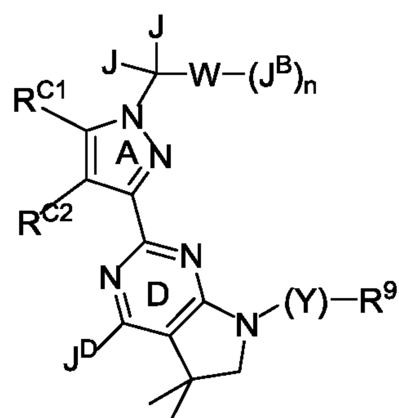
Formula I''
