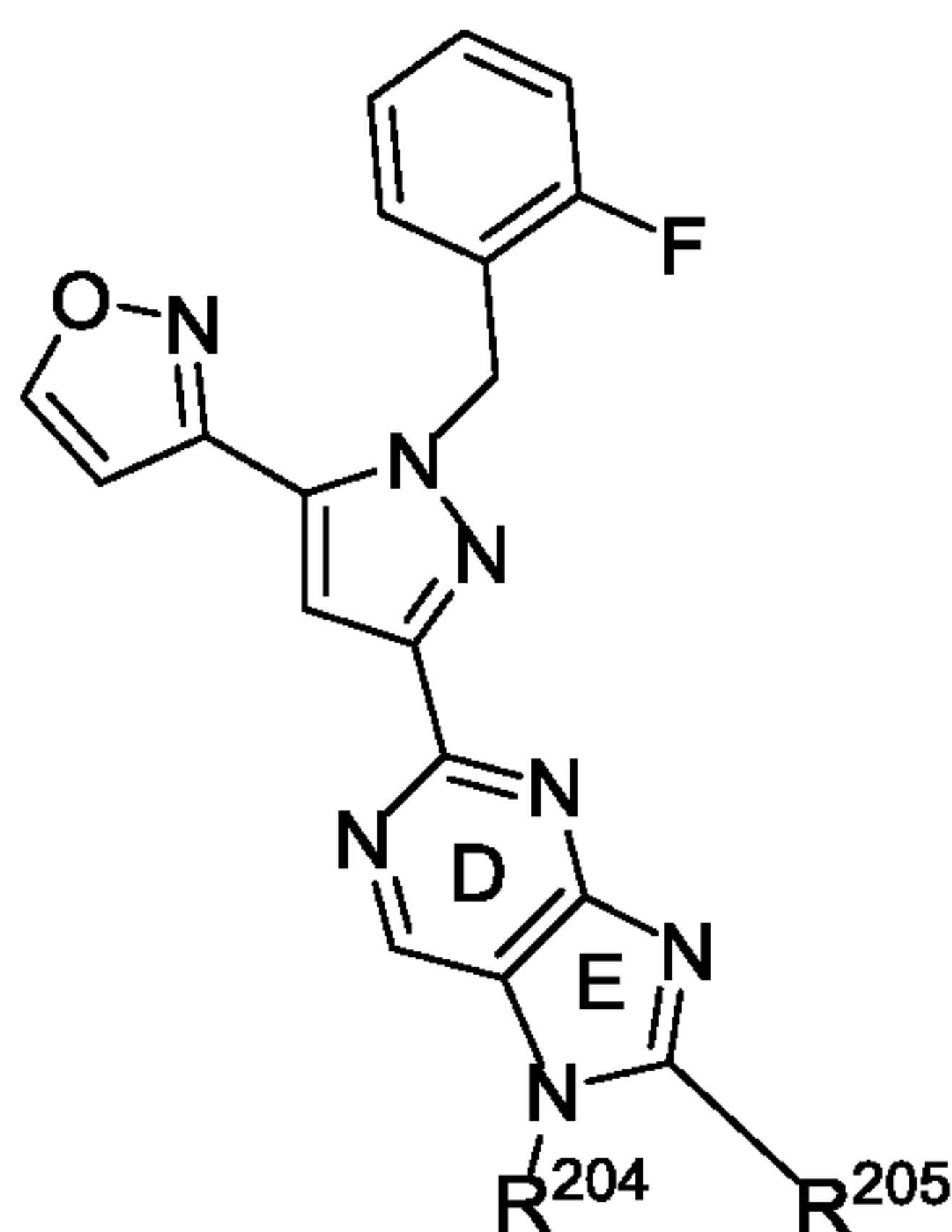
Formula B-2;
