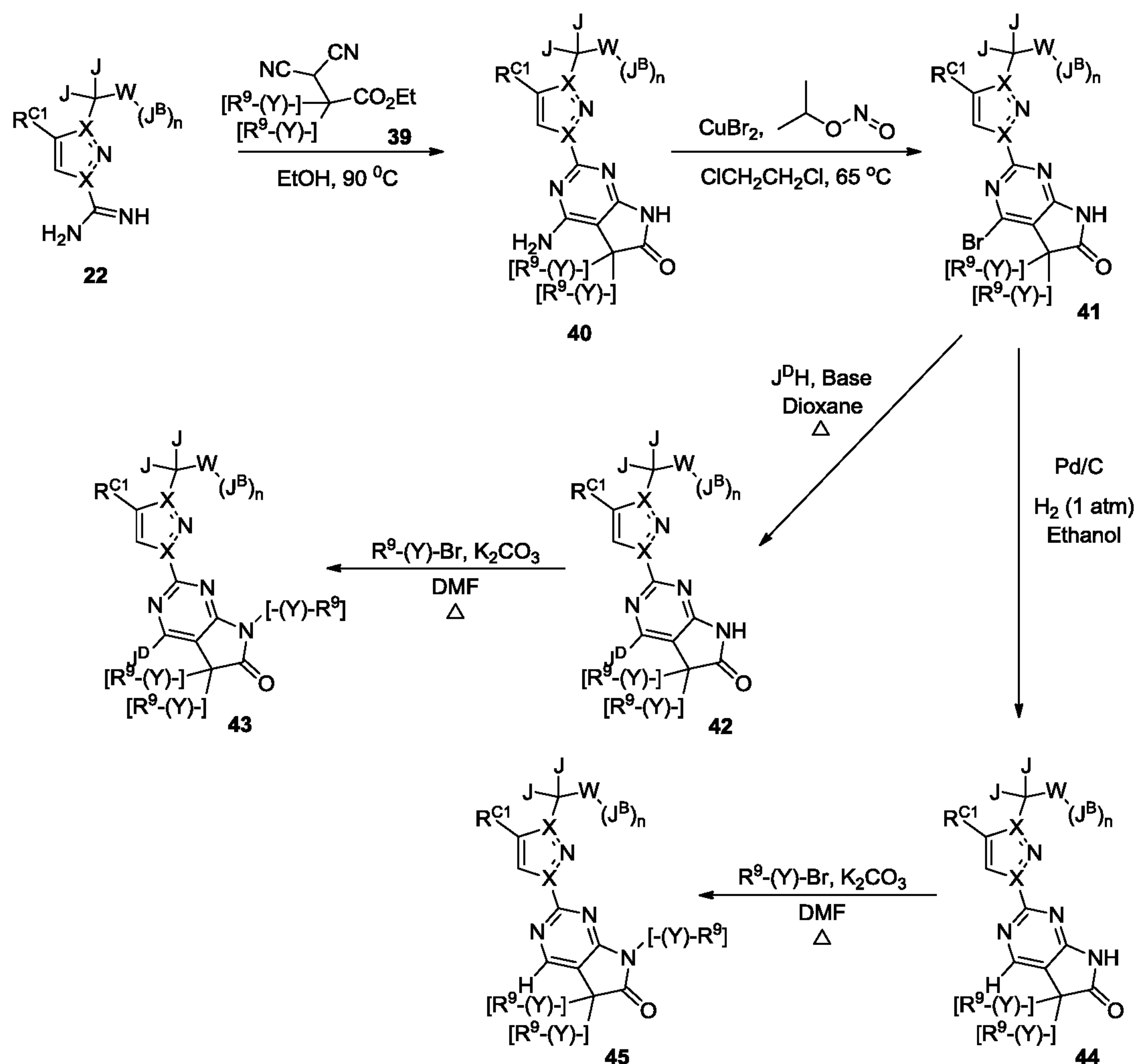
Scheme 7
