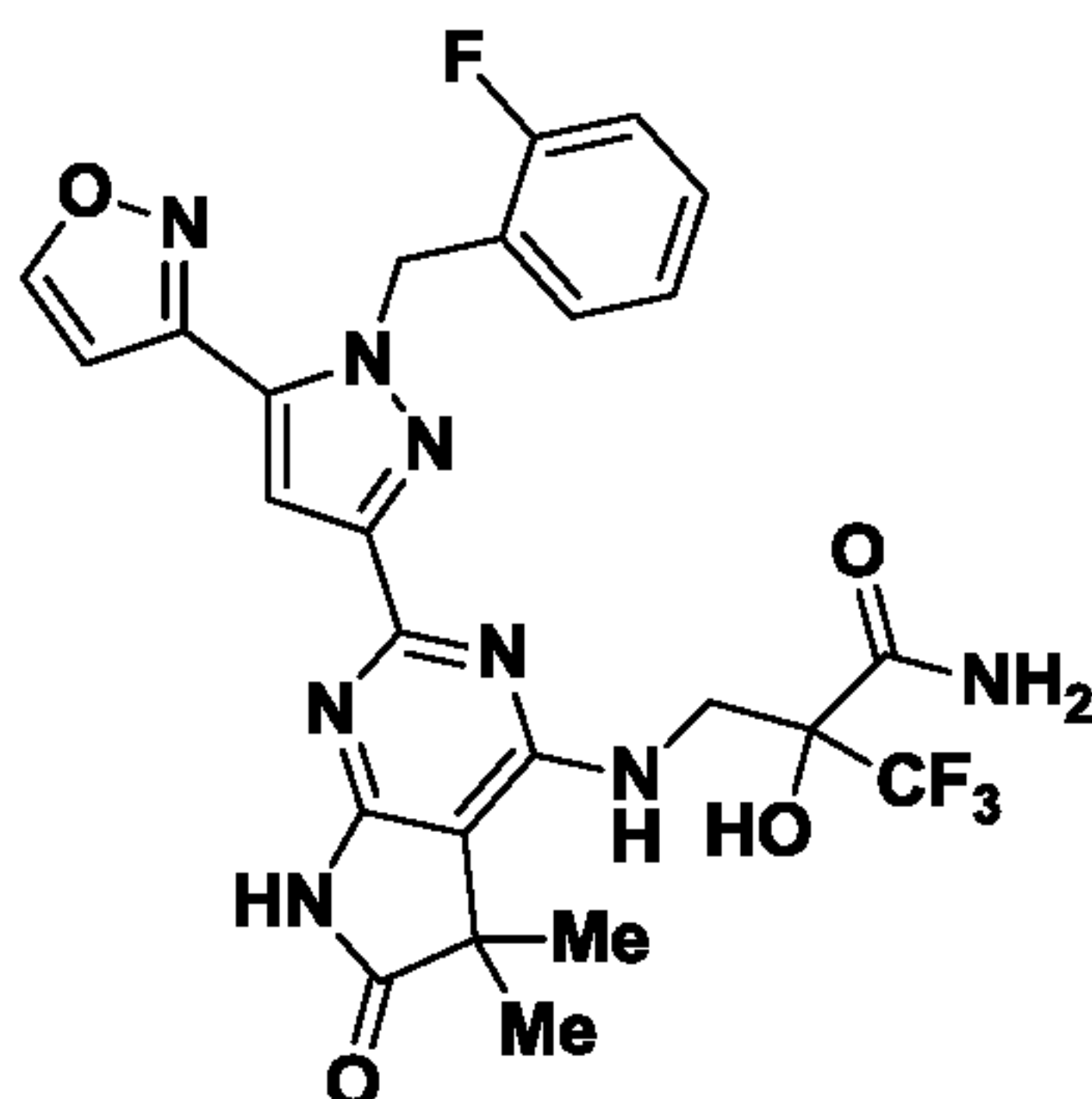
Compound I-8
