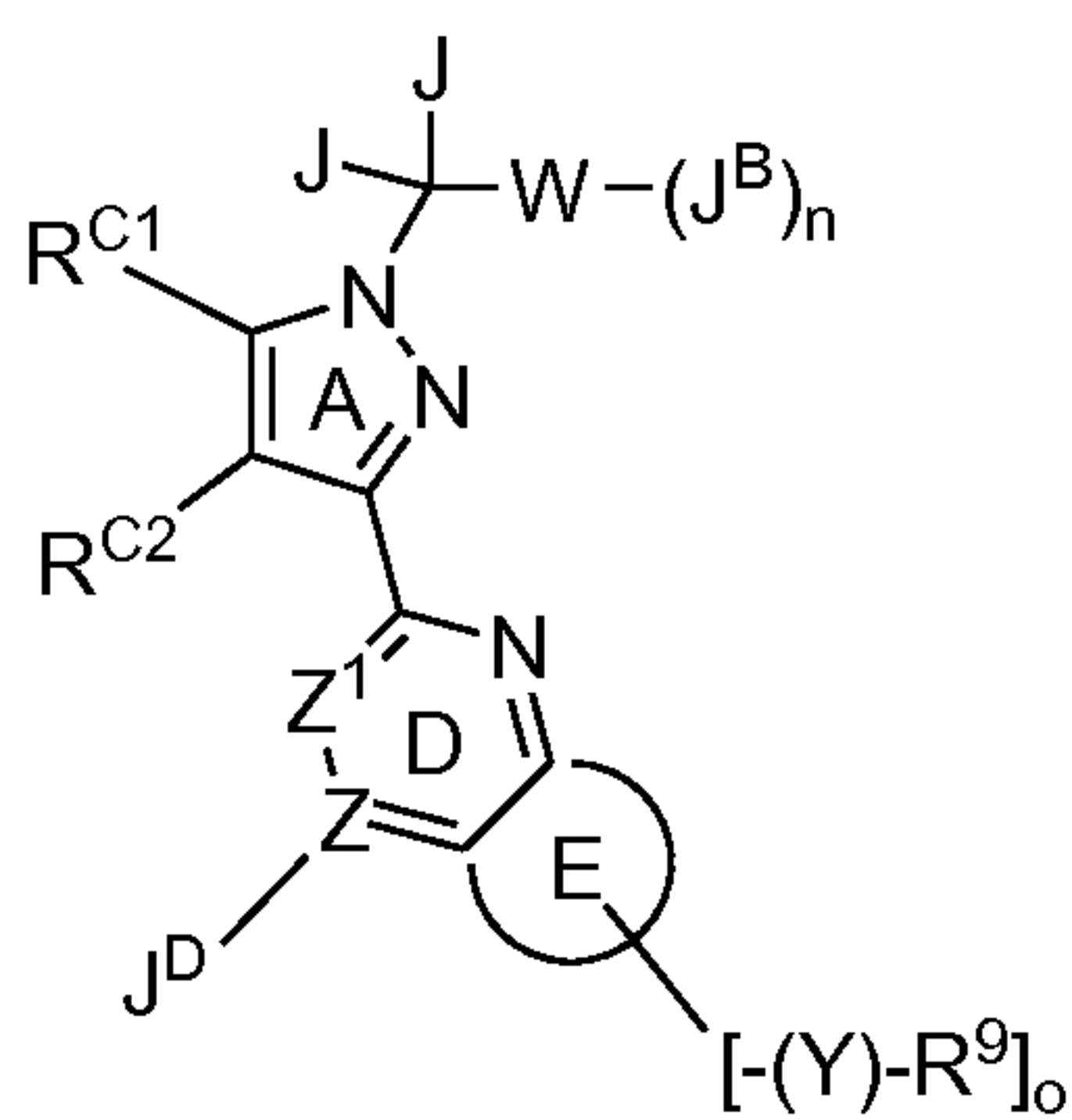
Formula IIA
