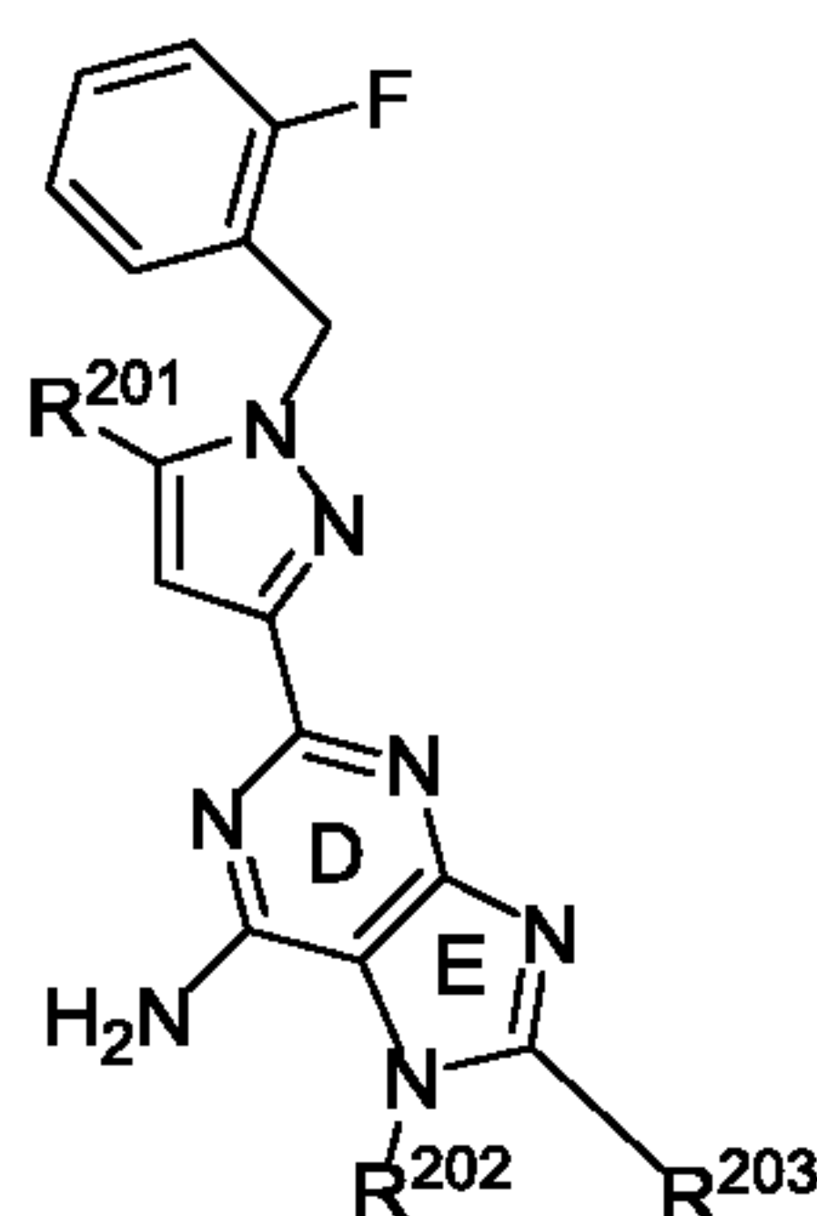
Formula B-1;
