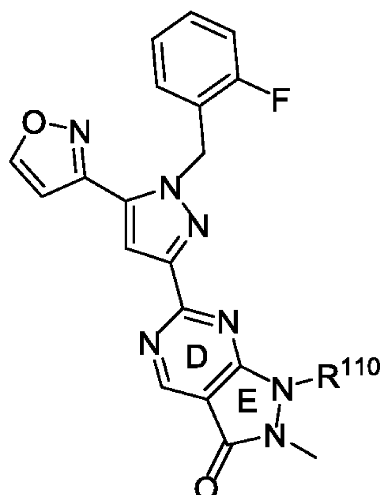
Formula B-4;
