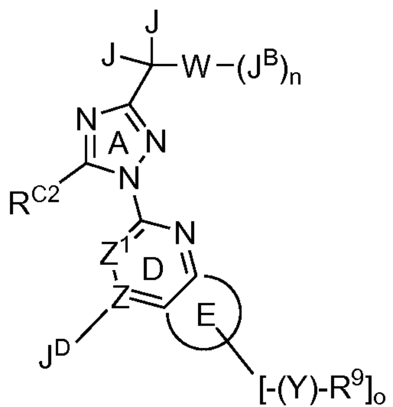
Formula IID
