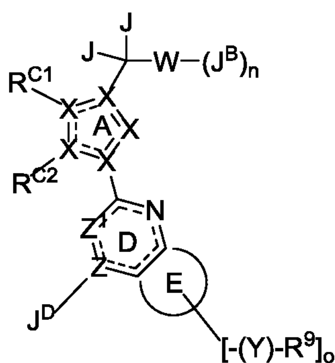
Formula I'
