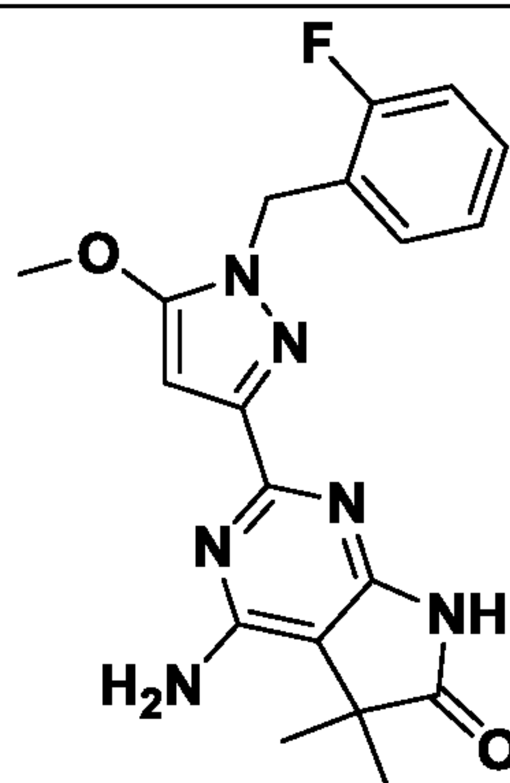
I-23
