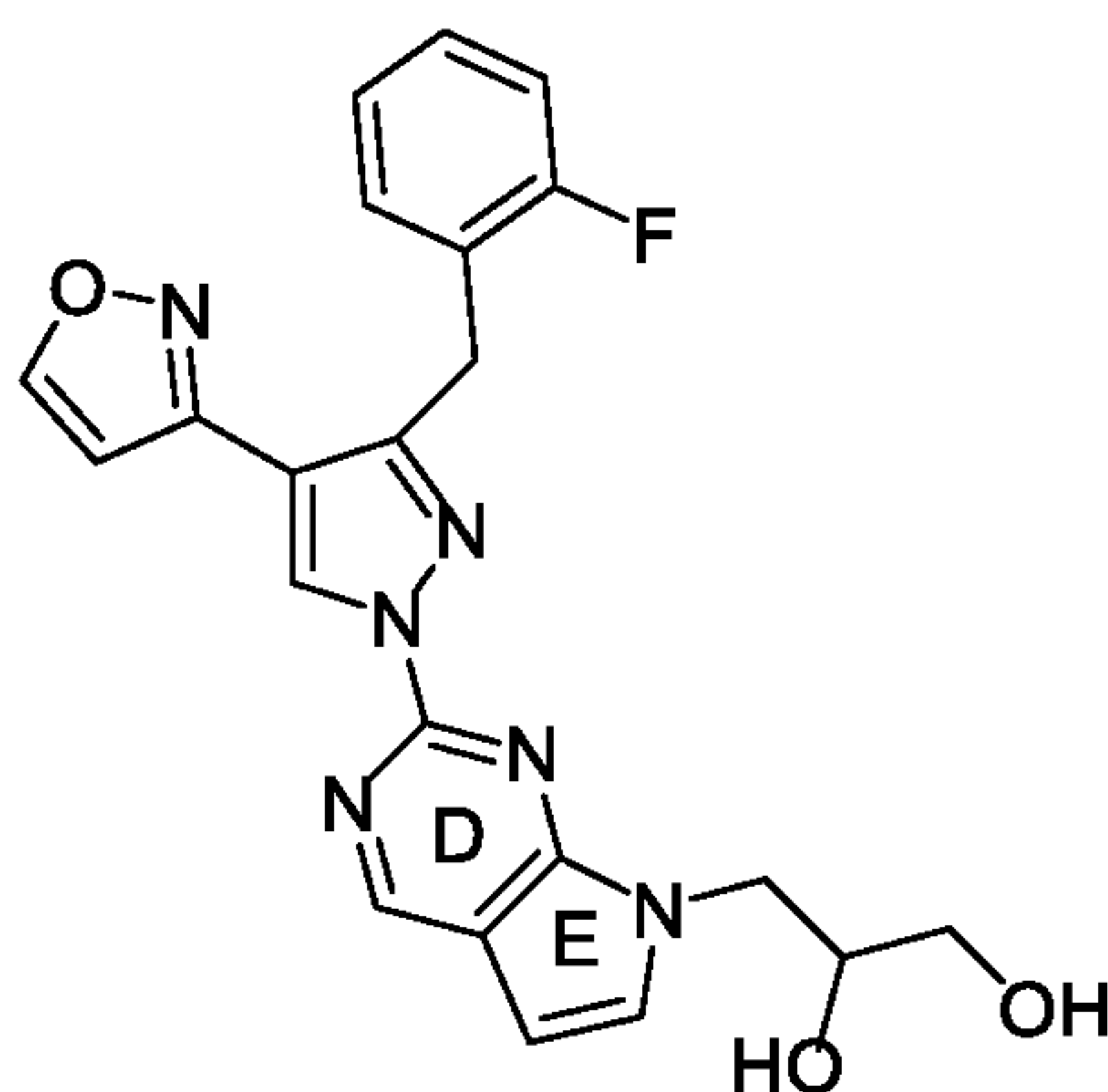
Formula B-5;
