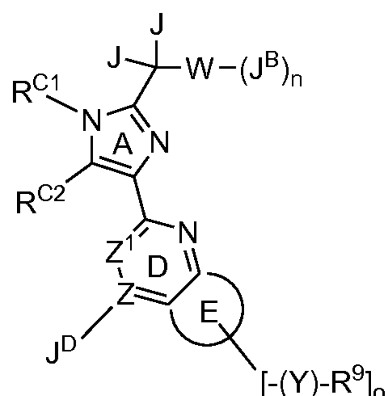
Formula IIE
