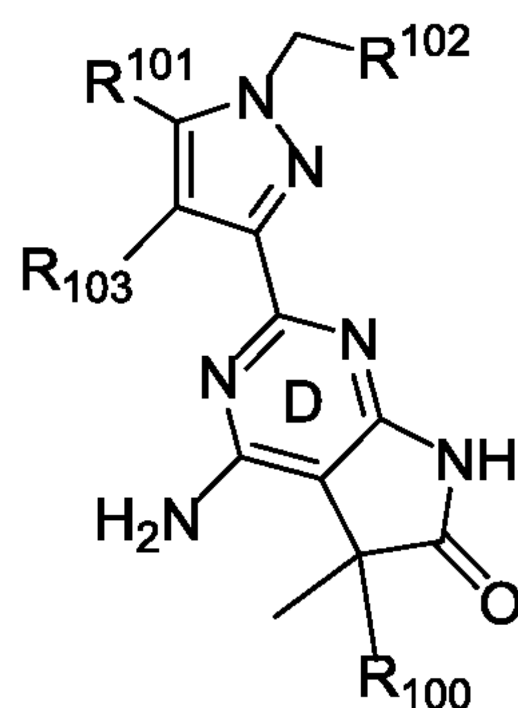
Formula A-1;
