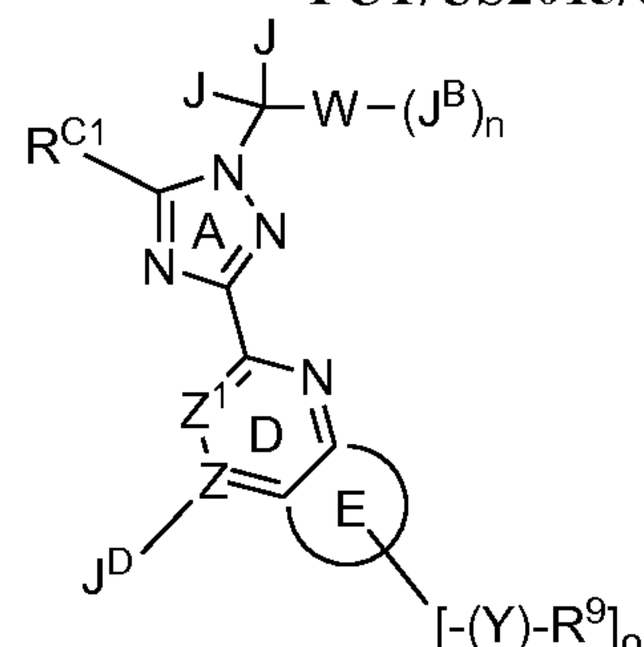
Formula IIC
