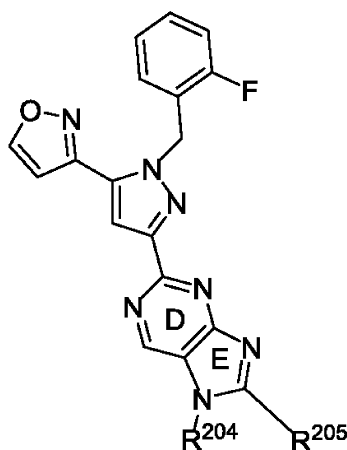
Formula B-2;
