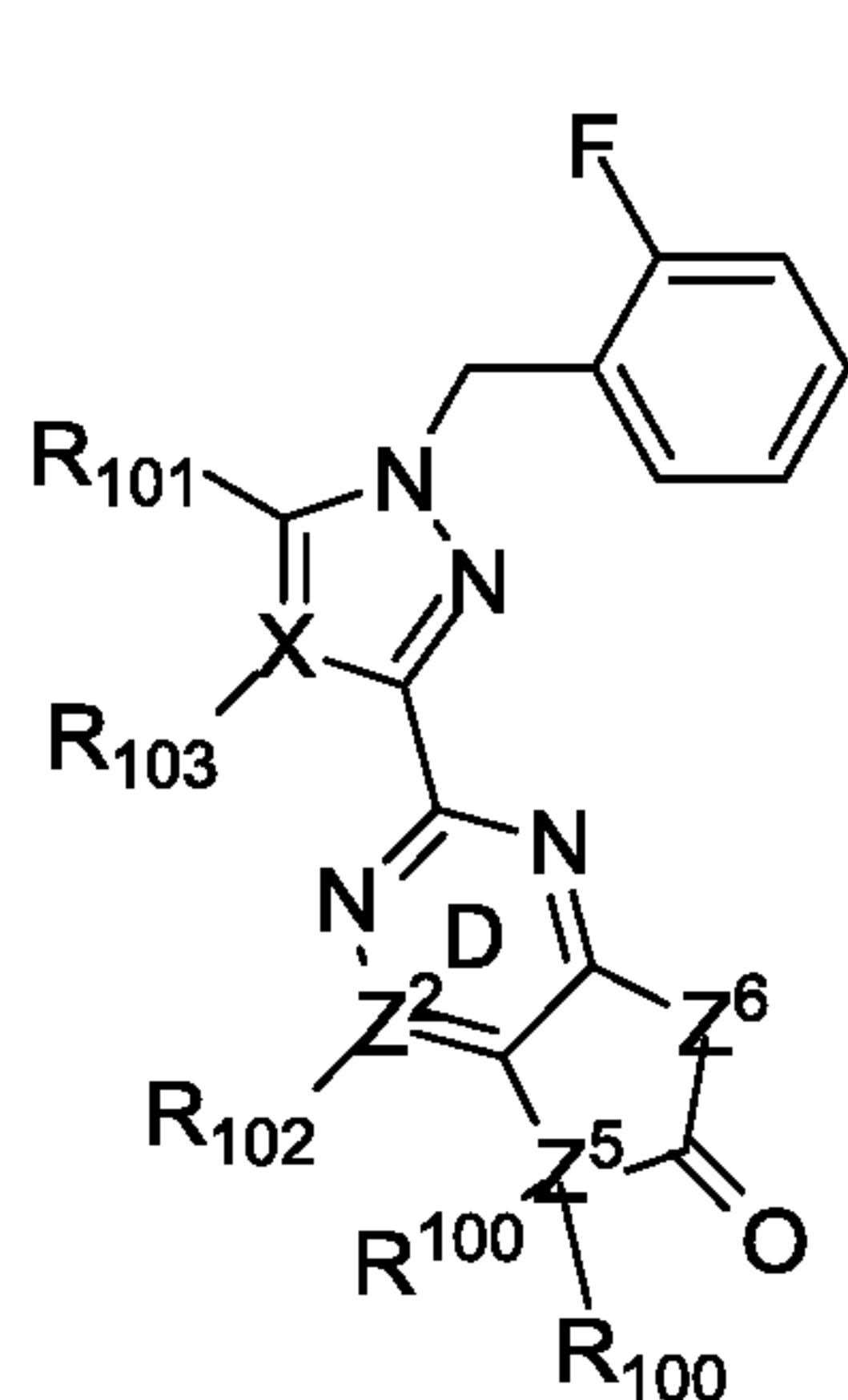
Formula C-1
