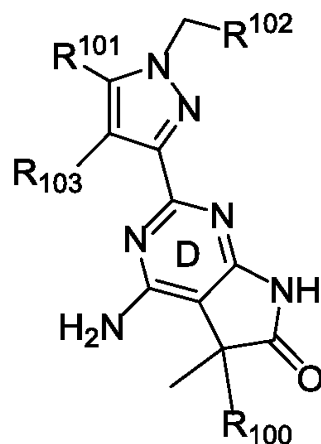
Formula A-1;
