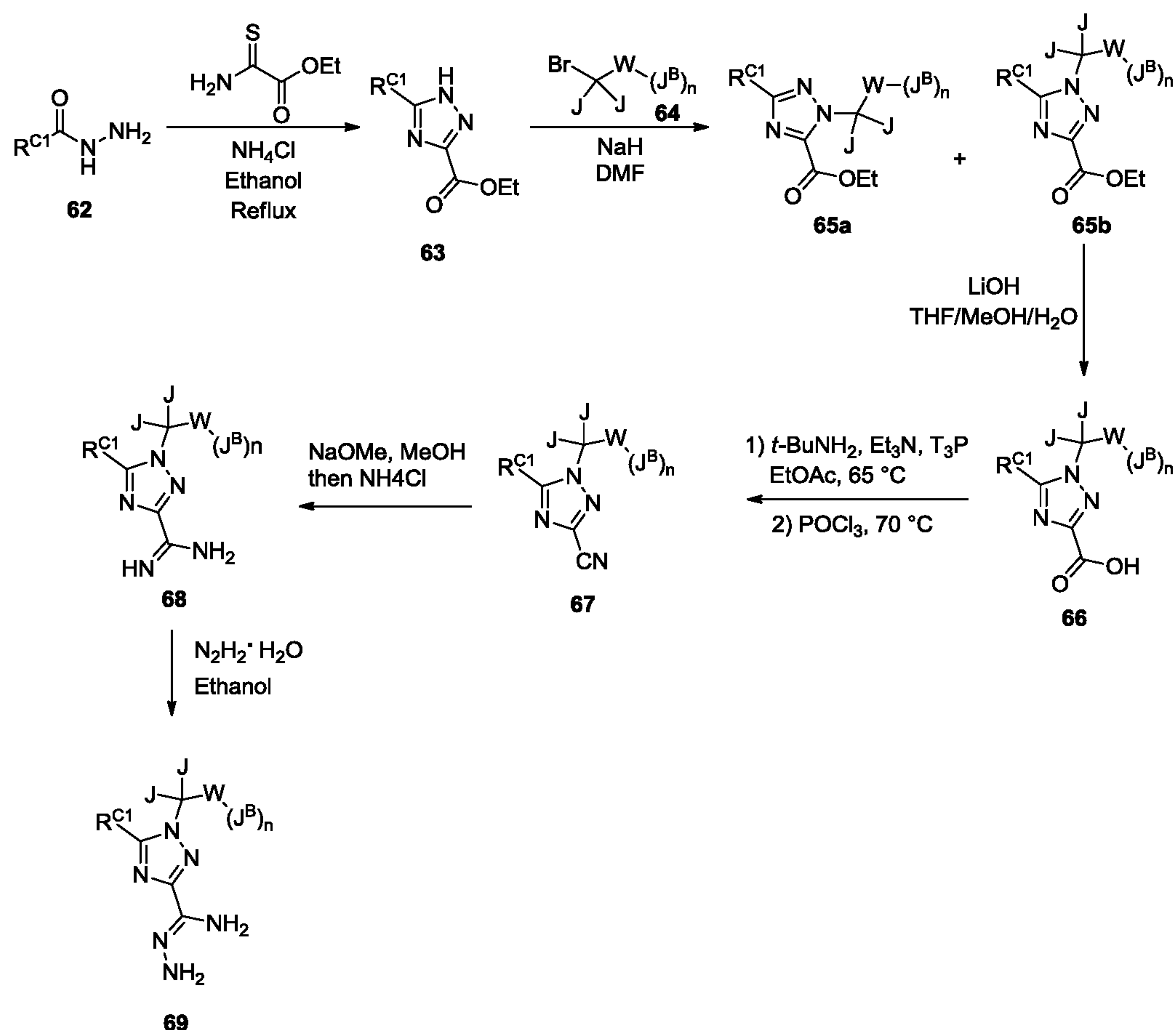
Scheme 12
