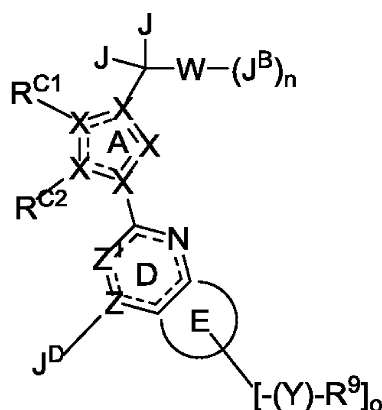
Formula I'
