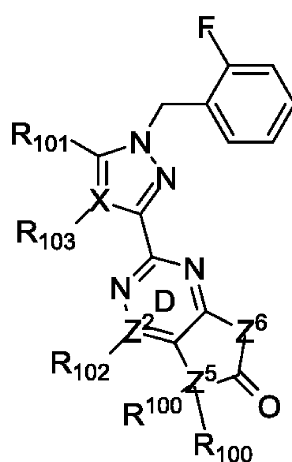
Formula C-1
