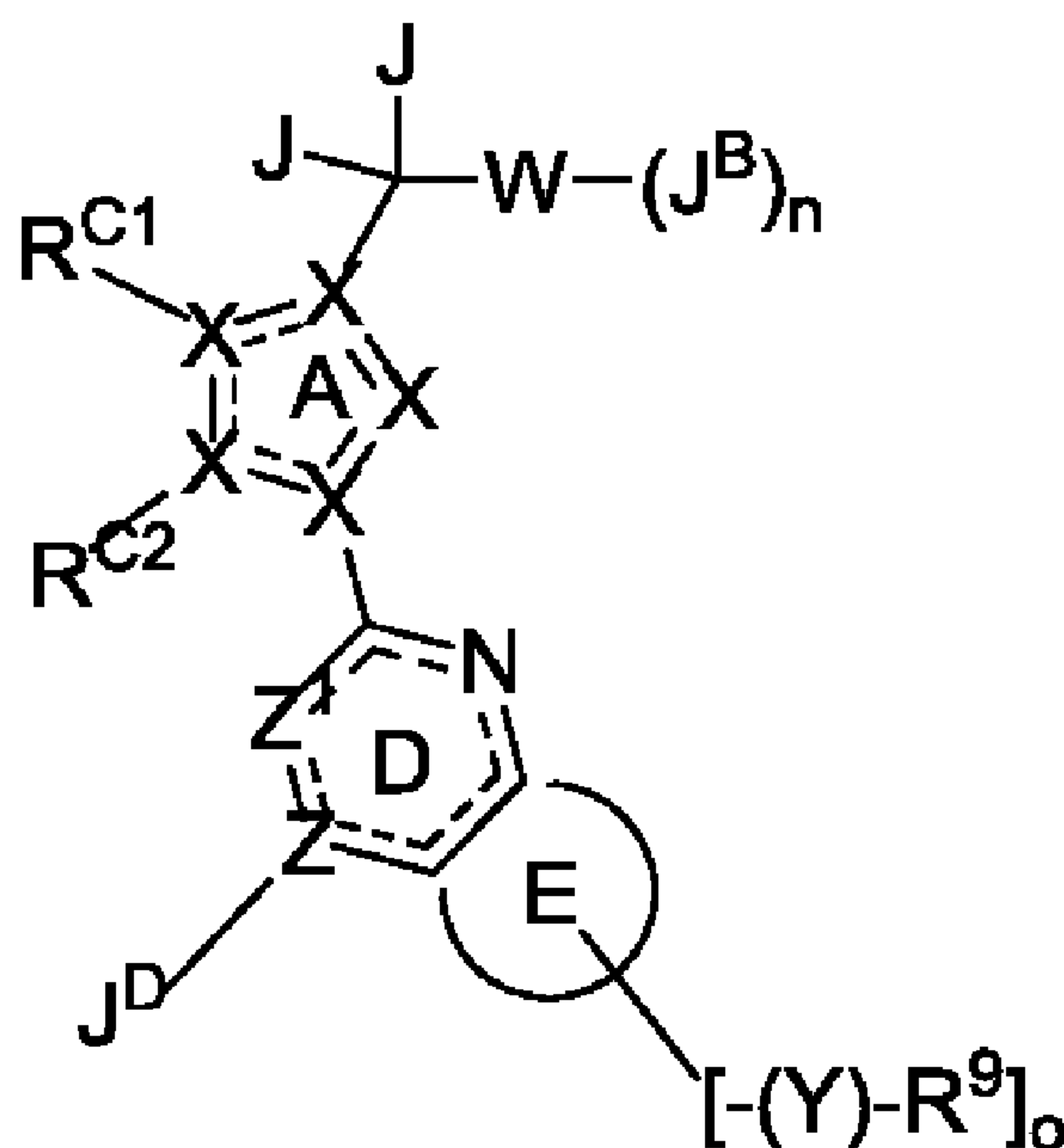
Formula I'
