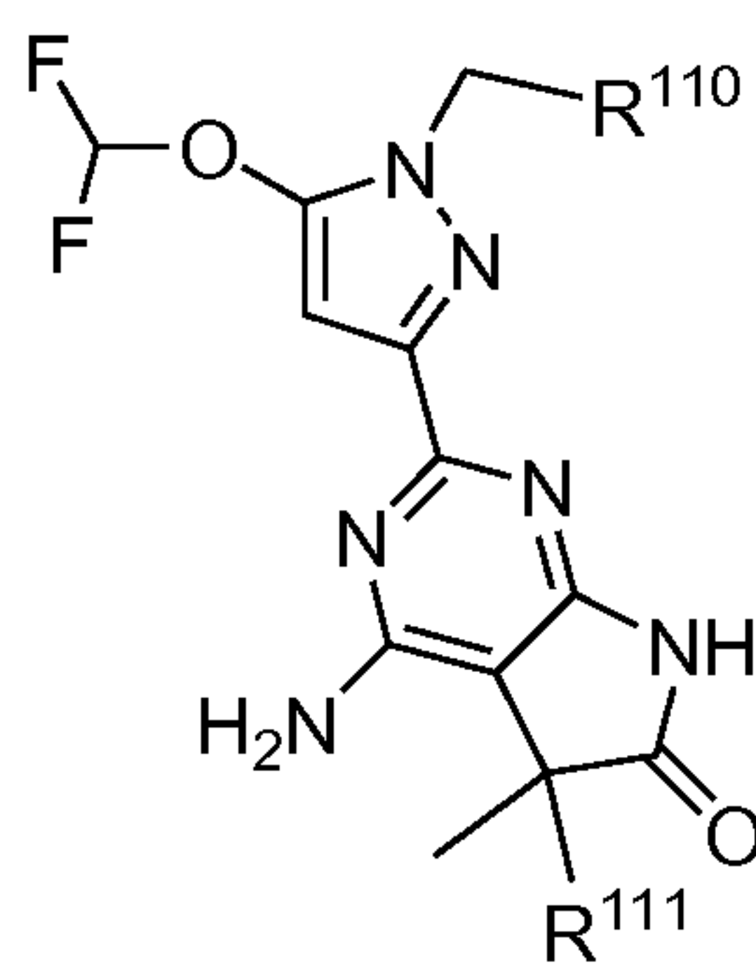
Formula A-7;
