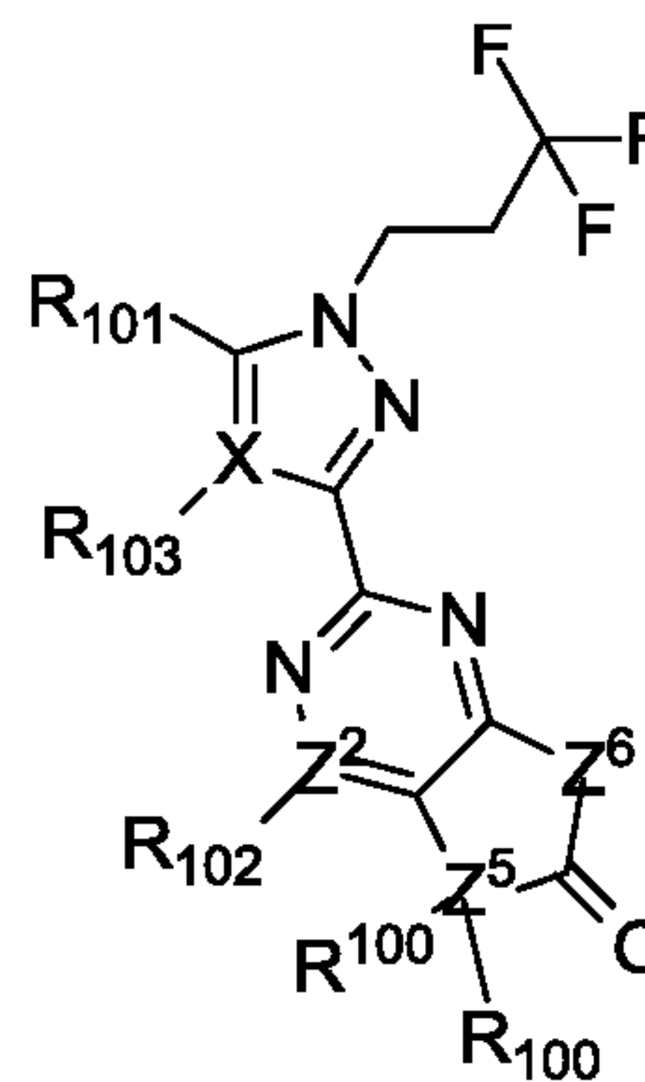
Formula C-2;
