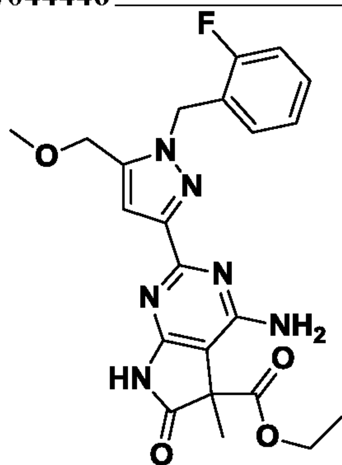
I-21
