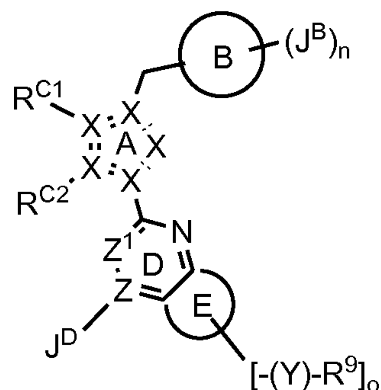
Formula I-c
