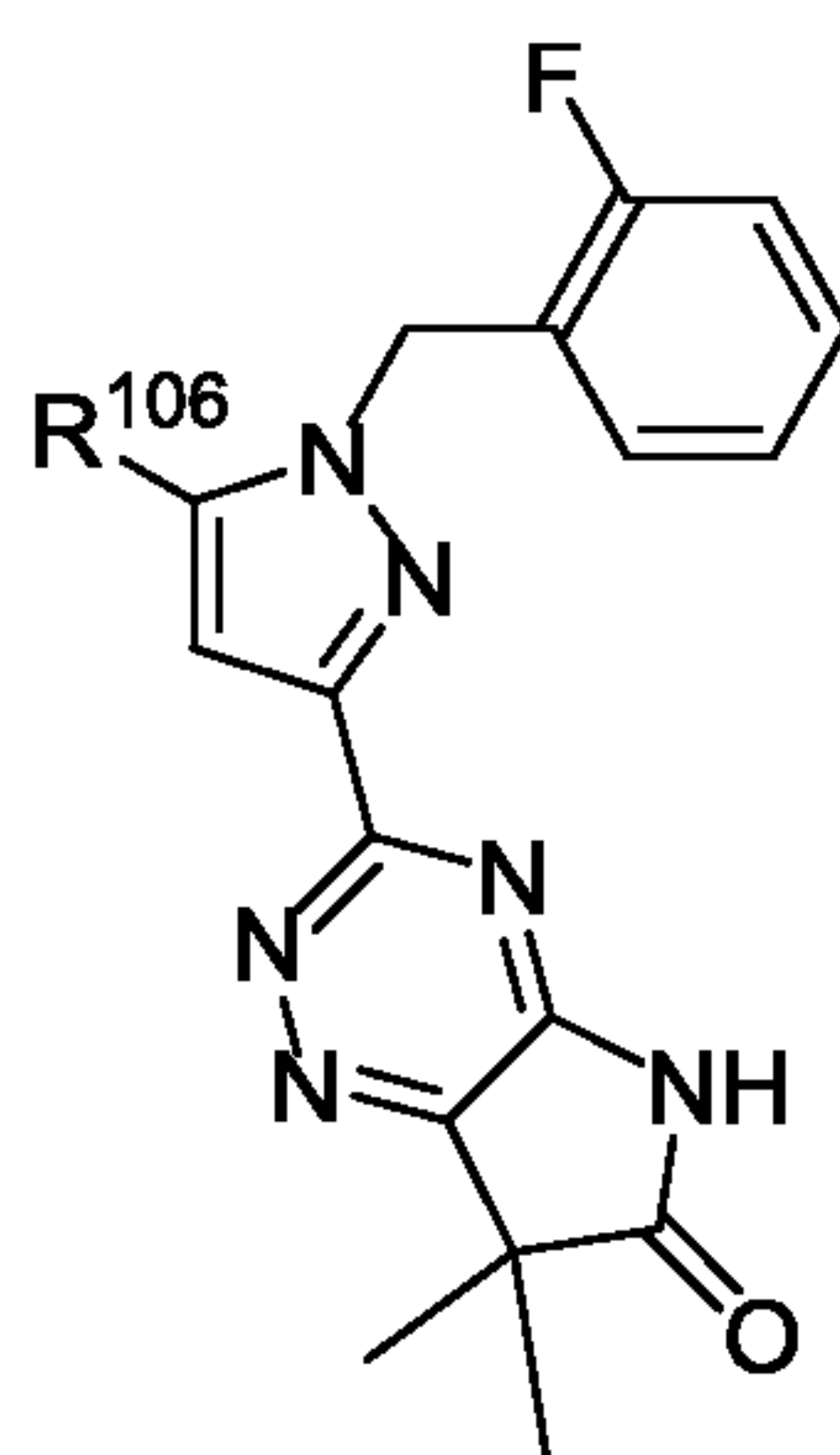
Formula A-3;
