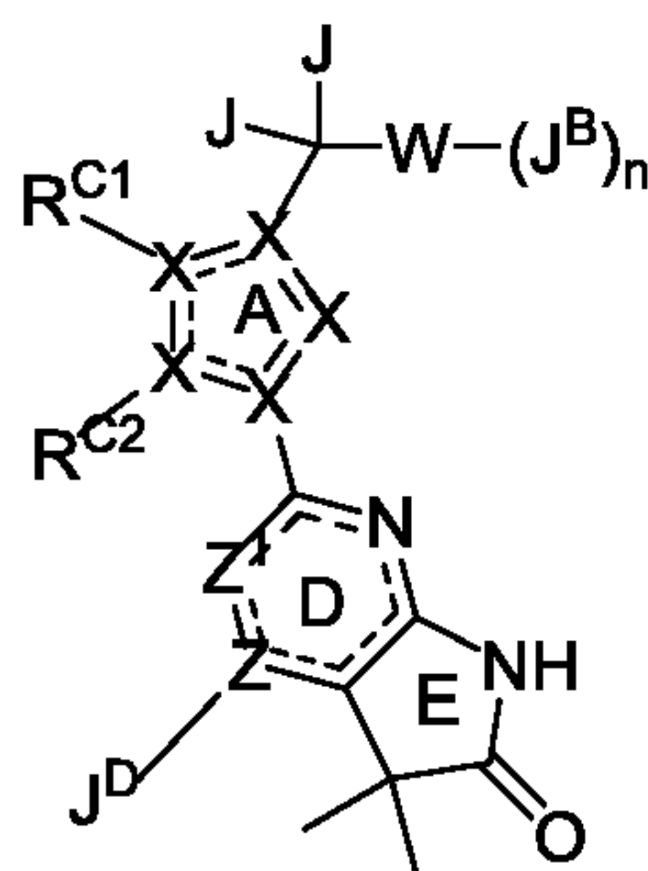
Formula I'D
