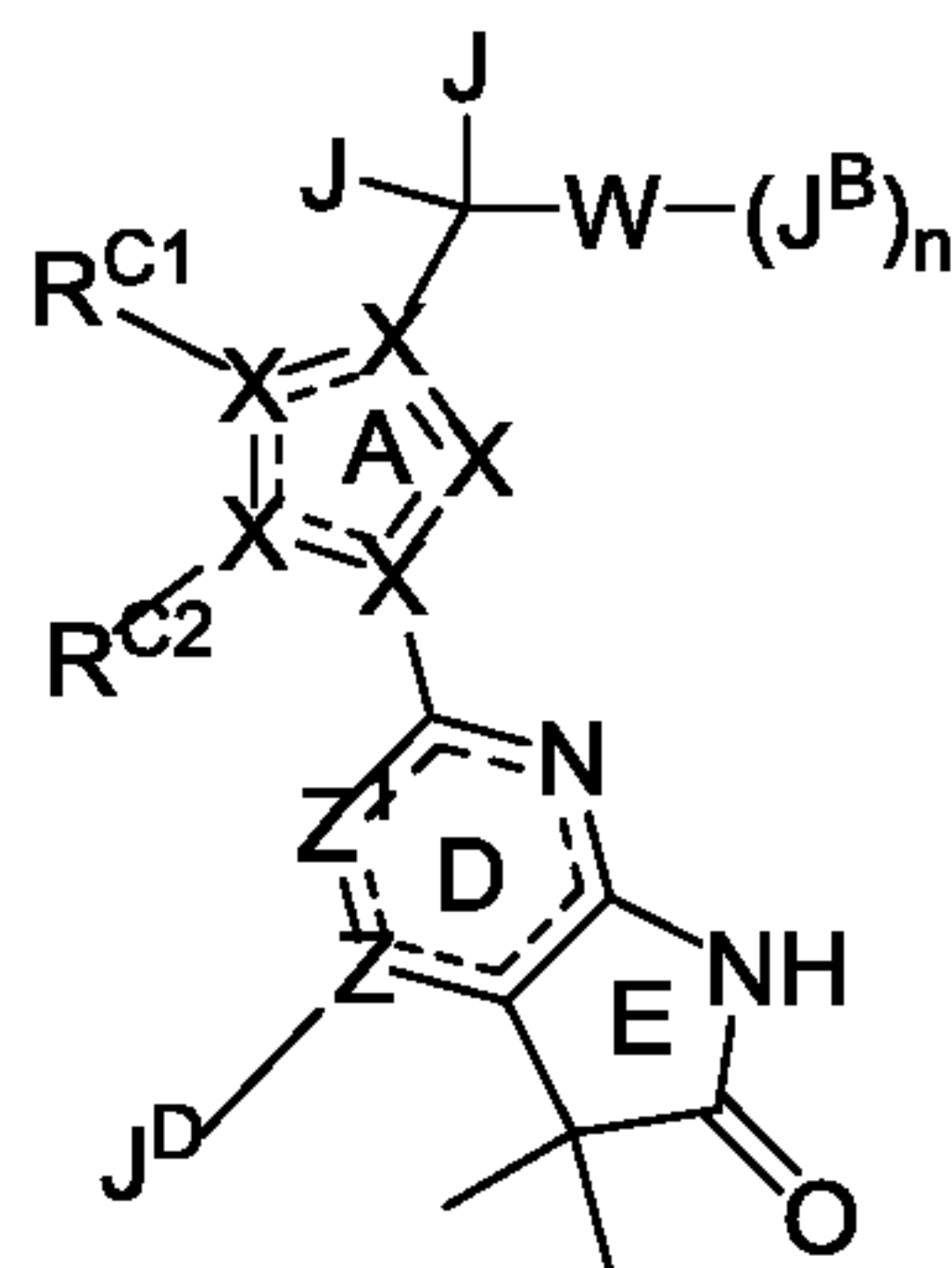
Formula I'D
