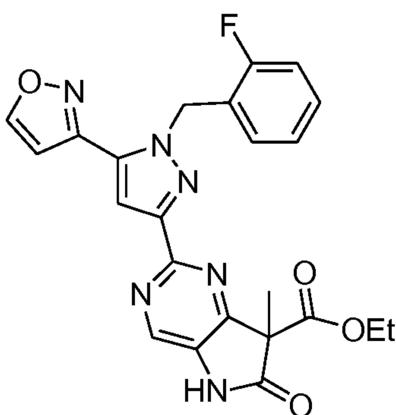
Formula A-5;
