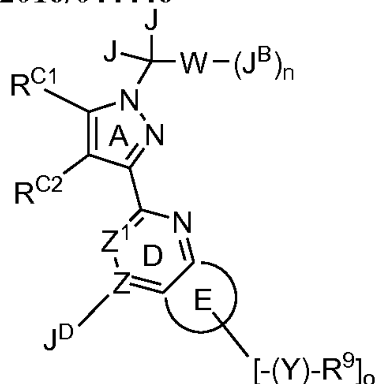
Formula IIA
