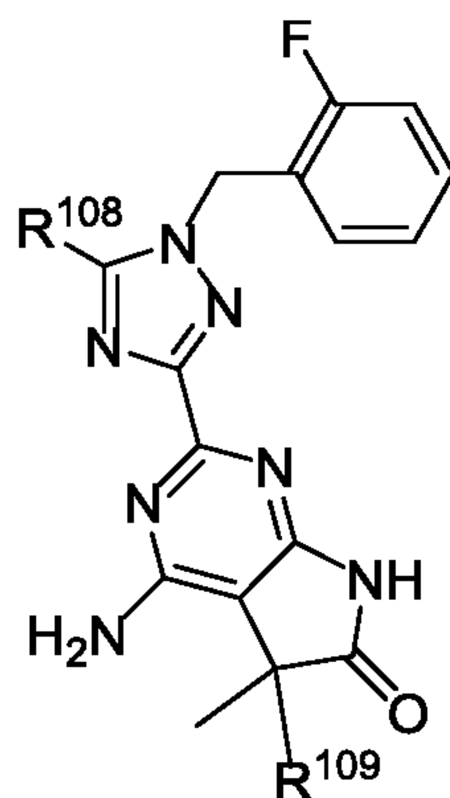
Formula A-6;
