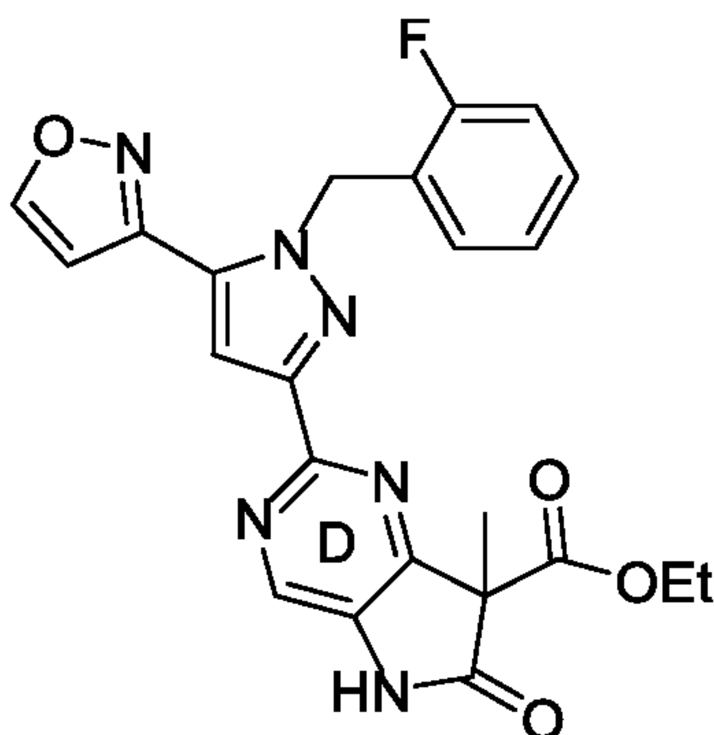
Formula A-5;
