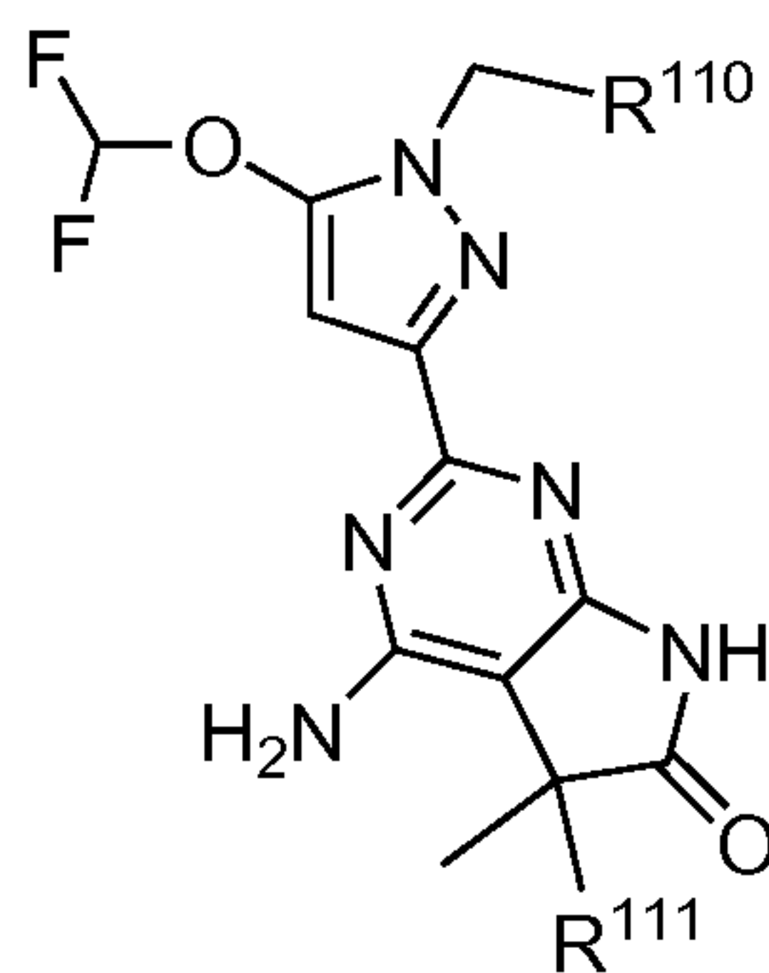
Formula A-7;
