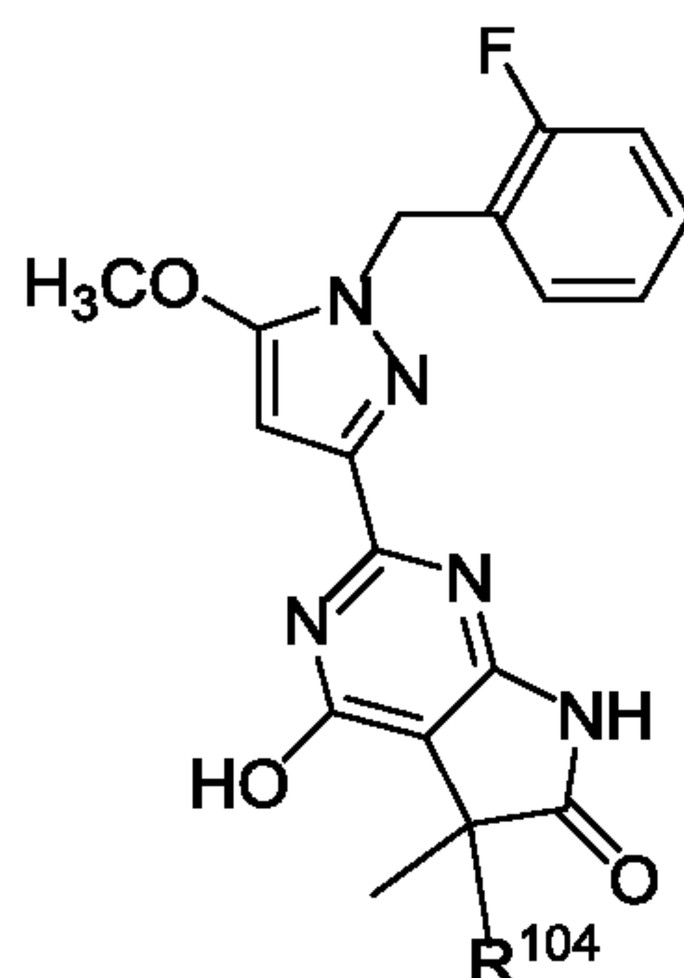
Formula A-2;
