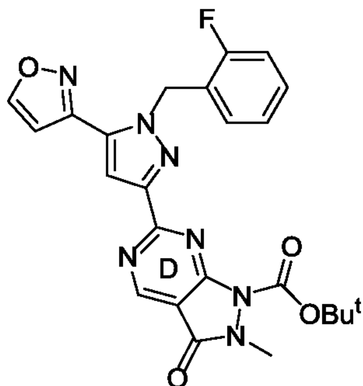
Formula A-8;
