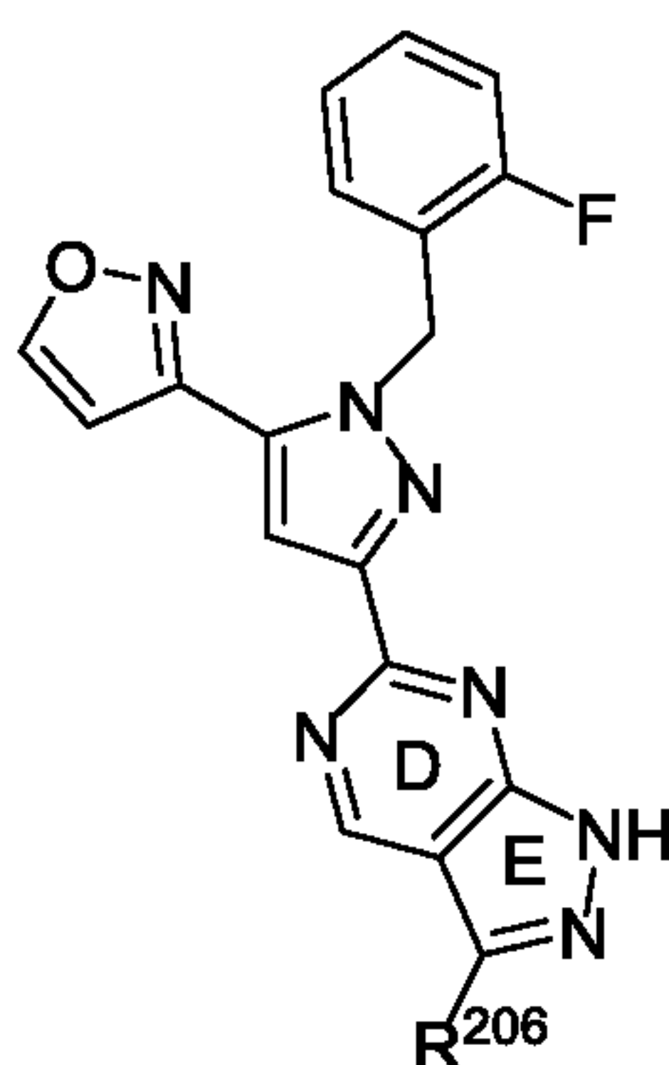
Formula B-3;
