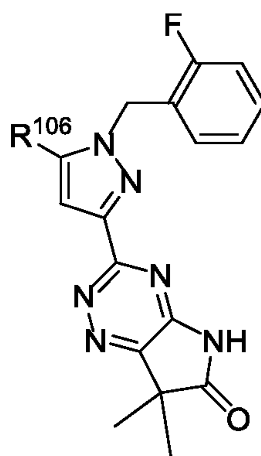
Formula A-3;
