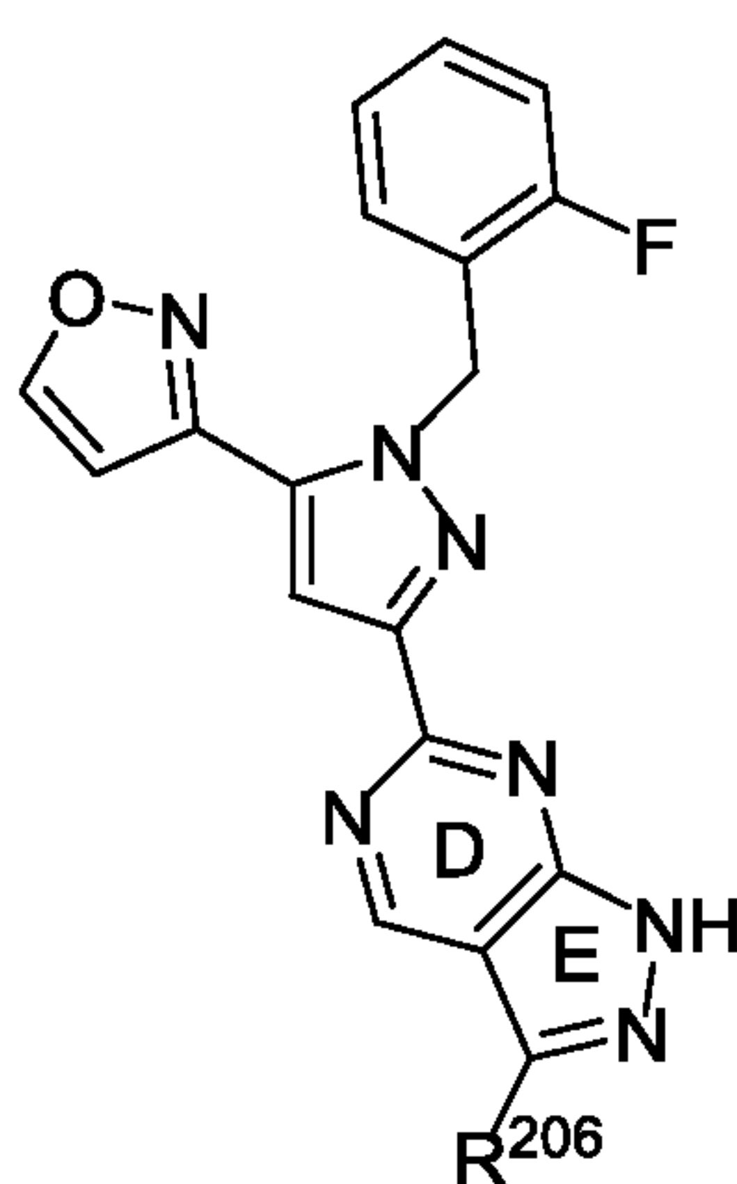
Formula B-3;
