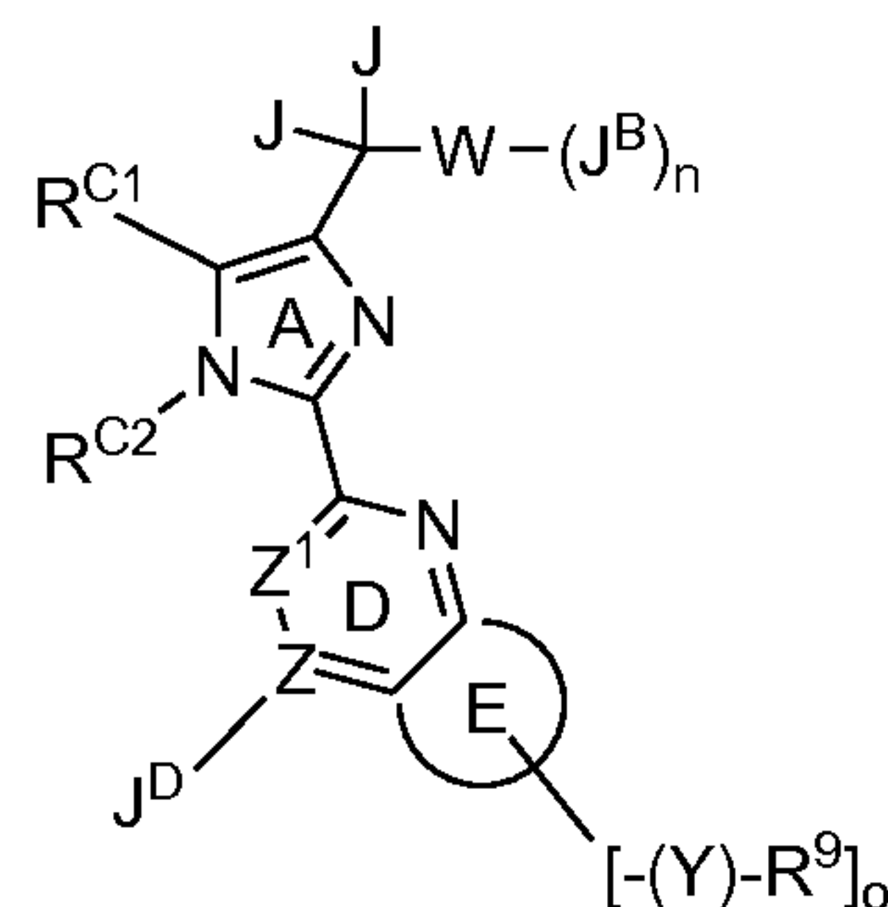
Formula IIF
