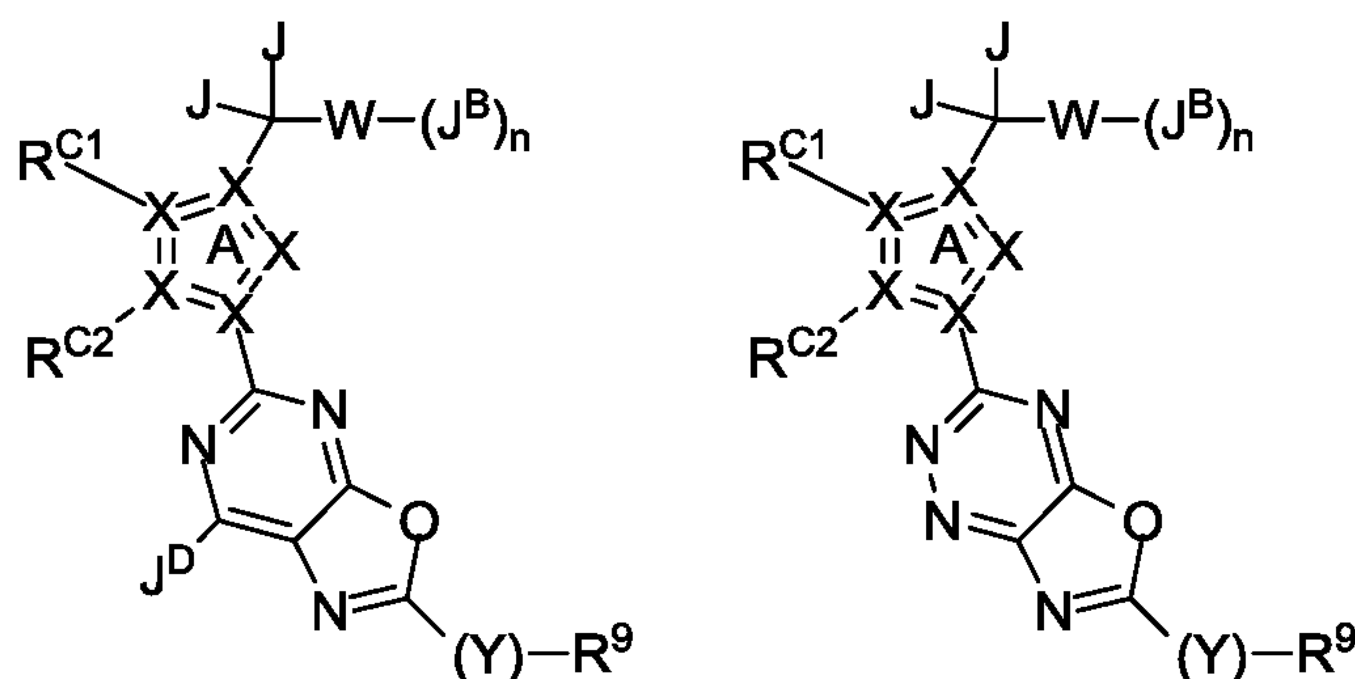
Formula I-p
