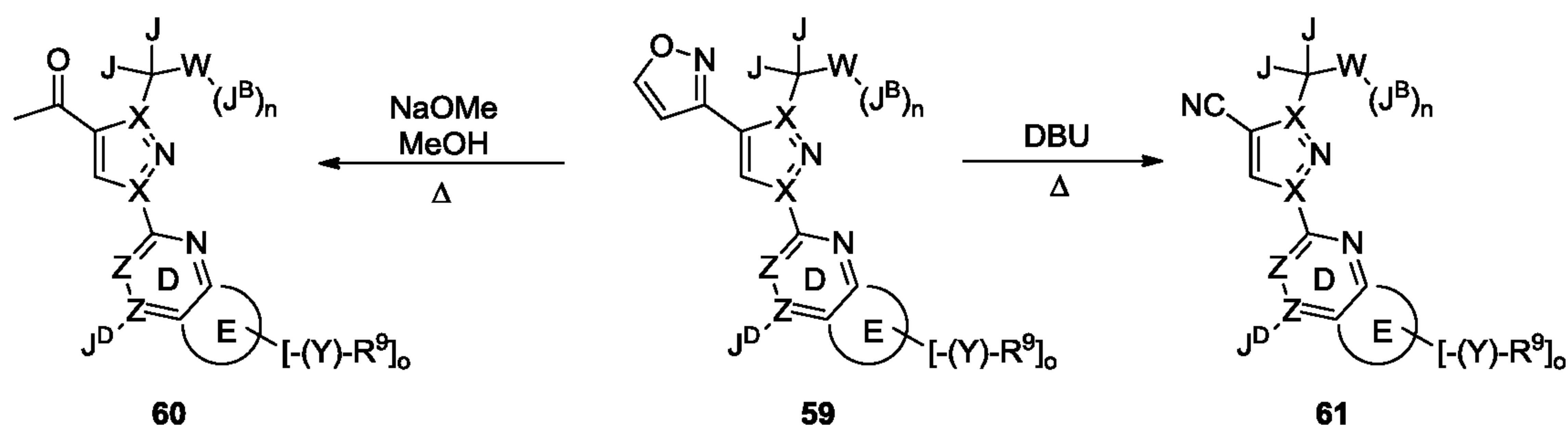
Scheme 11
