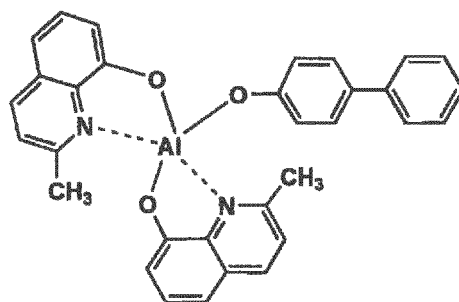
BAIq
