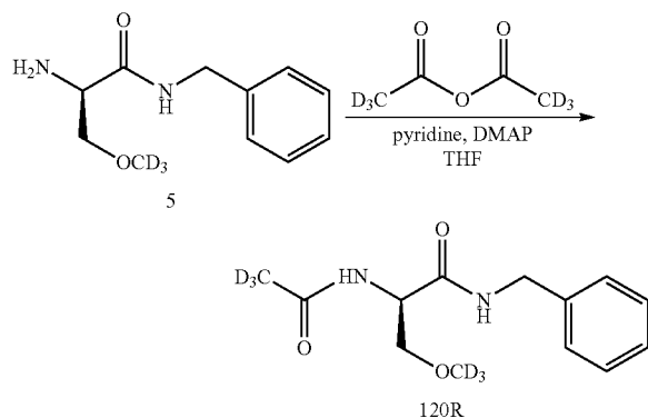
Scheme 3: Preparation of Compound 120:
