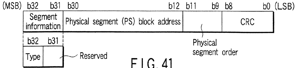
Layout of address field in WAP
