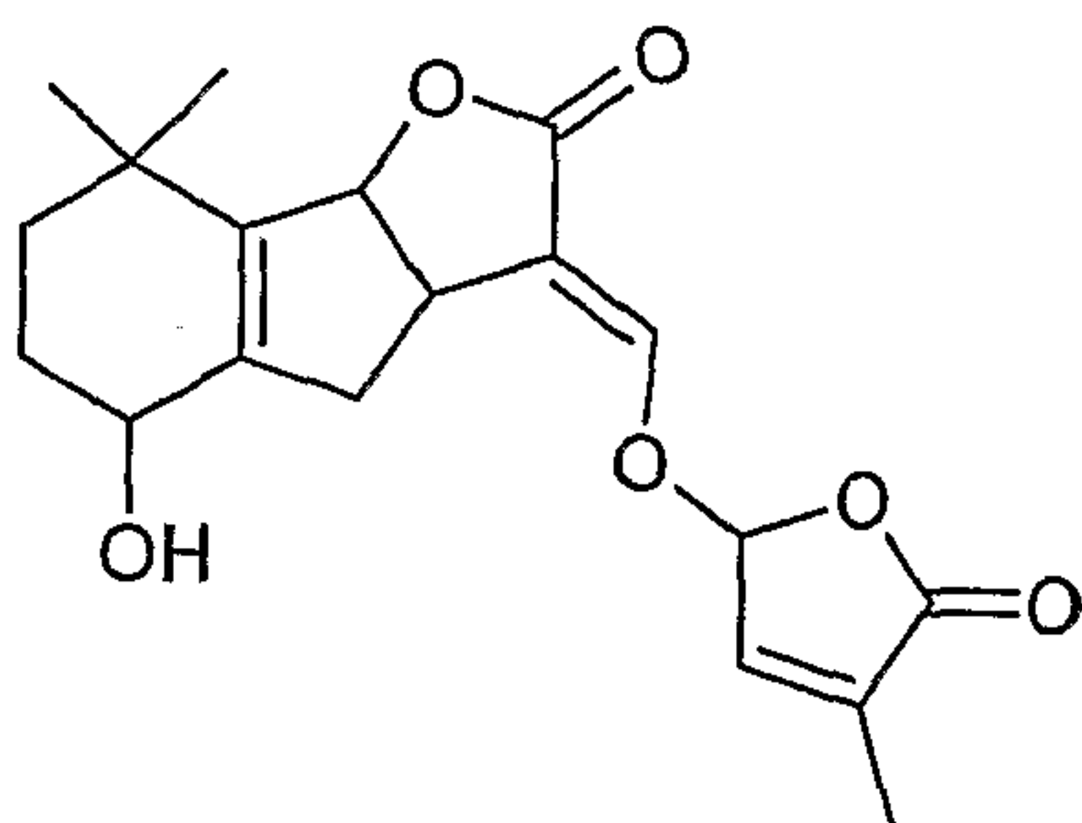
Strigol (Cook et al., Science, 1966, 1954:1189-1190 ;)
