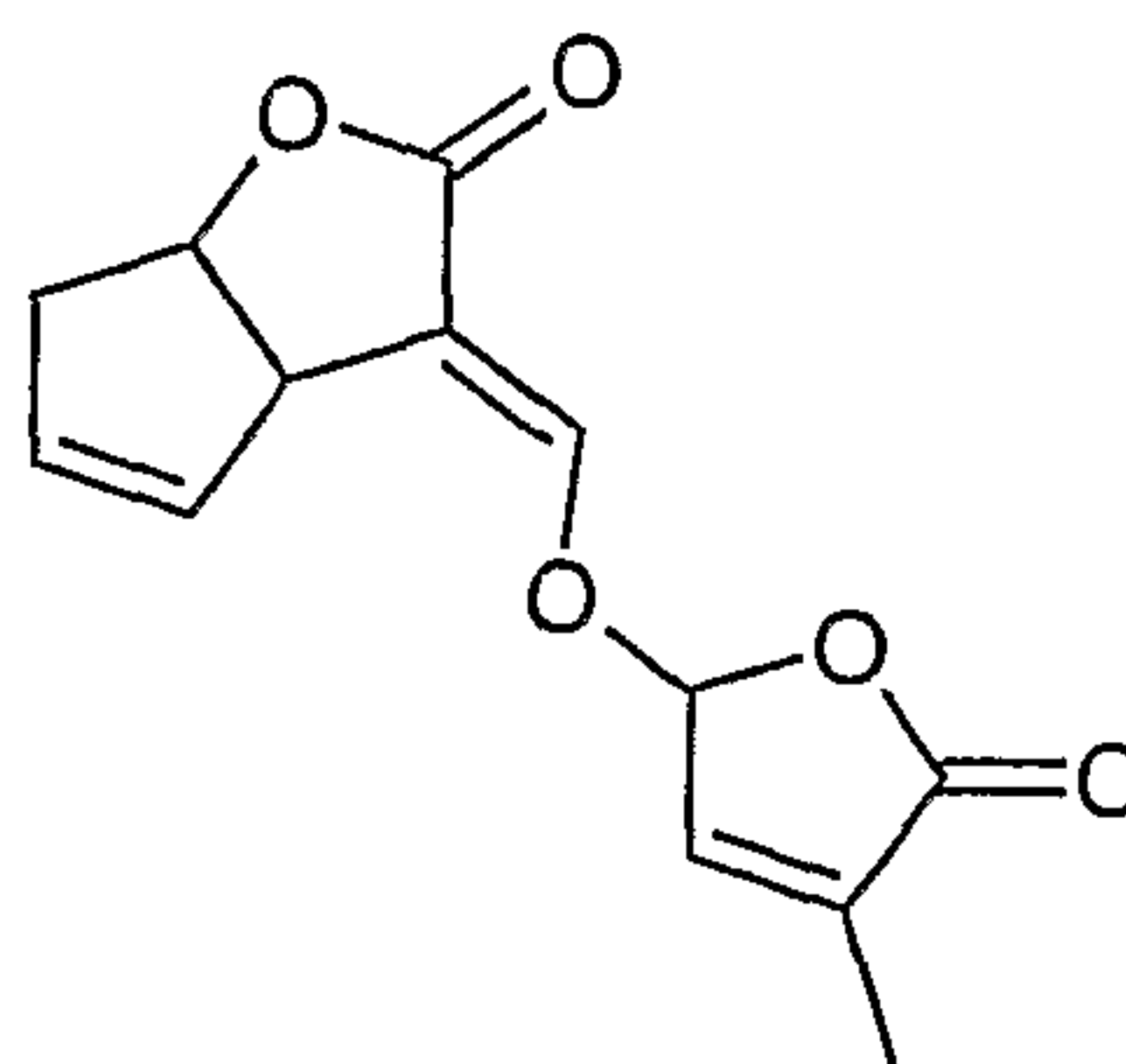
GR7 (Johnson et al. , Weed Res., 1976, 16:223-227)
