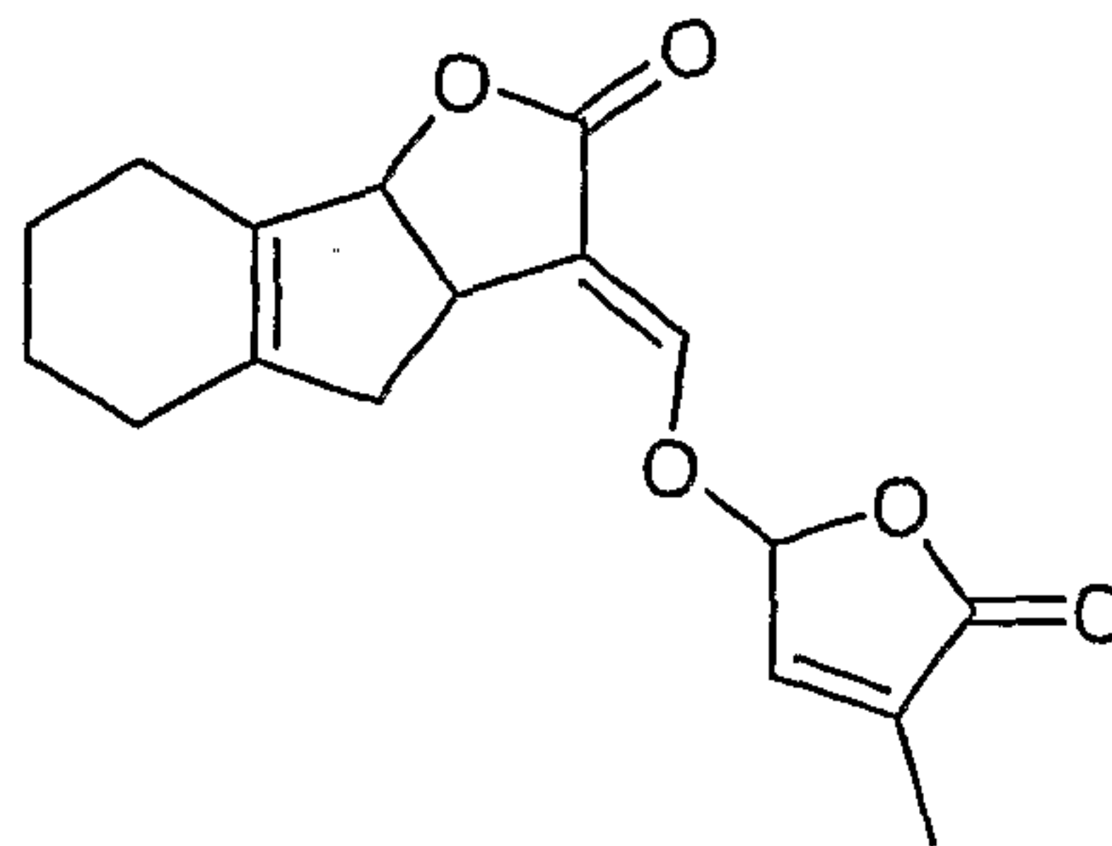
Déméthylsorgolactone (Thuring et al., J. Agric. Food Chem., 1997, 45(6):2278- 2283)
