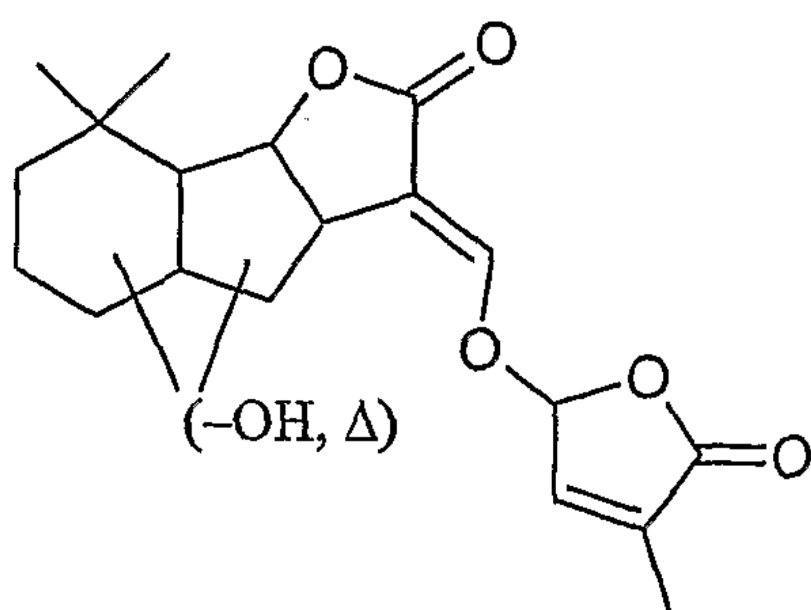
Orobanchol (Yokota et al., Phytochemistry, 1998, 49(7):1967-1973)
