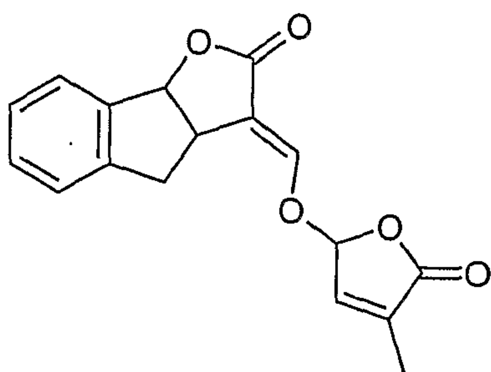
25 GR24 (Mangnus et al. , J. Agric. Food Chem., 1992, 40(6):697-700)
