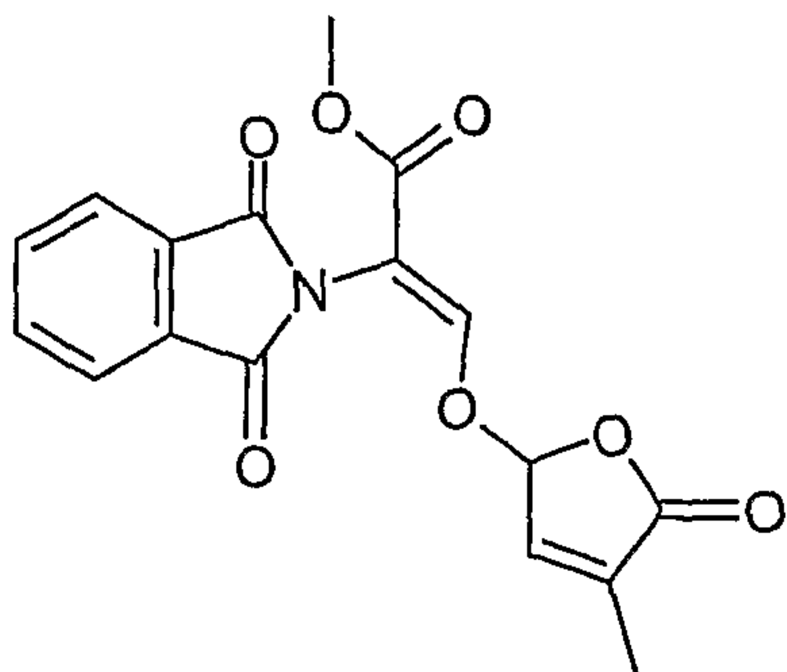
Nijmegen 1 (Nefkens et al., J. Agric. Food Chem., 1997, 45(6):2273-2277)
