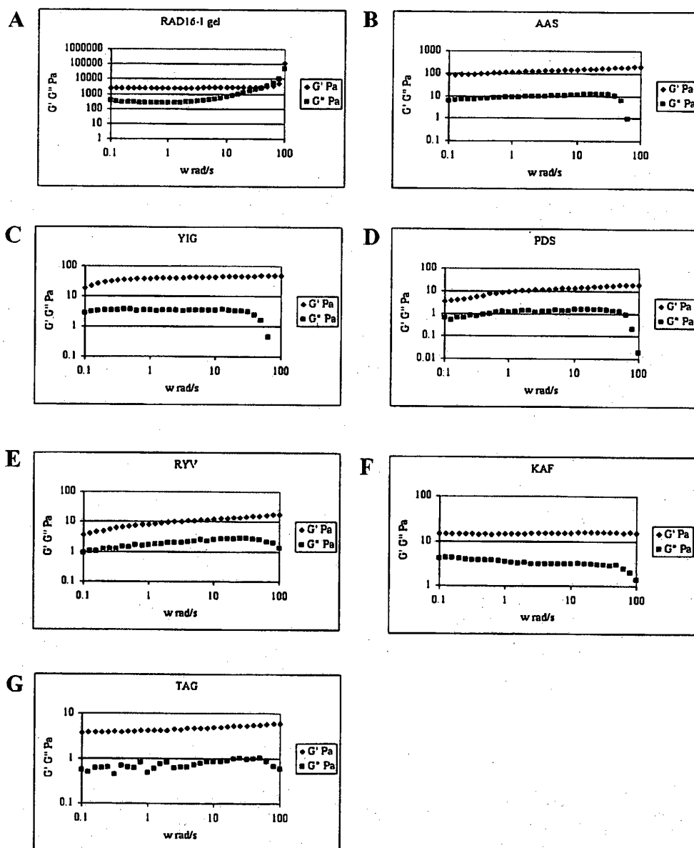
Figure 6. Dynamic frequency sweep test for peptide scaffolds at a fixed strain=0.01. A) RAD16-I, B) AAS, C) YIG, D) PDS, E) RYV, F) KAF, G) TAG. G' (Storage modulus) represents the elastic character of the material, and G'' (Loss modulus) represents its viscous character.
