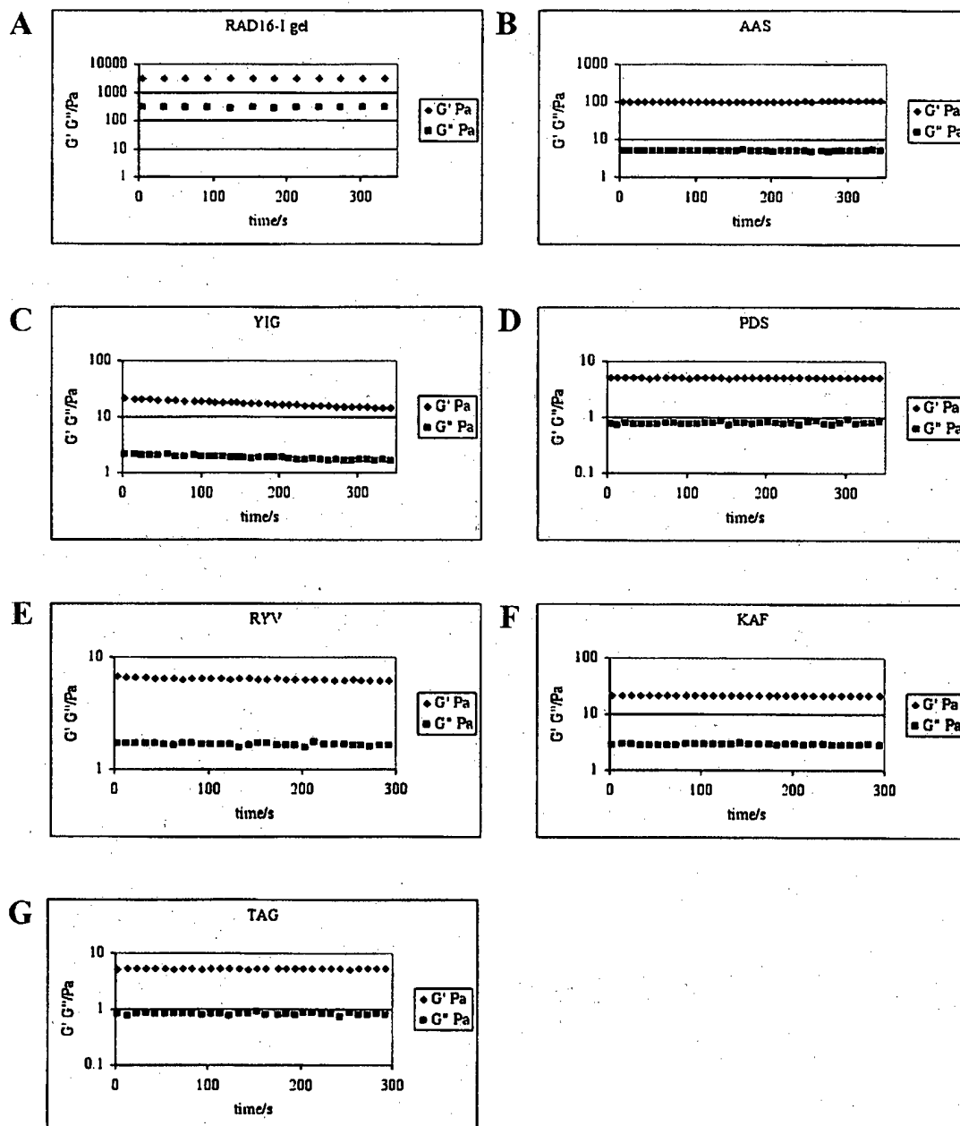
Figure 7. Dynamic time sweep test for peptide scaffolds at a fixed frequency=10 rad/s. A) RAD16-I, B) AAS, C) YIG, D) PDS, E) RYV, F) KAF, G) TAG.
